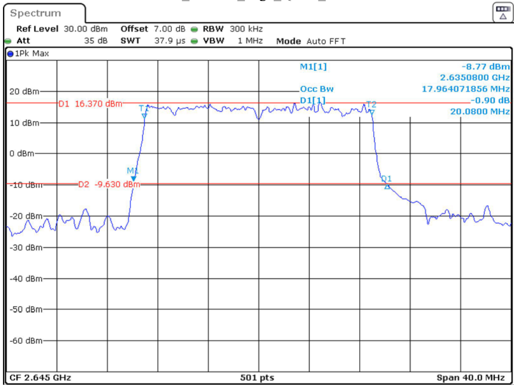
Band 41_20 MHz_High_QPSK_RB100#0
