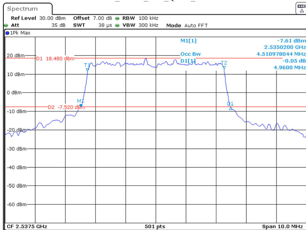
Band 41_5 MHz_Low_QPSK_RB25#0
