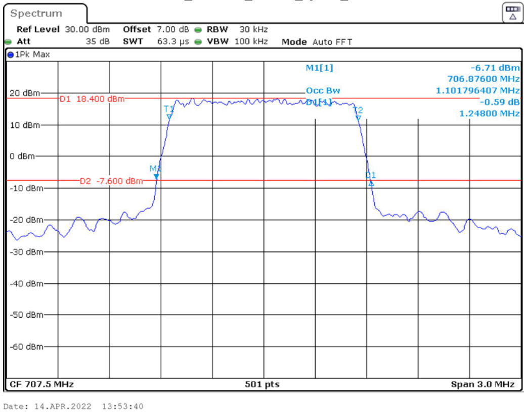
Band 12_1.4 MHz_Middle_QPSK_RB6#0
