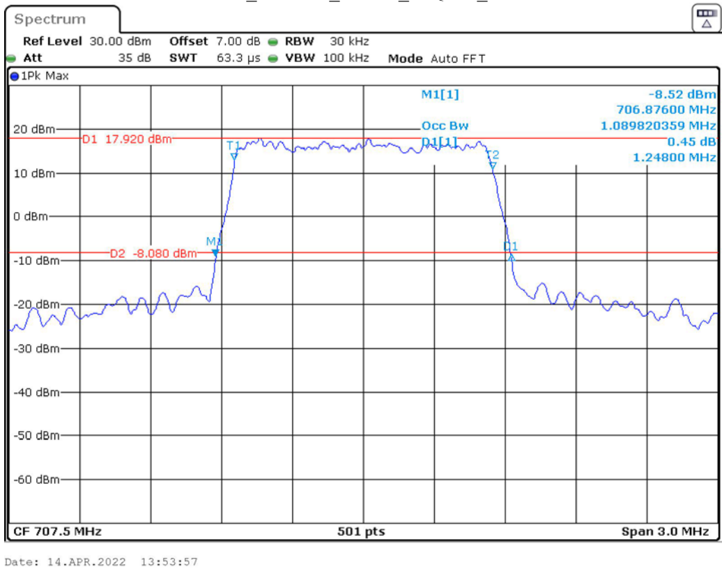
Band 12_1.4 MHz_Middle_16QAM_RB6#0
