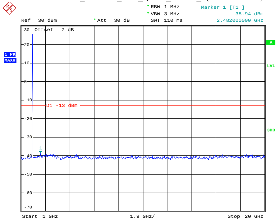
Band 2_1.4 MHz_Low_QPSK_RB6#0_2(1GHz-20GHz)
