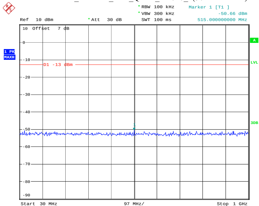
Band 2_1.4 MHz_Low_QPSK_RB6#0_1(30MHz-1GHz)
