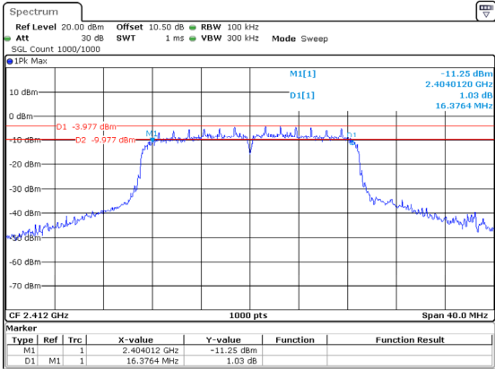
802.11n20_2412MHz 16.376MHz
