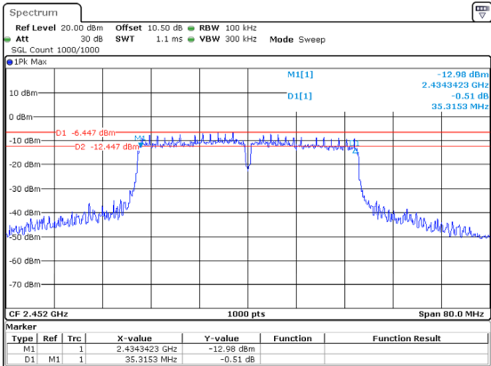
802.11n40_2452MHz 35.315MHz
