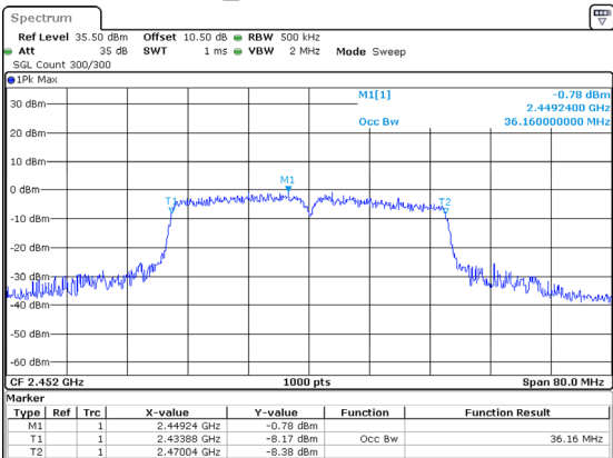
802.11n40_2452MHz 36.160MHz
