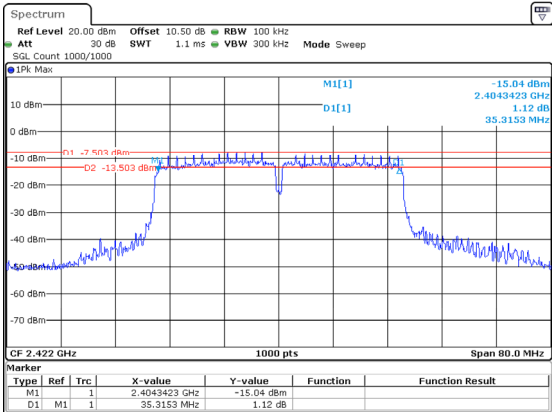
802.11n40_2422MHz 35.315MHz
