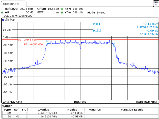
802.11n20_2437MHz 16.817MHz
