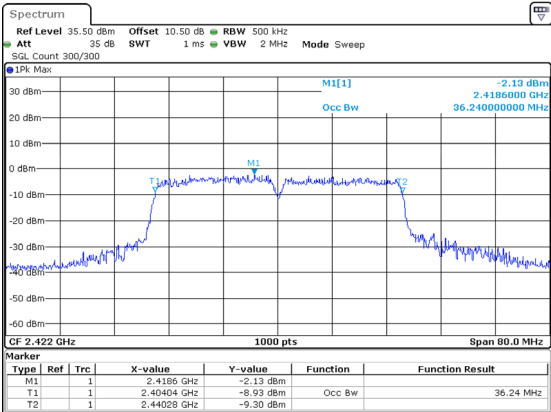
802.11n40_2422MHz 36.240MHz
