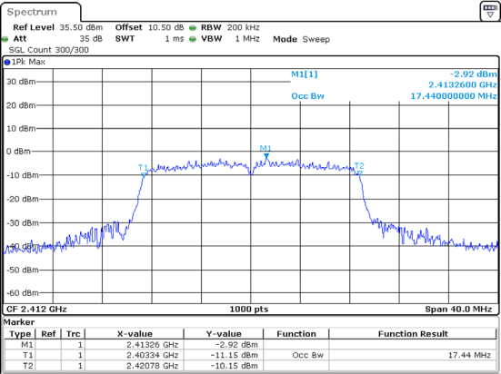
802.11n20_2412MHz 17.440MHz
