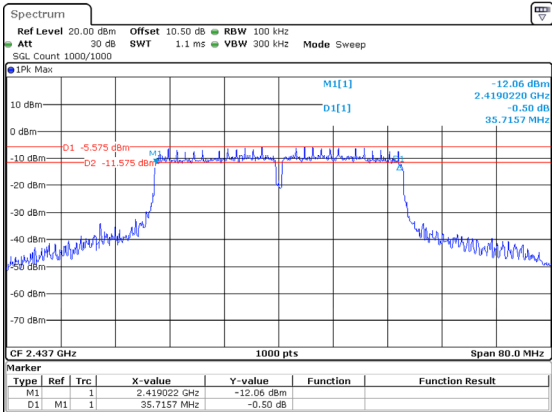
802.11n40_2437MHz 35.716MHz
