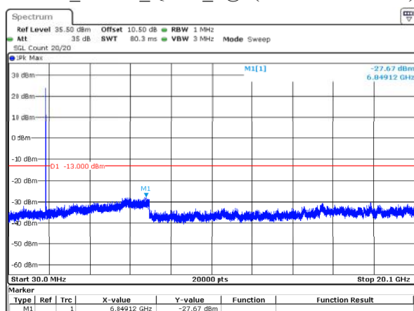
20MHz_Middle_QPSK_1@0(30MHz~20.1GHz)
