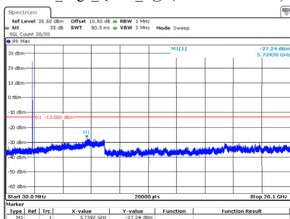
20MHz_High_QPSK_1@0(30MHz~20.1GHz)
