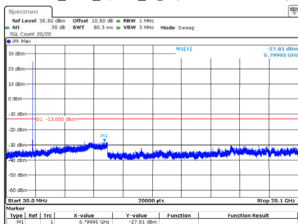
20MHz_Low_QPSK_1@0(30MHz~20.1GHz)
