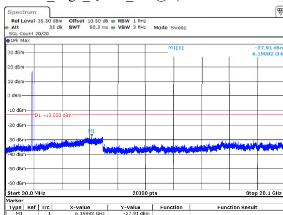
20MHz_High_QPSK_100@0(30MHz~20.1GHz)
