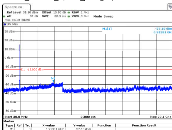
20MHz_Middle_QPSK_100@0(30MHz~20.1GHz)
