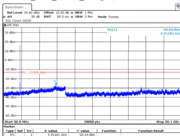
20MHz_Low_QPSK_100@0(30MHz~20.1GHz)
