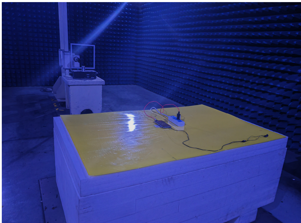
Photo of Radiated Emission Measurement (30MHz-1GHz)
