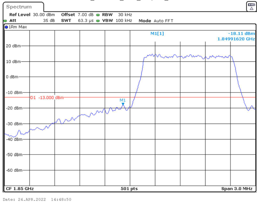
Band 2_1.4 MHz_Low_16QAM_RB6#0
