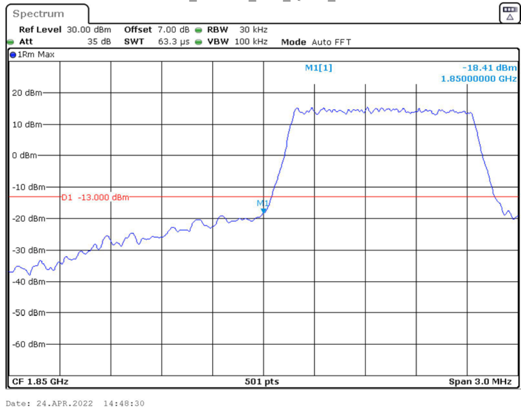
Band 2_1.4 MHz_Low_QPSK_RB6#0
