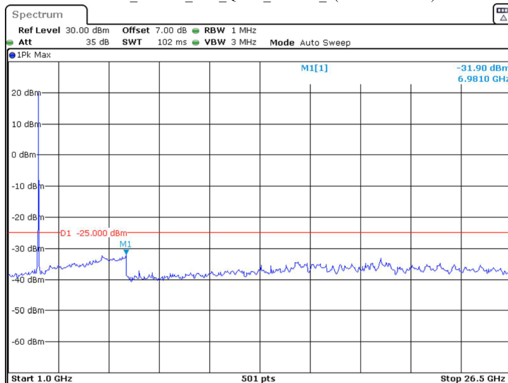
Band 41_15 MHz_Low_QPSK_RB75#0_2(1GHz-26.5GHz)
