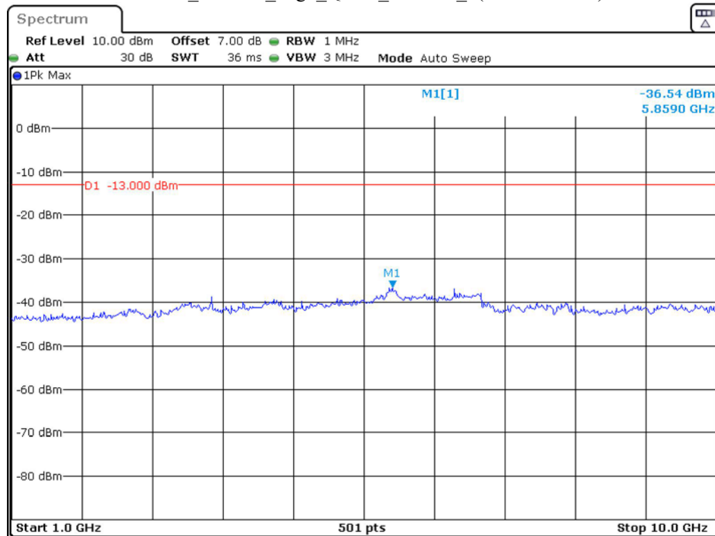
Band 12_10 MHz_High_QPSK_RB50#0_2(1GHz-10GHz)
