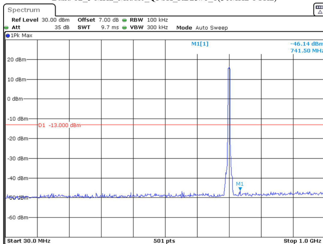
Band 12_5 MHz_Middle_QPSK_RB25#0_1(30MHz-1GHz)
