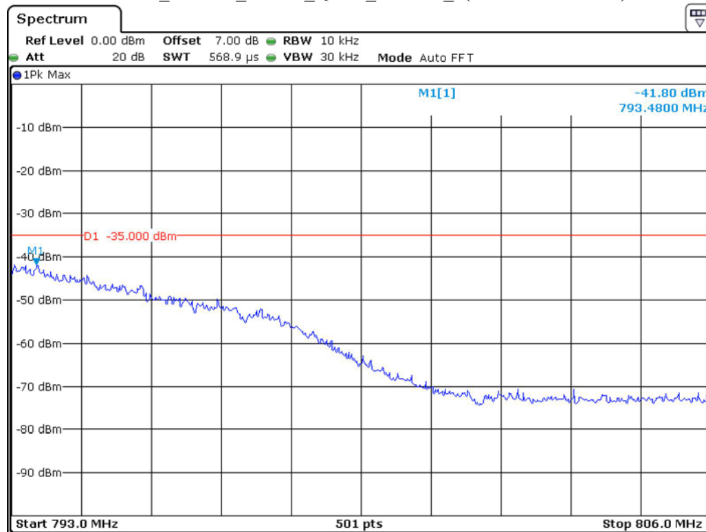
Band 13_10 MHz_Middle_QPSK_RB50#0_4(793MHz-806MHz)
