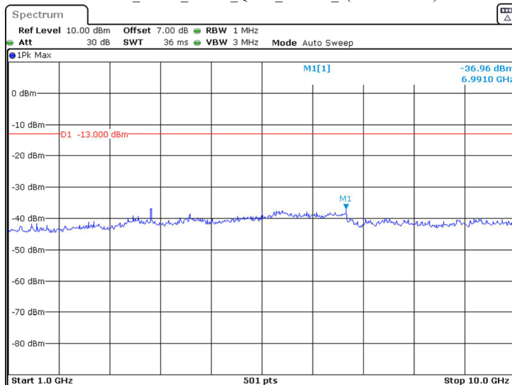
Band 12_5 MHz_Middle_QPSK_RB25#0_2(1GHz-10GHz)
