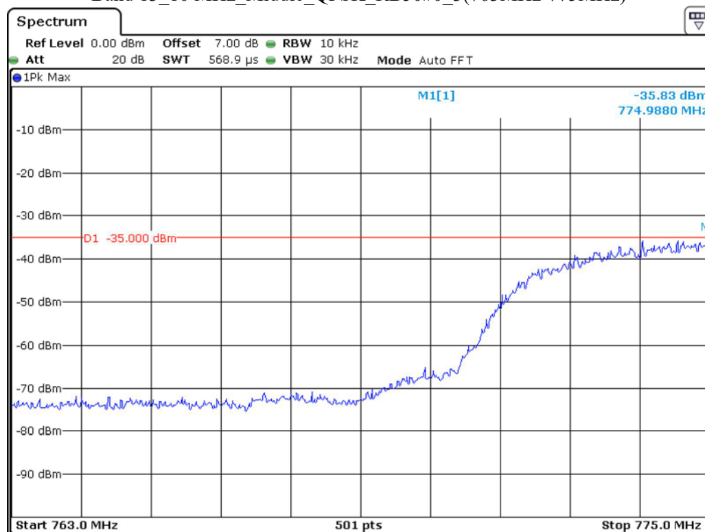
Band 13_10 MHz_Middle_QPSK_RB50#0_3(763MHz-775MHz)
