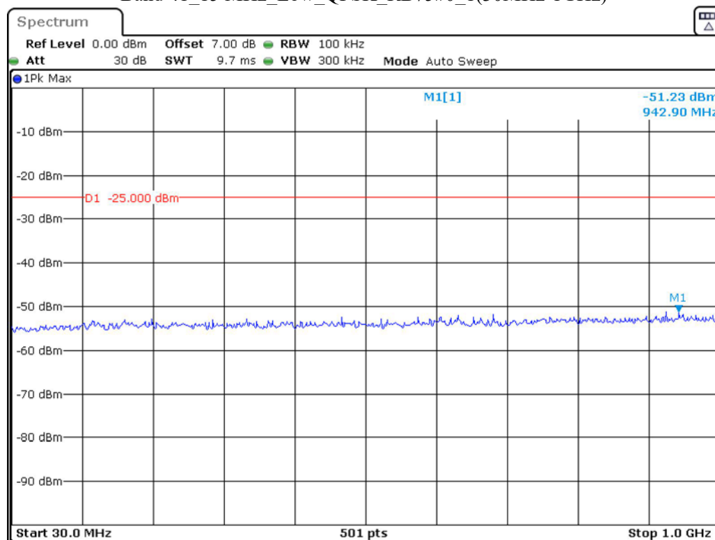
Band 41_15 MHz_Low_QPSK_RB75#0_1(30MHz-1GHz)
