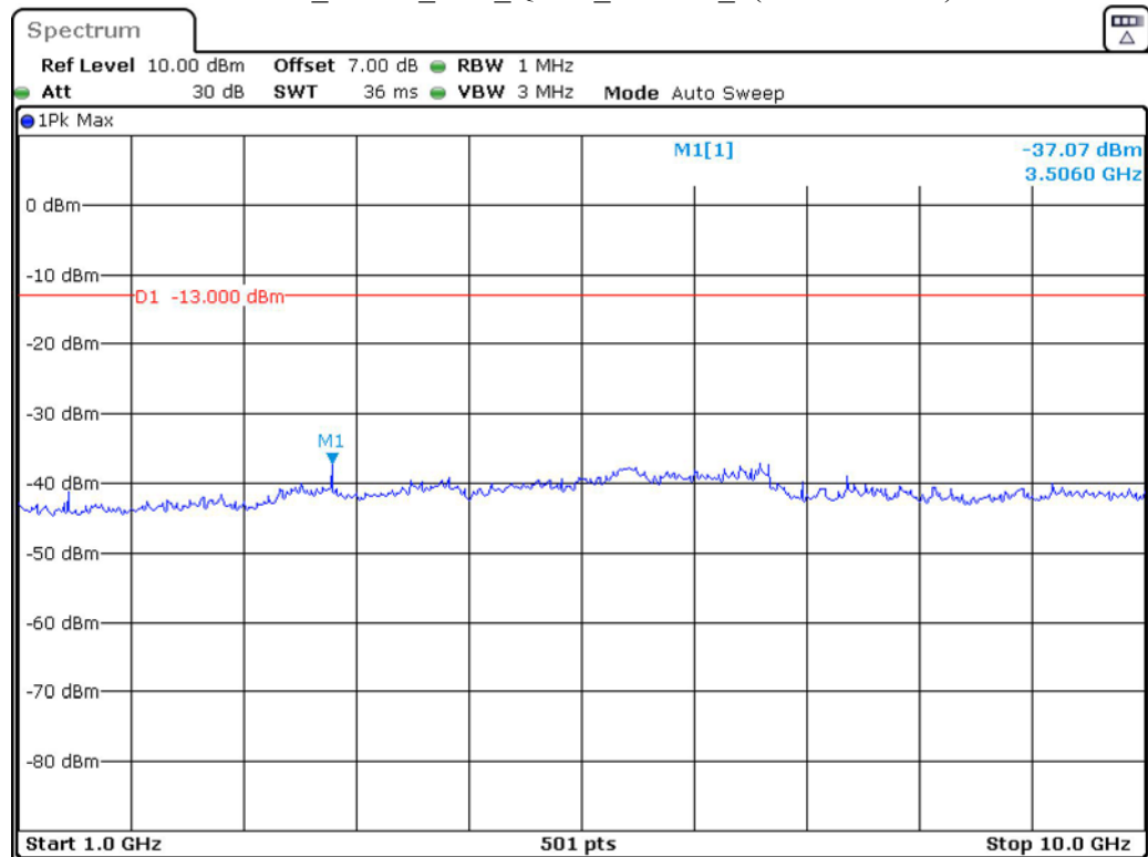
Band 12_3 MHz_Low_QPSK_RB15#0_2(1GHz-10GHz)
