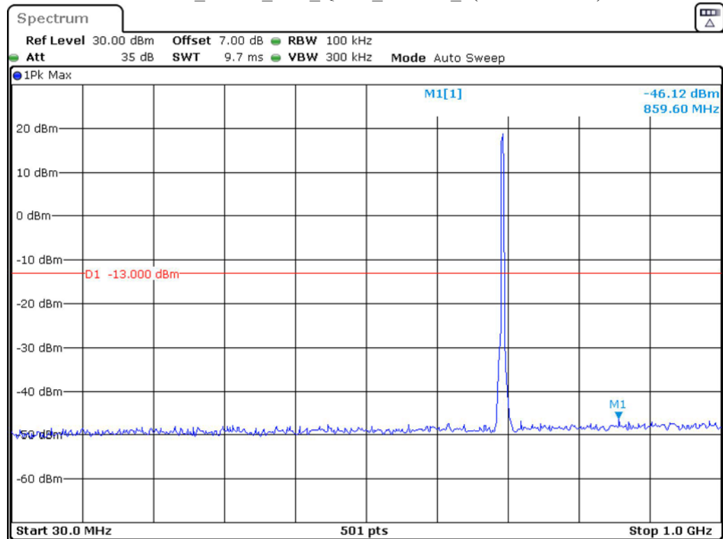
Band 12_3 MHz_Low_QPSK_RB15#0_1(30MHz-1GHz)
