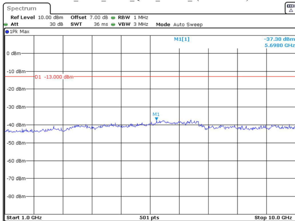
Band 5_3 MHz_Middle_QPSK_RB15#0_2(1GHz-10GHz)
