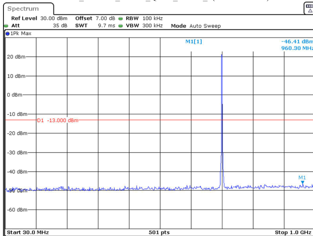
Band 12_1.4 MHz_Middle_QPSK_RB6#0_1(30MHz-1GHz)
