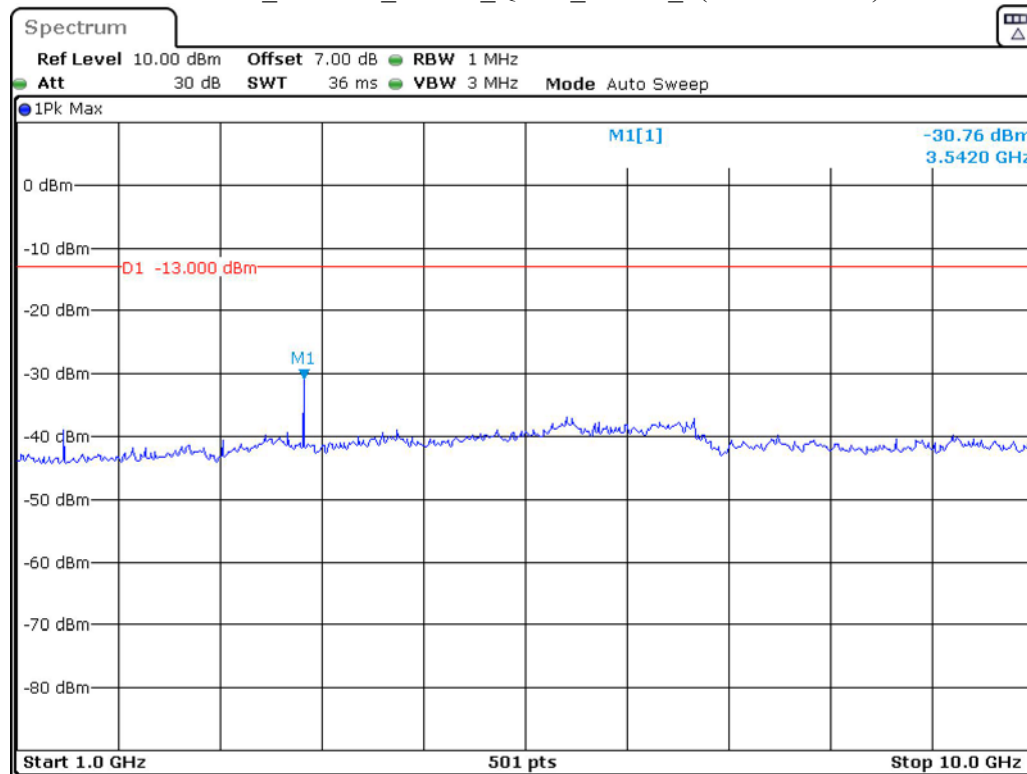
Band 12_1.4 MHz_Middle_QPSK_RB6#0_2(1GHz-10GHz)
