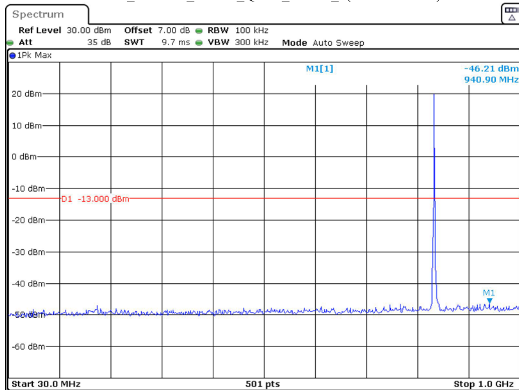
Band 5_1.4 MHz_Middle_QPSK_RB6#0_1(30MHz-1GHz)
