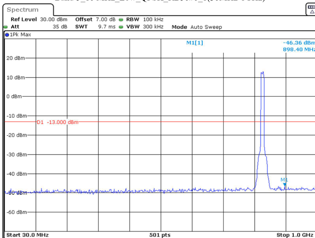
Band 5_10 MHz_Low_QPSK_RB50#0_1(30MHz-1GHz)
