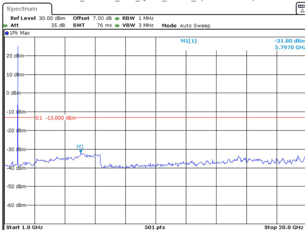
Band 2_1.4 MHz_Low_QPSK_RB6#0_2(1GHz-20GHz)
