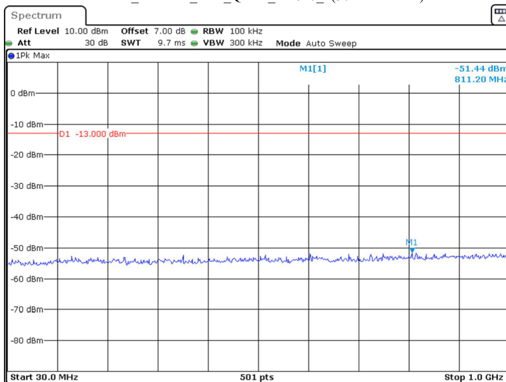
Band 2_1.4 MHz_Low_QPSK_RB6#0_1(30MHz-1GHz)
