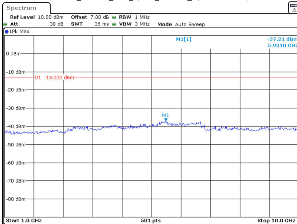
Band 5_10 MHz_Low_QPSK_RB50#0_2(1GHz-10GHz)
