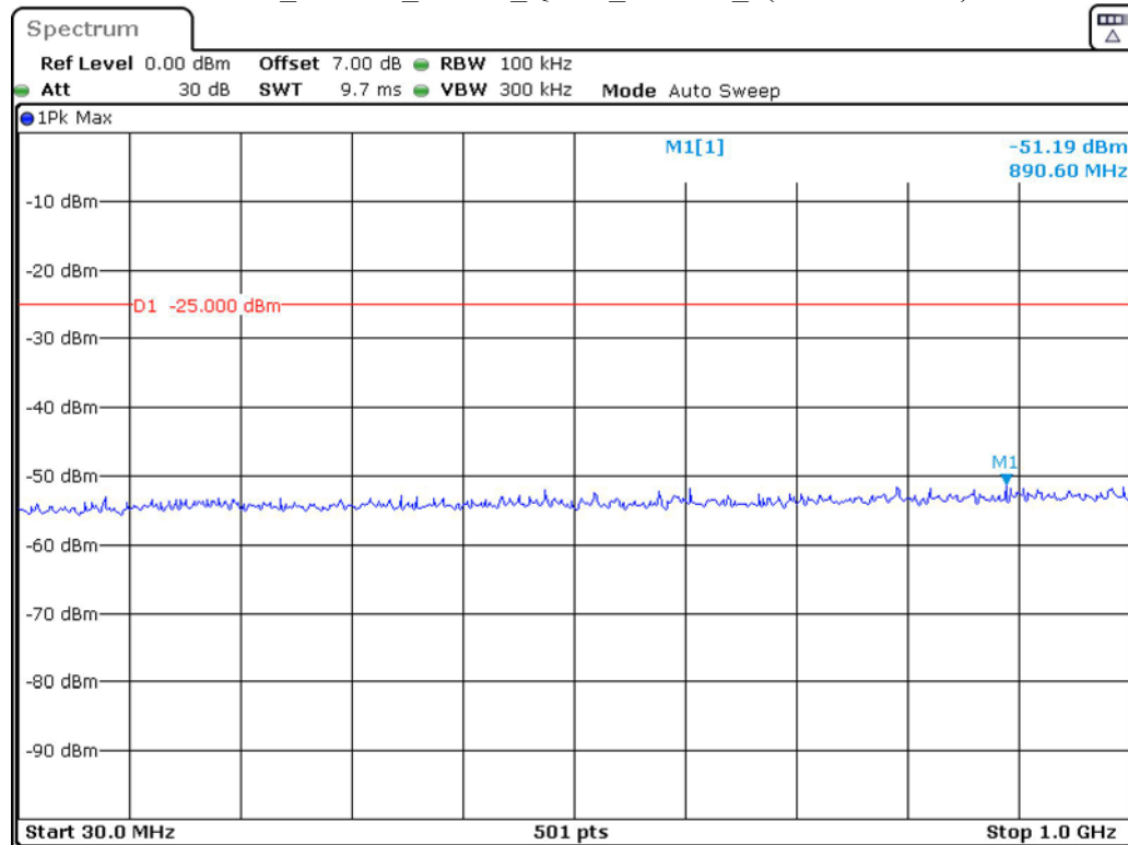
Band 41_10 MHz_Middle_QPSK_RB50#0_1(30MHz-1GHz)
