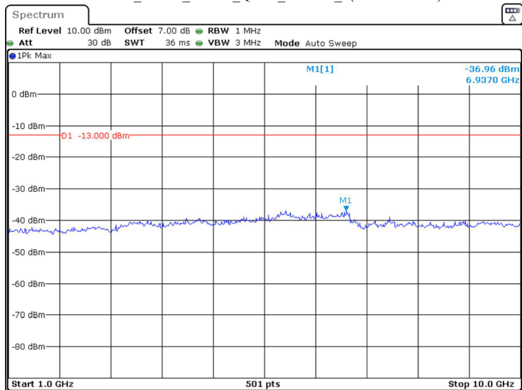
Band 12_5 MHz_Middle_QPSK_RB25#0_2(1GHz-10GHz)
