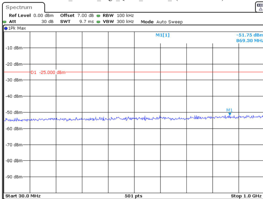
Band 41_10 MHz_High_QPSK_RB50#0_1(30MHz-1GHz)
