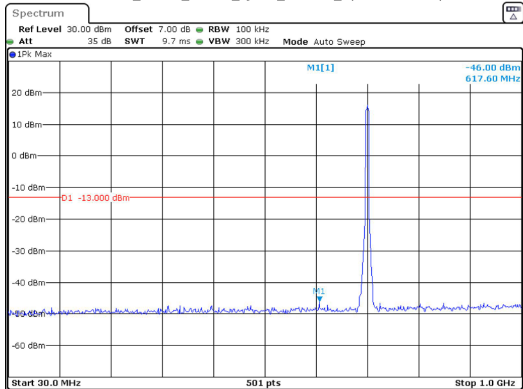
Band 12_5 MHz_Middle_QPSK_RB25#0_1(30MHz-1GHz)
