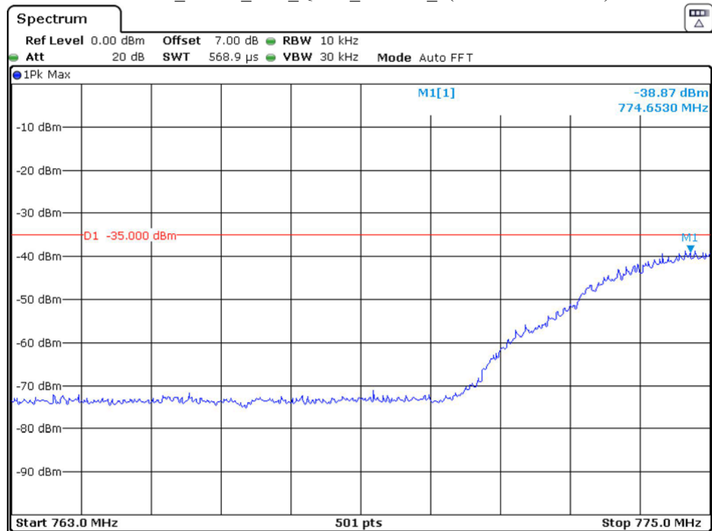
Band 13_5 MHz_Low_QPSK_RB25#0_2(763MHz-775MHz)
