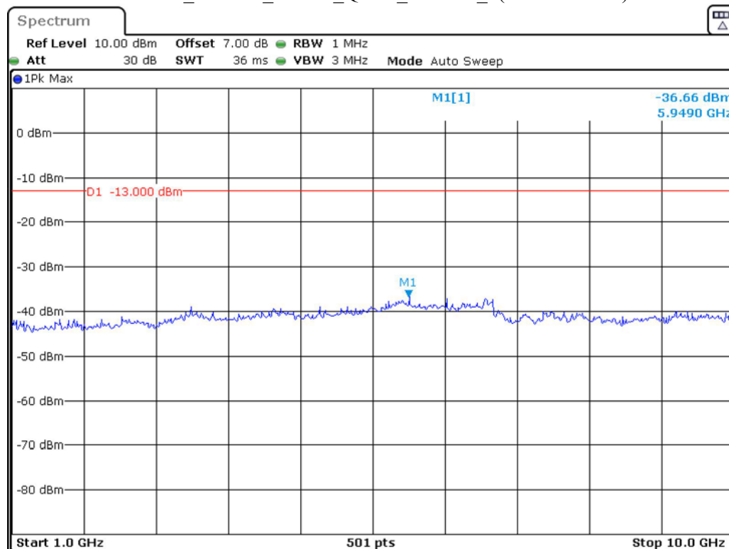
Band 13_10 MHz_Middle_QPSK_RB50#0_2(1GHz-10GHz)
