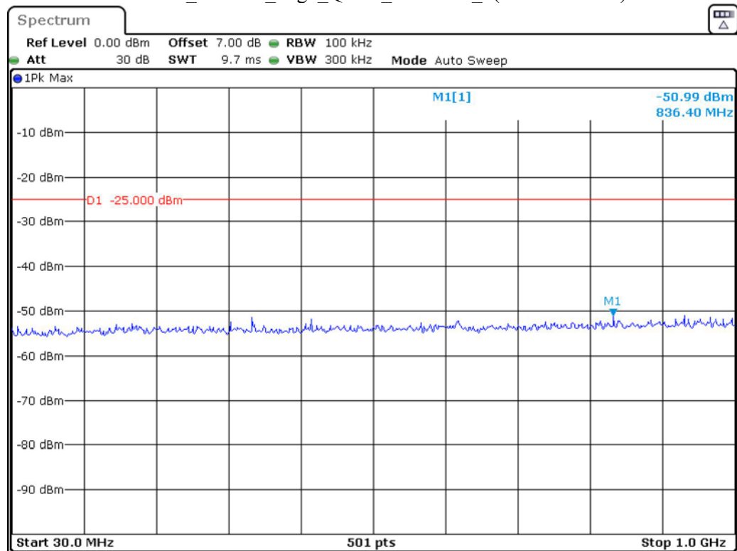
Band 41_20 MHz_High_QPSK_RB100#0_1(30MHz-1GHz)
