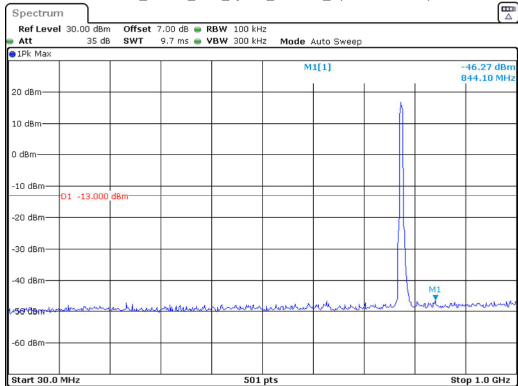
Band 13_5 MHz_Low_QPSK_RB25#0_1(30MHz-1GHz)
