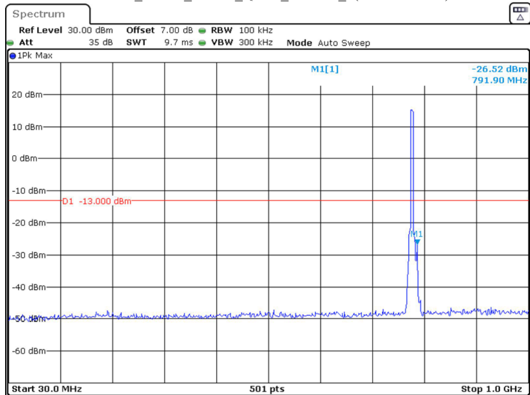
Band 13_5 MHz_Middle_QPSK_RB25#0_1(30MHz-1GHz)
