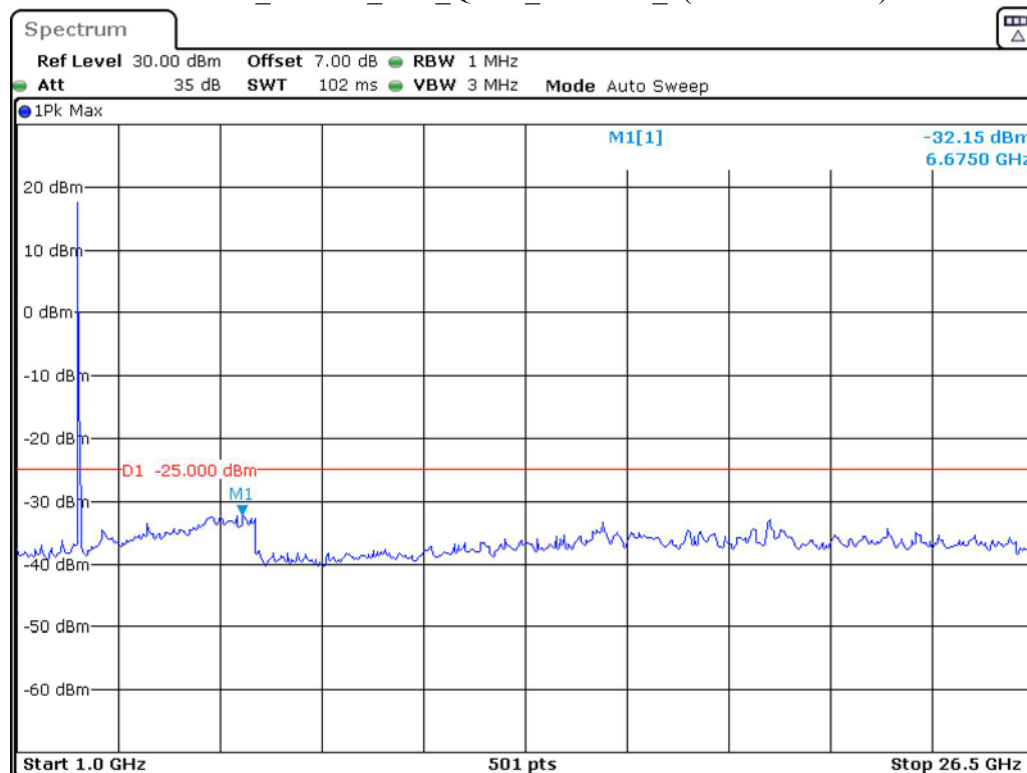
Band 41_20 MHz_Low_QPSK_RB100#0_2(1GHz-26.5GHz)
