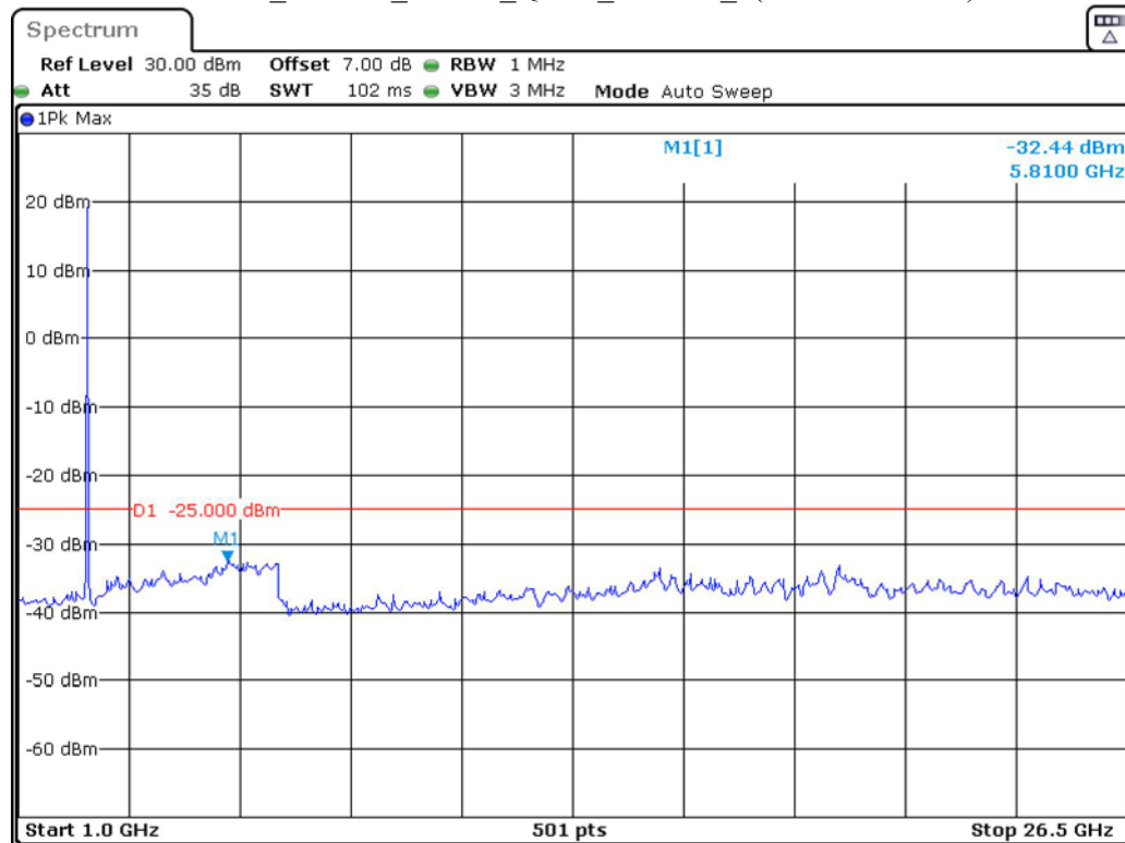
Band 41_10 MHz_Middle_QPSK_RB50#0_2(1GHz-26.5GHz)
