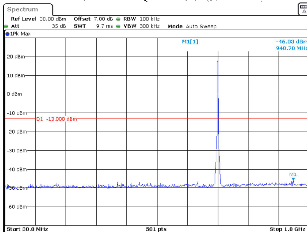
Band 12_3 MHz_Middle_QPSK_RB15#0_1(30MHz-1GHz)
