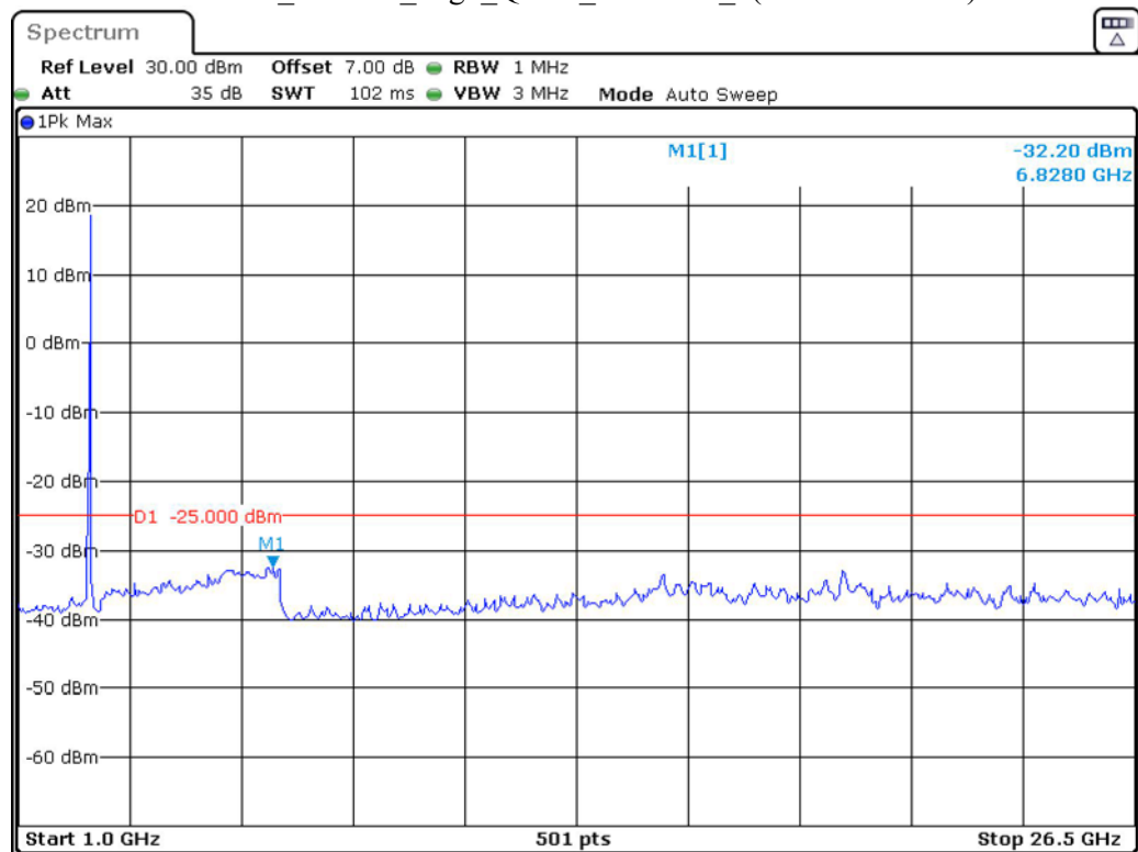
Band 41_20 MHz_High_QPSK_RB100#0_2(1GHz-26.5GHz)
