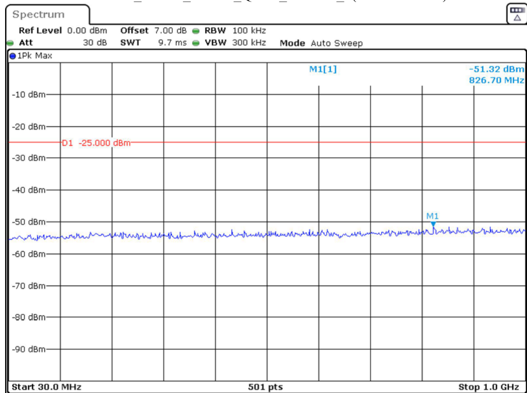
Band 41_5 MHz_Middle_QPSK_RB25#0_1(30MHz-1GHz)
