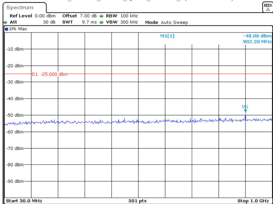
Band 41_15 MHz_Middle_QPSK_RB75#0_1(30MHz-1GHz)
