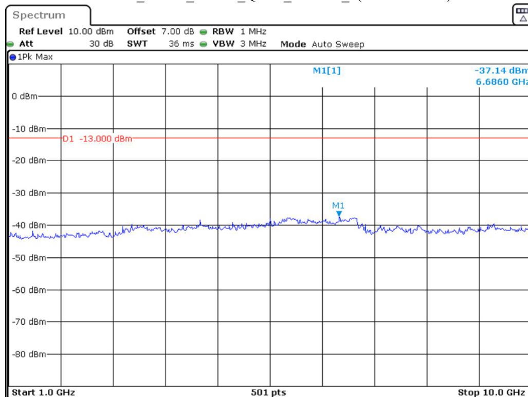
Band 12_3 MHz_Middle_QPSK_RB15#0_2(1GHz-10GHz)
