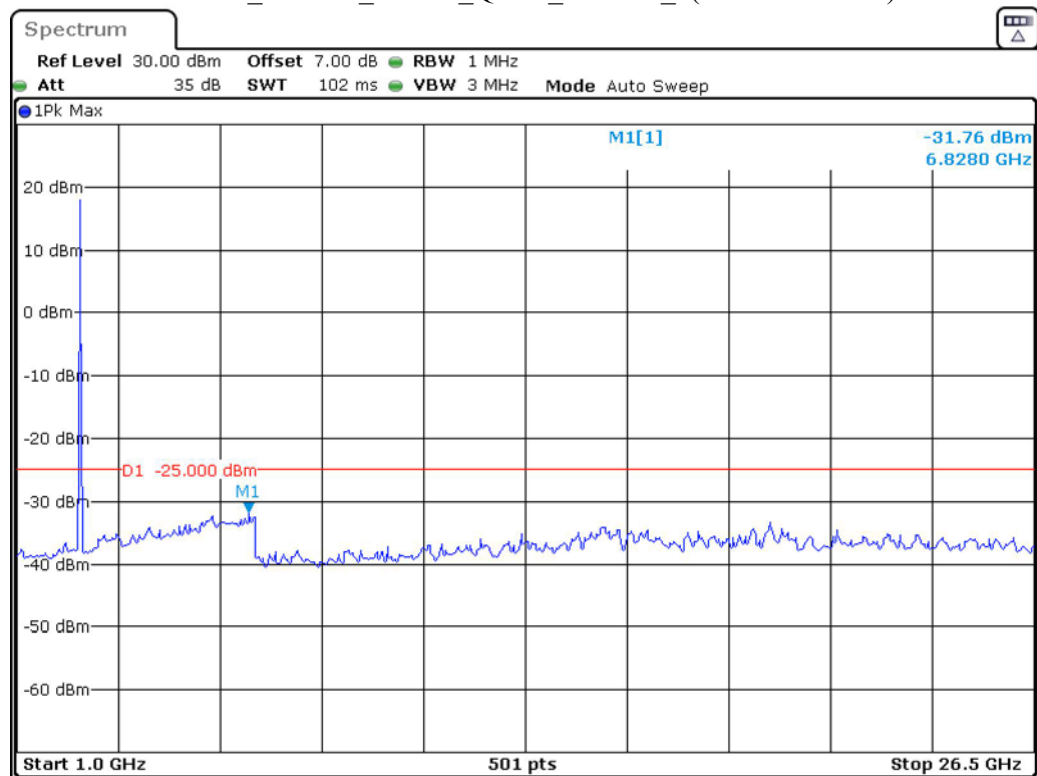
Band 41_15 MHz_Middle_QPSK_RB75#0_2(1GHz-26.5GHz)
