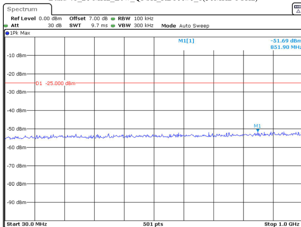
Band 41_20 MHz_Low_QPSK_RB100#0_1(30MHz-1GHz)
