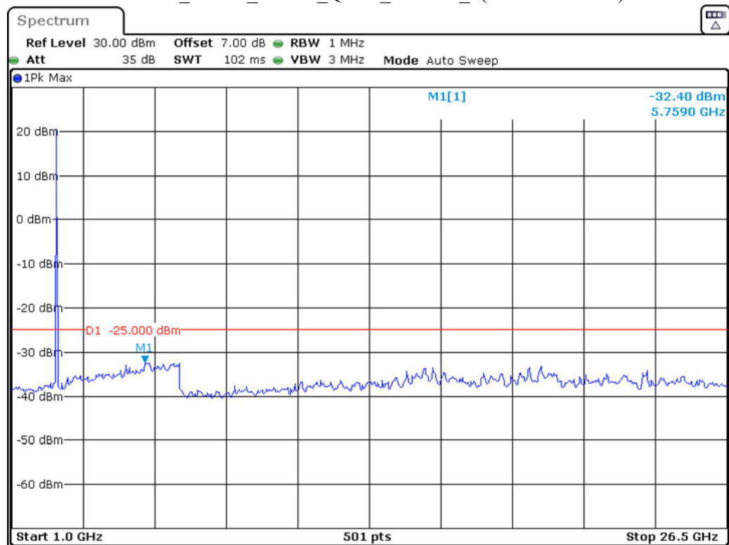
Band 41_5 MHz_Middle_QPSK_RB25#0_2(1GHz-26.5GHz)
