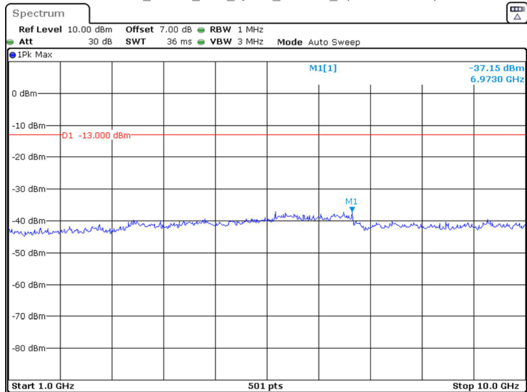
Band 13_5 MHz_Low_QPSK_RB25#0_2(1GHz-10GHz)
