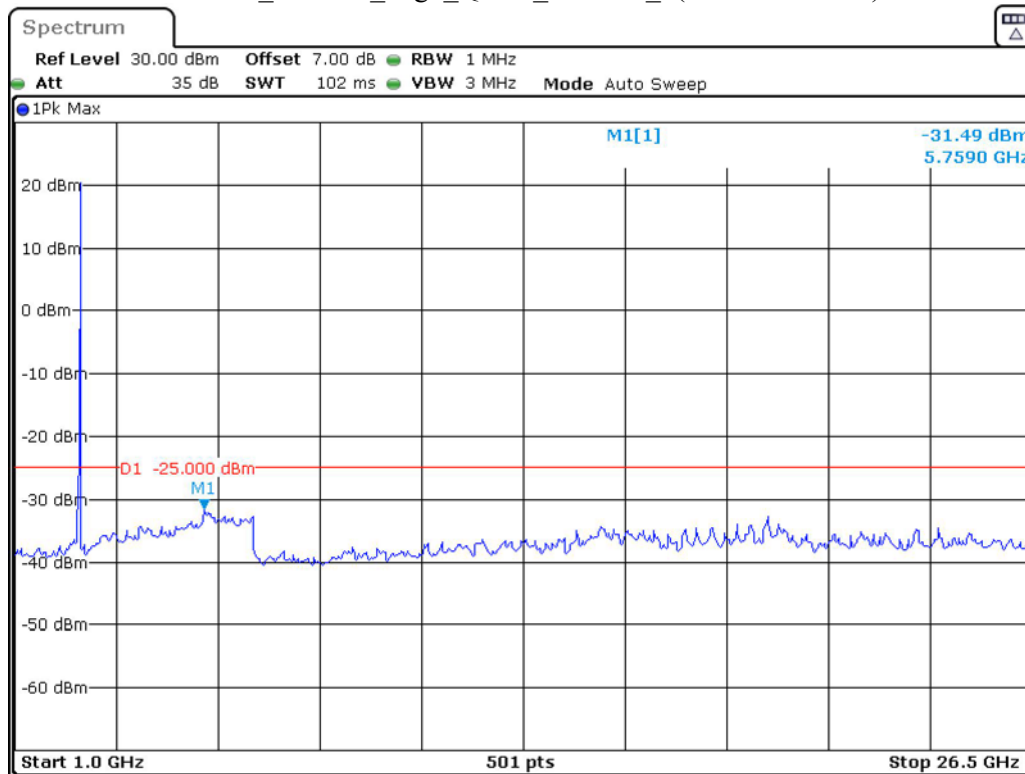
Band 41_10 MHz_High_QPSK_RB50#0_2(1GHz-26.5GHz)
