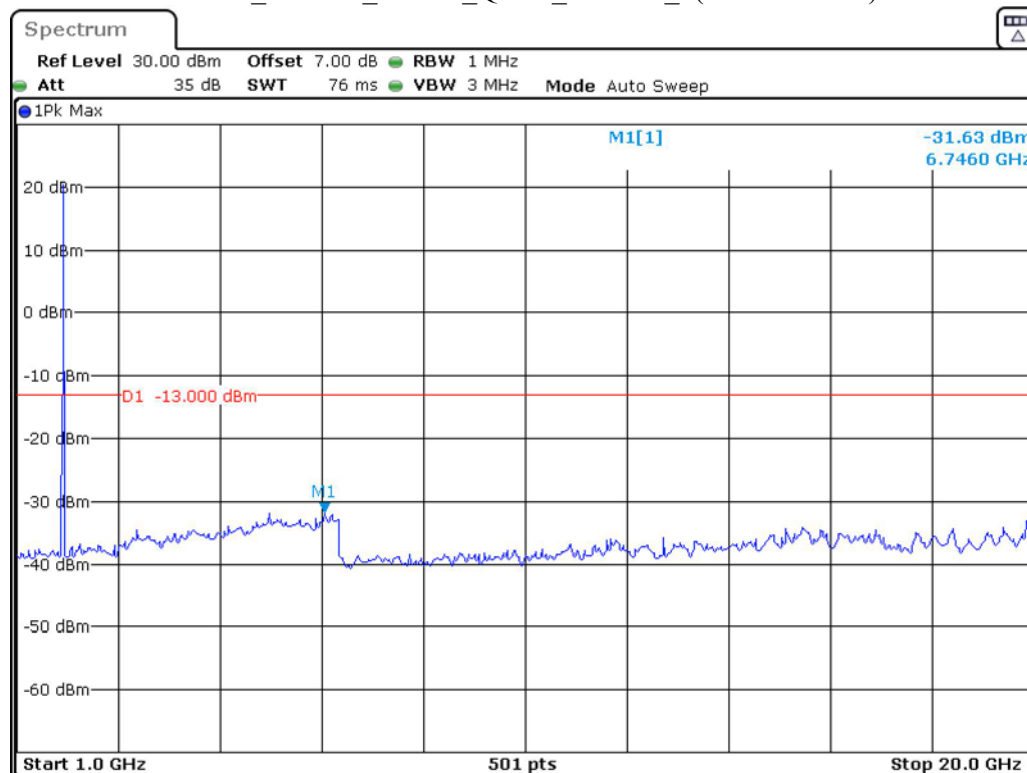
Band 2_10 MHz_Middle_QPSK_RB50#0_2(1GHz-20GHz)
