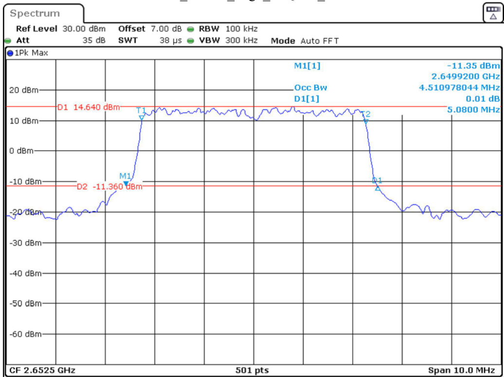
Band 41_5 MHz_High_16QAM_RB25#0
