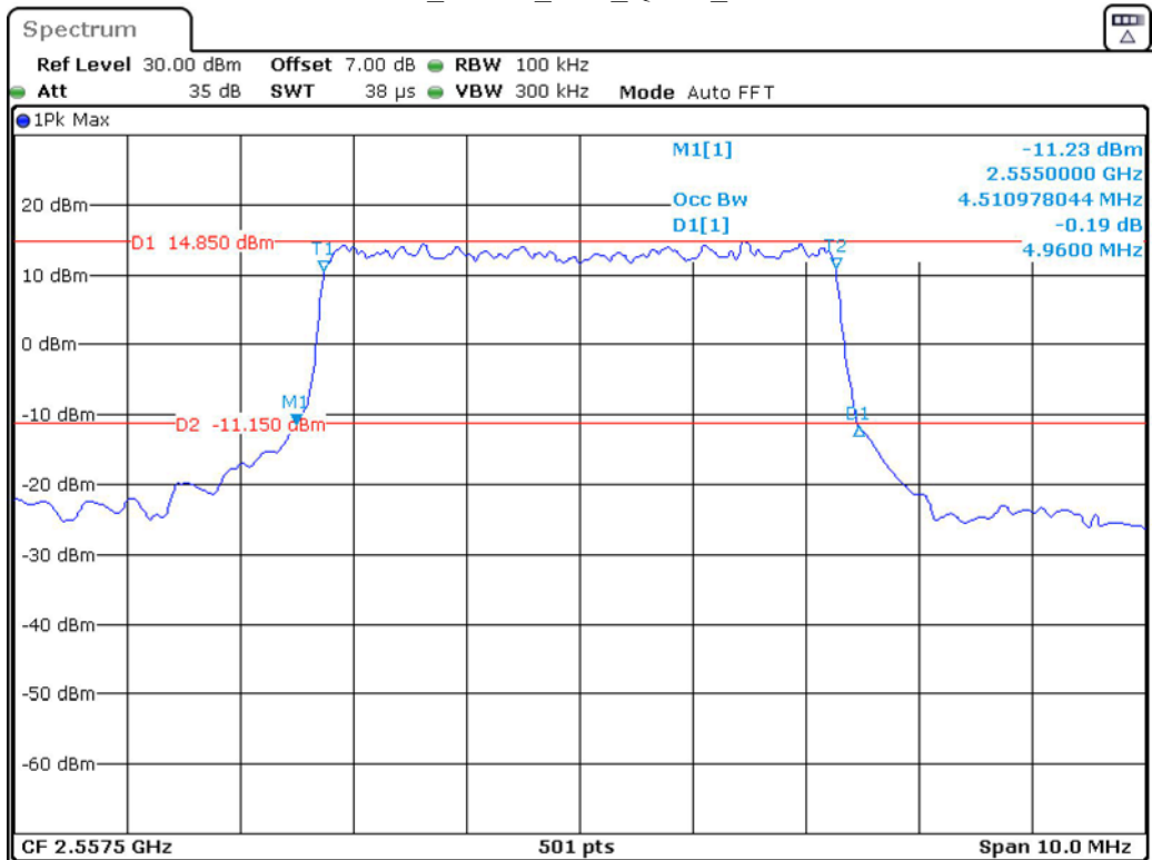
Band 41_5 MHz_Low_QPSK_RB25#0
