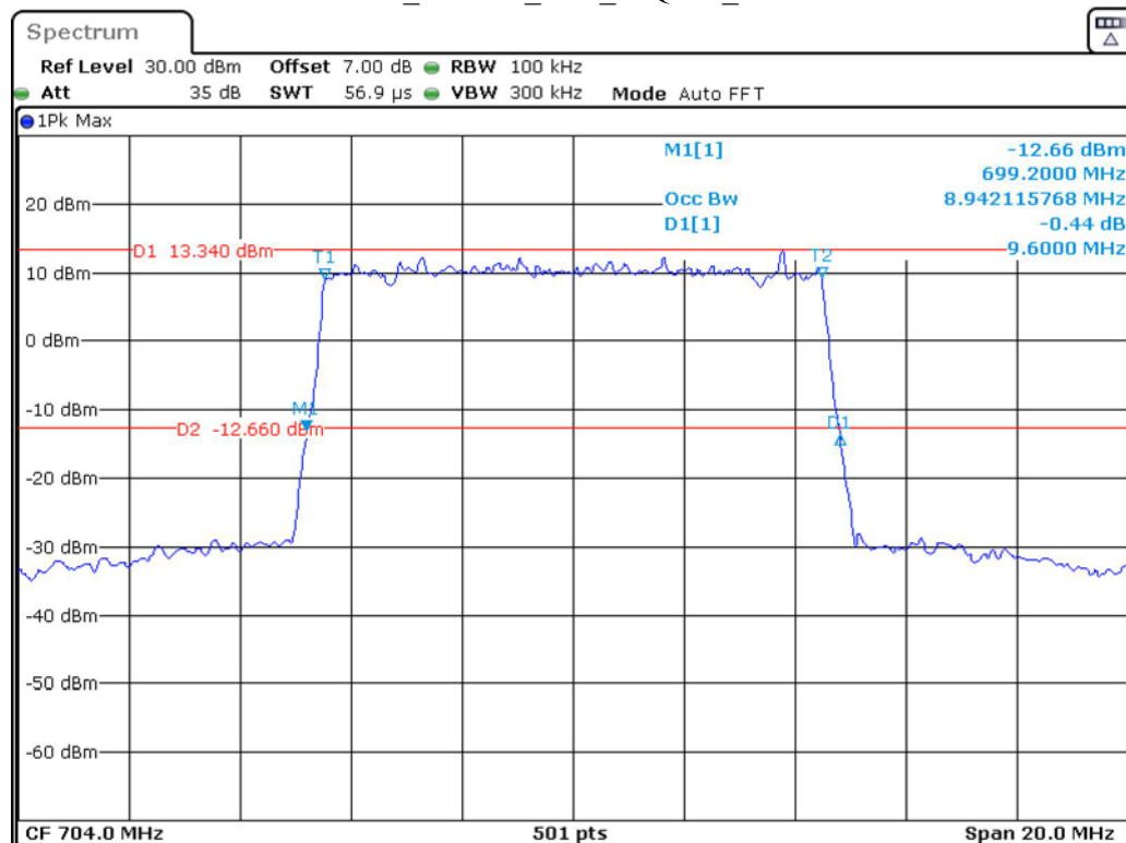
Band 12_10 MHz_Low_16QAM_RB50#0
