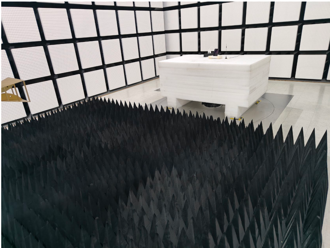
Radiated Emission Above 1GHz View-RX
