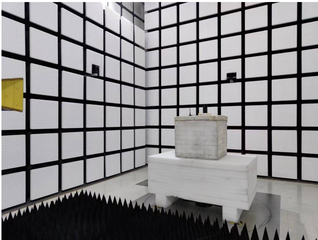
Radiated Emission Above 1GHz View-TX
