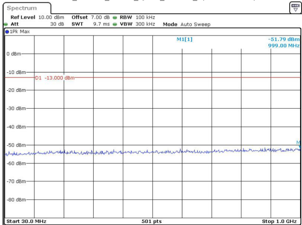
Band 2_15 MHz_Middle_QPSK_RB75#0_1(30MHz-1GHz)
