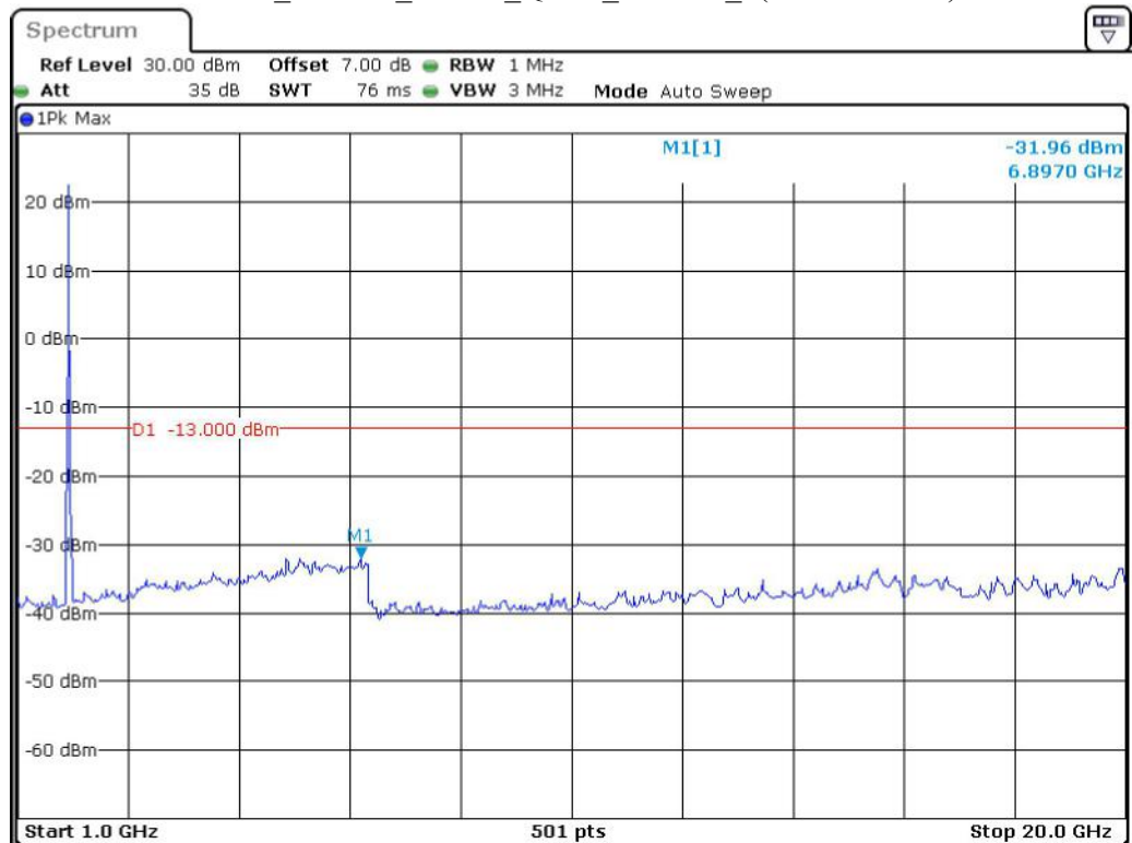
Band 2_15 MHz_Middle_QPSK_RB75#0_2(1GHz-20GHz)
