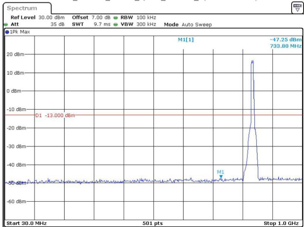
Band 5_10 MHz_Middle_QPSK_RB50#0_1(30MHz-1GHz)
