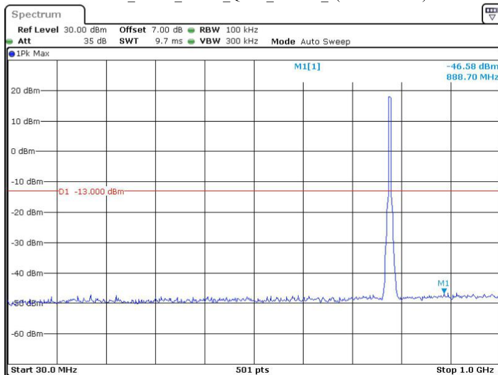
Band 13_5 MHz_Middle_QPSK_RB25#0_1(30MHz-1GHz)
