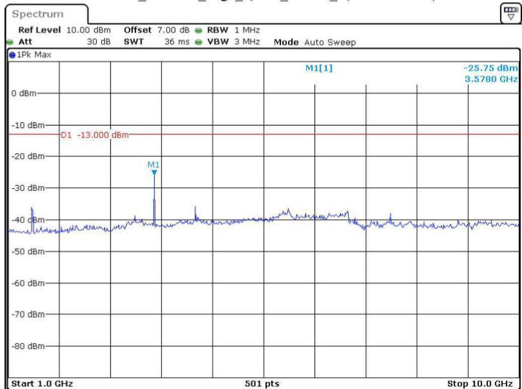
Band 12_1.4 MHz_High_QPSK_RB6#0_2(1GHz-10GHz)
