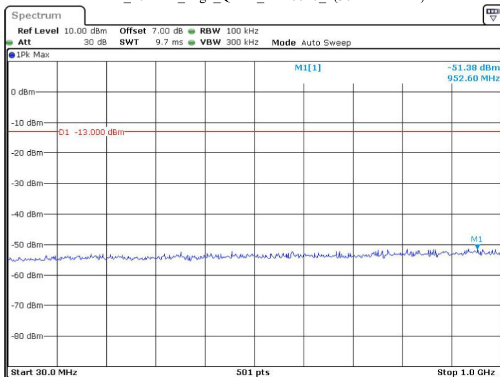
Band 2_20 MHz_High_QPSK_RB100#0_1(30MHz-1GHz)
