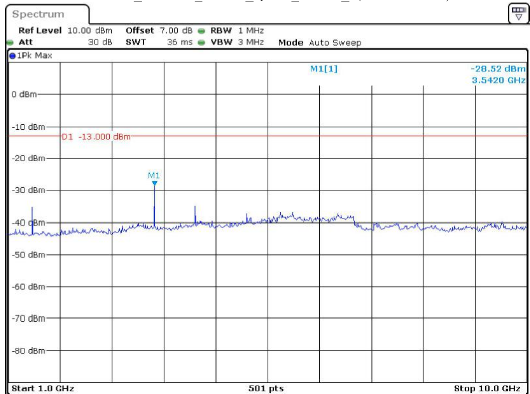
Band 12_1.4 MHz_Middle_QPSK_RB6#0_2(1GHz-10GHz)
