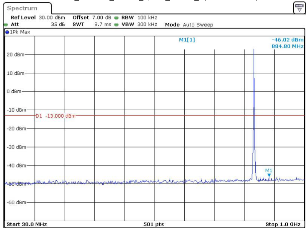
Band 5_1.4 MHz_Middle_QPSK_RB6#0_1(30MHz-1GHz)
