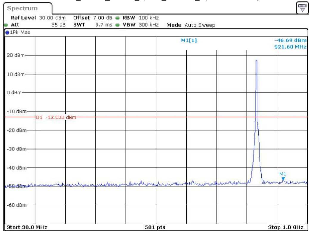
Band 5_5 MHz_Middle_QPSK_RB25#0_1(30MHz-1GHz)
