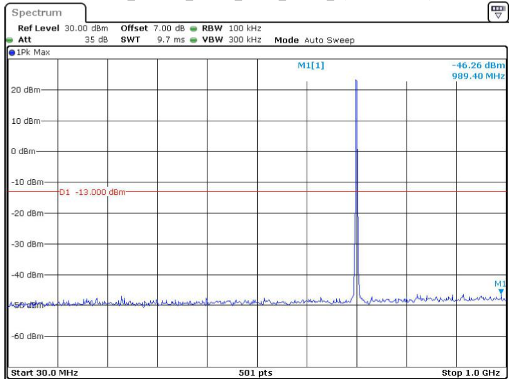
Band 12_1.4 MHz_Middle_QPSK_RB6#0_1(30MHz-1GHz)
