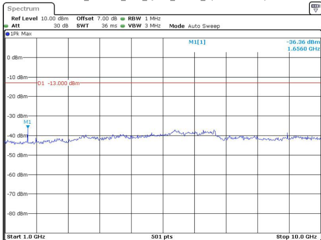
Band 5_1.4 MHz_Low_QPSK_RB6#0_2(1GHz-10GHz)
