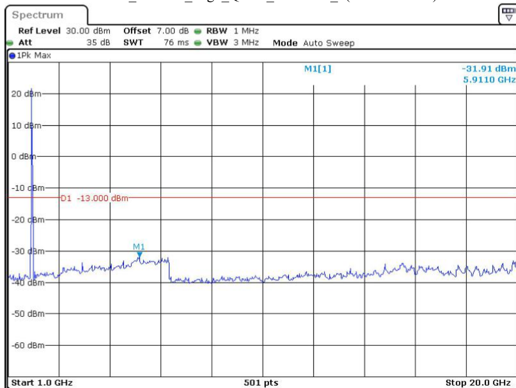
Band 2_20 MHz_High_QPSK_RB100#0_2(1GHz-20GHz)
