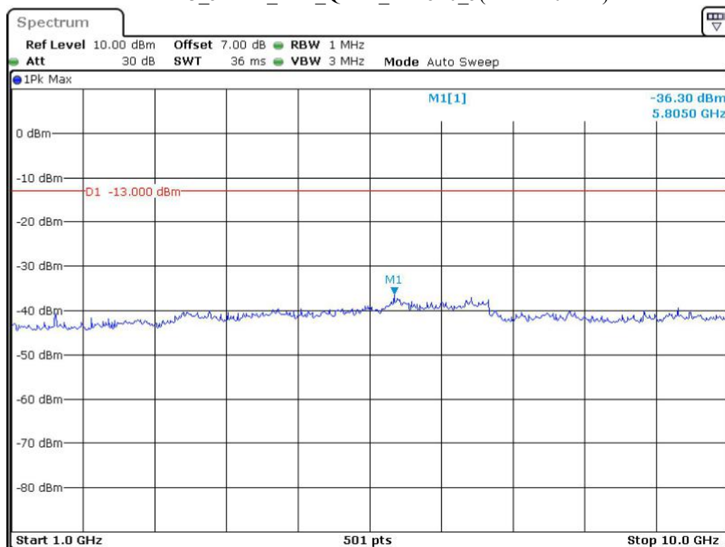
Band 13_5 MHz_Low_QPSK_RB25#0_5(1GHz-10GHz)
