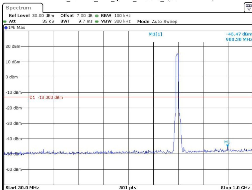
Band 12_10 MHz_Low_QPSK_RB50#0_1(30MHz-1GHz)
