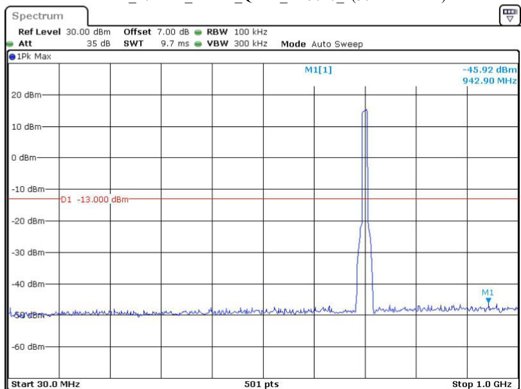
Band 12_10 MHz_Middle_QPSK_RB50#0_1(30MHz-1GHz)
