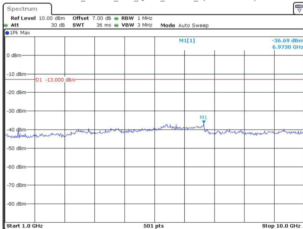
Band 12_10 MHz_Low_QPSK_RB50#0_2(1GHz-10GHz)
