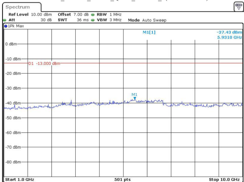
Band 12_10 MHz_Middle_QPSK_RB50#0_2(1GHz-10GHz)
