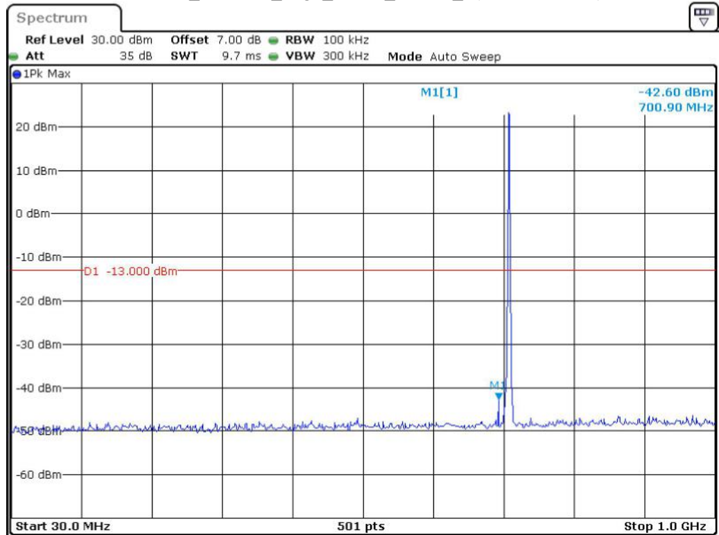
Band 12_1.4 MHz_High_QPSK_RB6#0_1(30MHz-1GHz)
