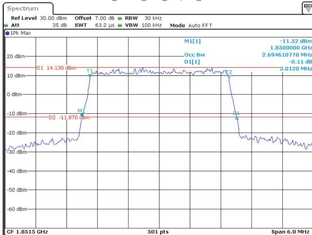
Band 2_3 MHz_Low_16QAM_RB15#0
