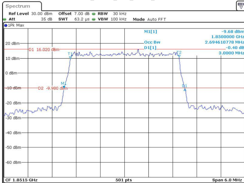
Band 2_3 MHz_Low_QPSK_RB15#0
