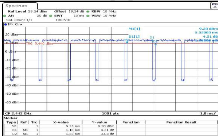
11N20SISO_Ant1_2442
