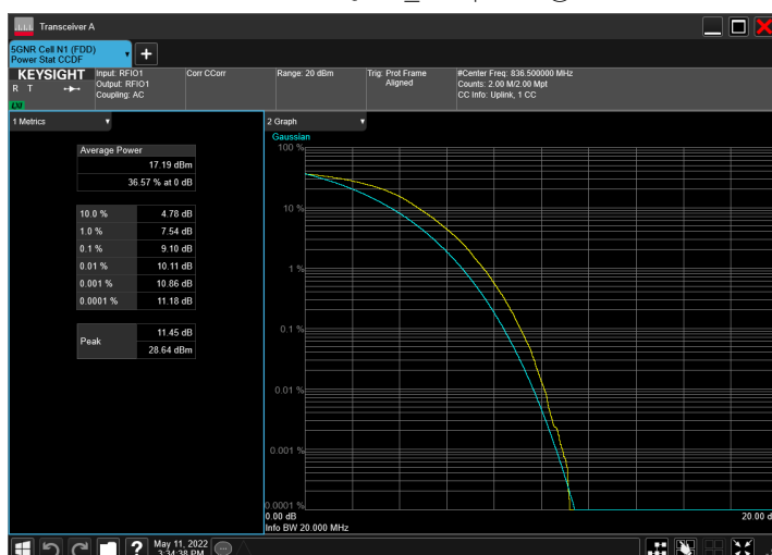
DC_2A_n5A_10MHz|15MHz_15kHz_1880MHz|836.5MHz_CP -OFDM 64 QAM_RB0|RB79@0
