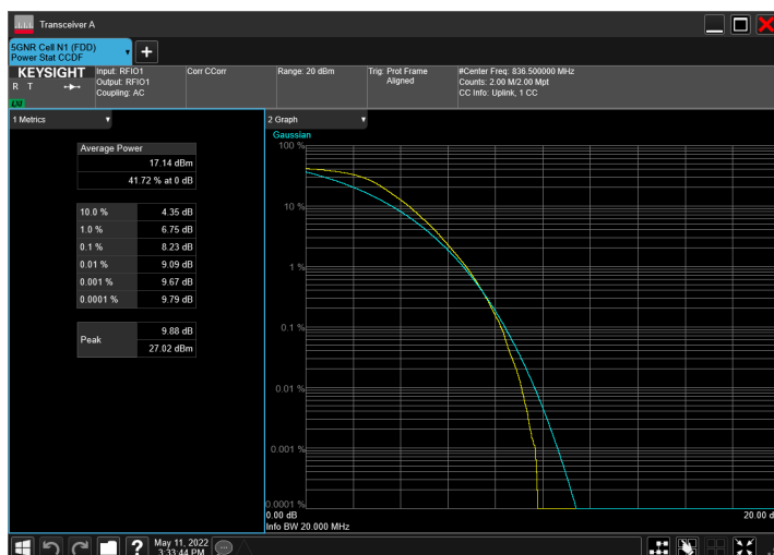
DC_2A_n5A_10MHz|15MHz_15kHz_1880MHz|836.5MHz_CP -OFDM QPSK_RB0|RB79@0
