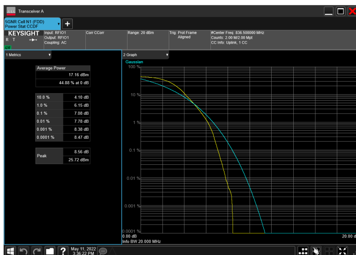
DC_2A_n5A_10MHz|20MHz_15kHz_1880MHz|836.5MHz_DF T-s-OFDM PI/2 BPSK_RB0|RB100@0
