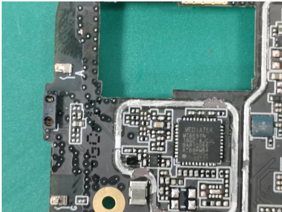
Main antenna
