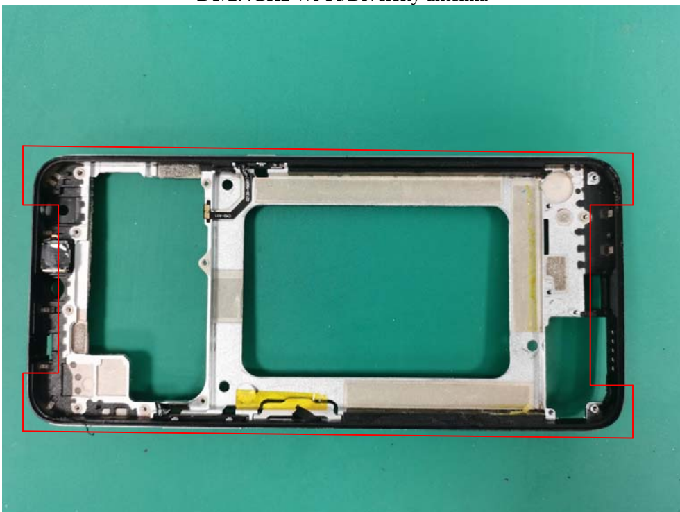
BT/2.4GHz Wi-Fi/Diversity antenna
