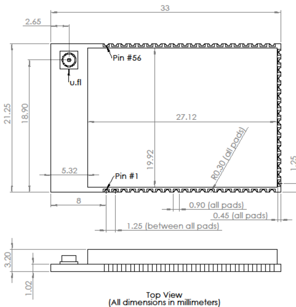
Figure 1: Mechanical dimensions
