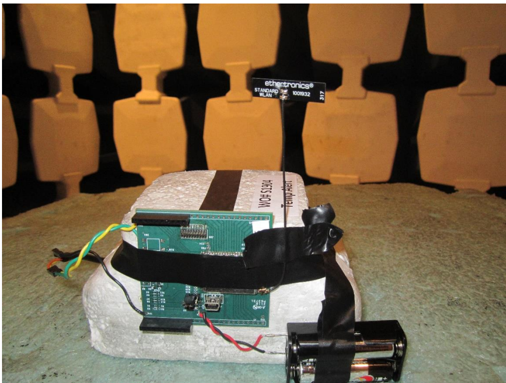
External Antenna – Horizontal Orientation
