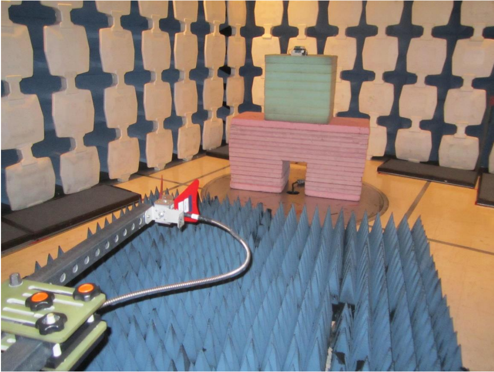
1-6GHz
