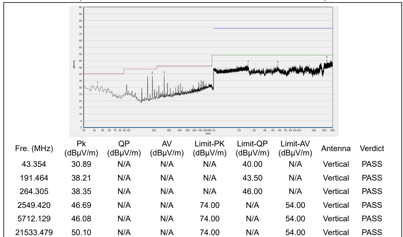
(30MHz to 25GHz, Antenna Vertical, 8-DPSK, channel 78)
