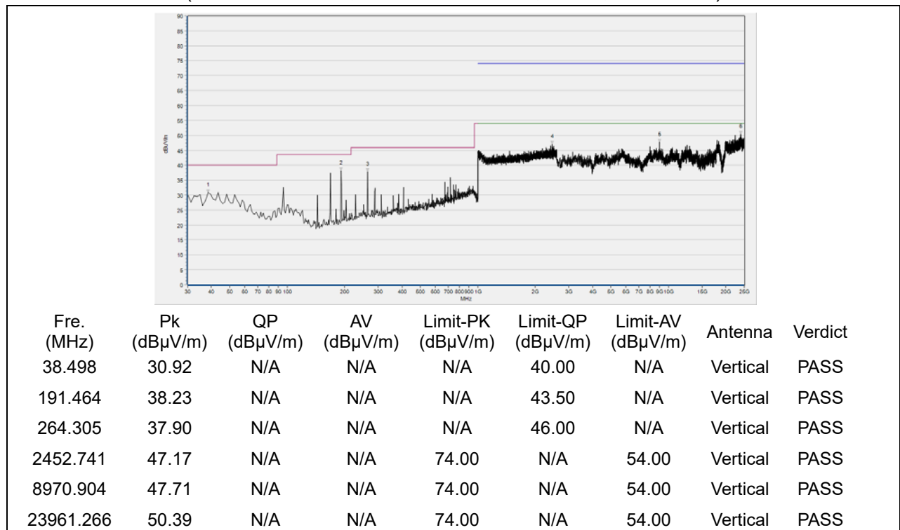
(30MHz to 25GHz, Antenna Vertical, GFSK, channel 78)
