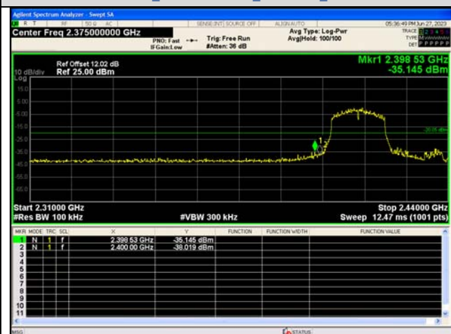
Out Of Band Emission IEEE 802.11g_Channel 1_20MHz_Antenna 0
