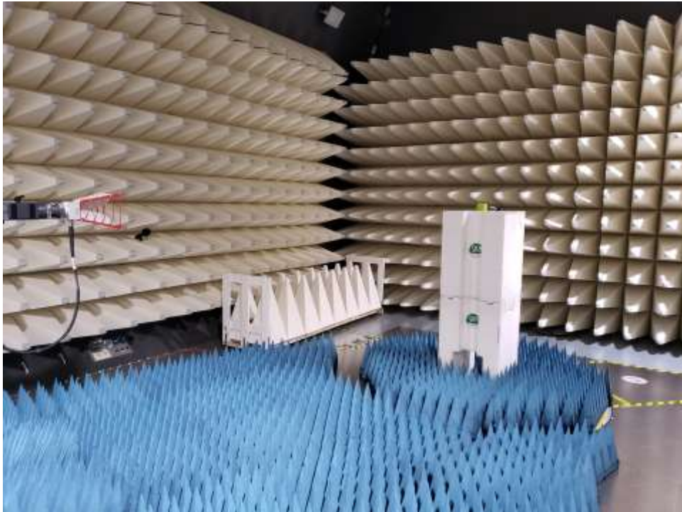
5. Radiated Emission test setup High Range
