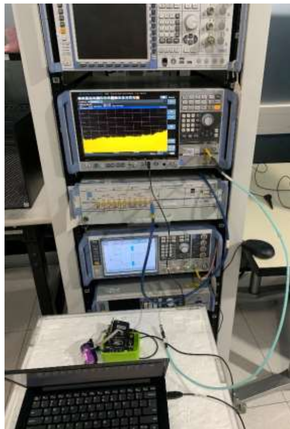
6. Conducted test setup
