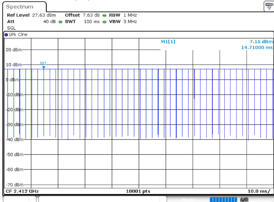
Duty Cycle NVNT 802.11b 2412MHz Ant 1
