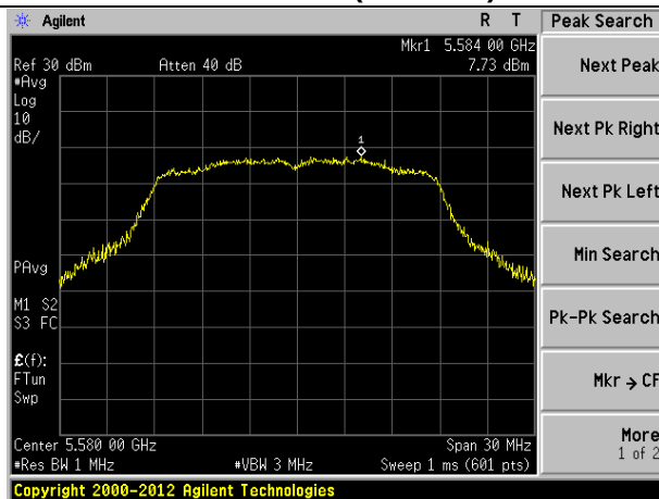
Channel 116 (5580MHz)
