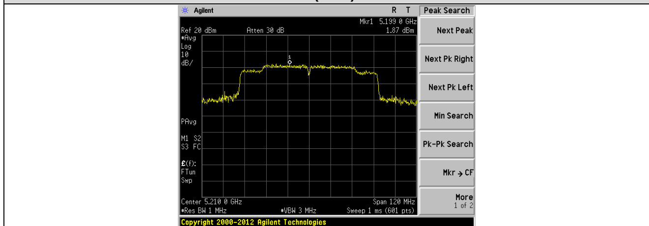
Channel 40 (5210MHz)
