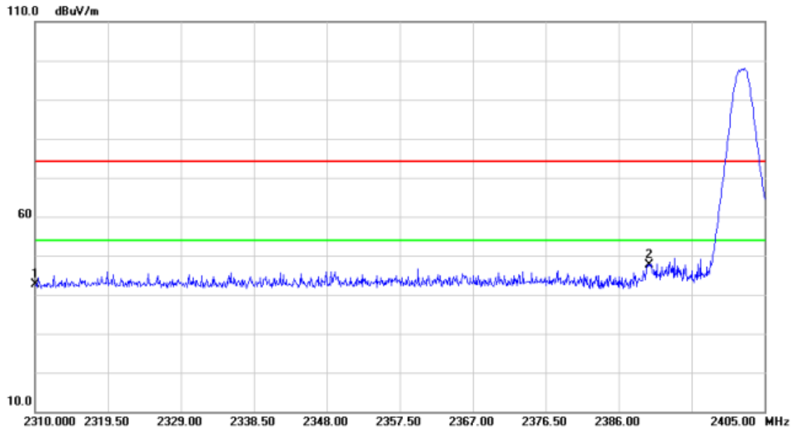
Radiated Emission
