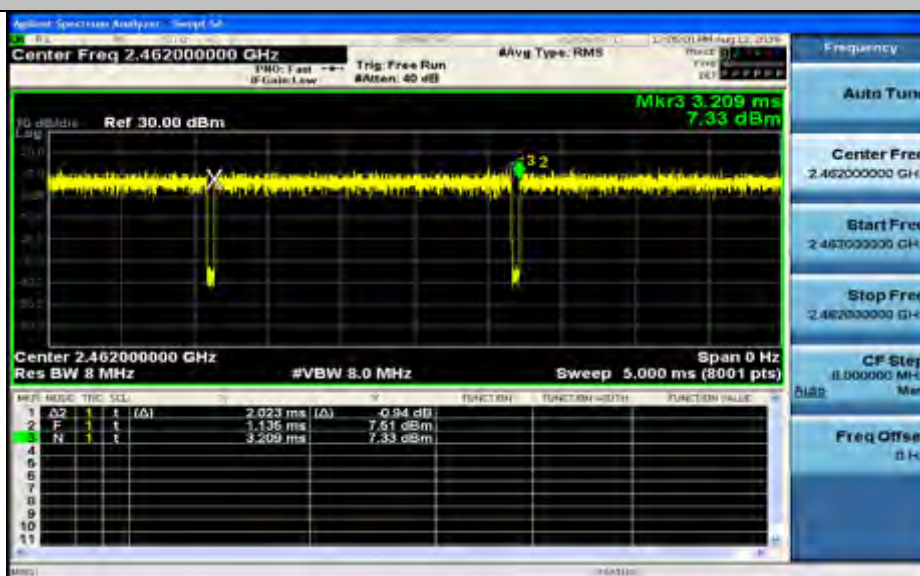
Duty Cycle_11G_2462_Ant1
