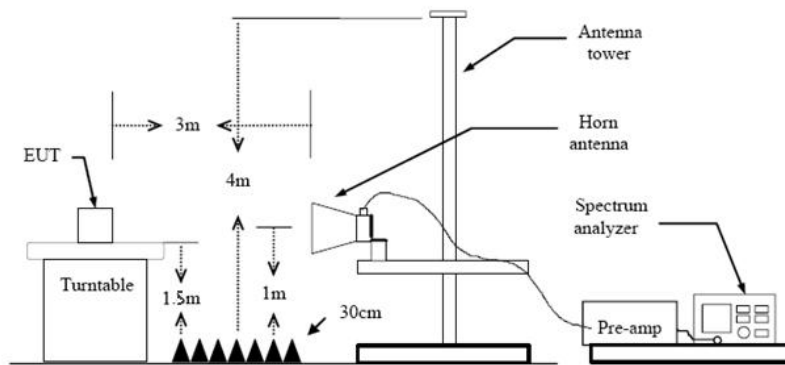
Above 1GHz Test Setup
