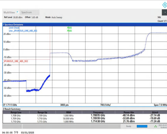
Band4_5MHz_QPSK_19975_1RB#24
