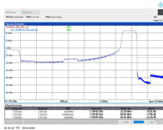
Band4_10MHz_QPSK_20350_1RB#49
