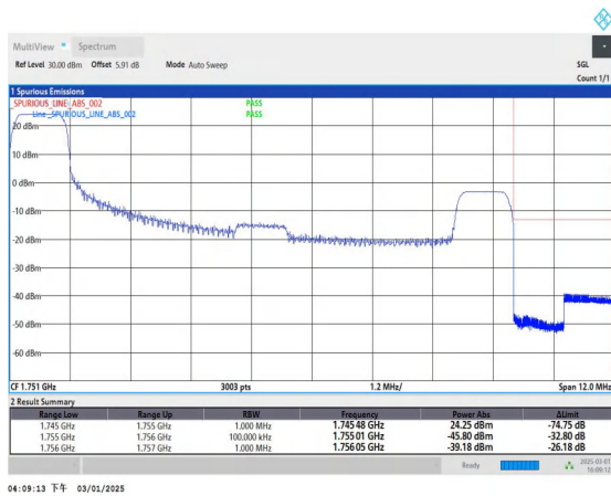
Band4_10MHz_QPSK_20350_1RB#0
