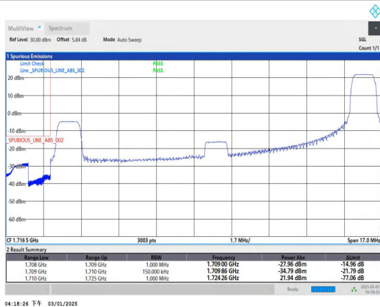
Band4_15MHz_QPSK_20025_1RB#74
