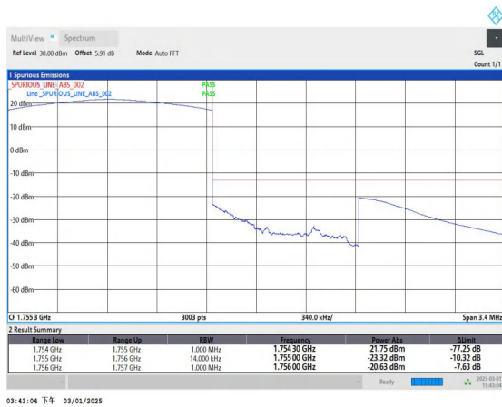
Band4_1.4MHz_QPSK_20393_6RB#0
