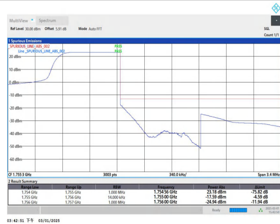
Band4_1.4MHz_QPSK_20393_1RB#5
