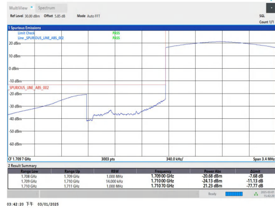
Band4_1.4MHz_QPSK_19957_6RB#0
