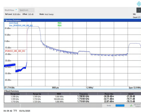
Band4_10MHz_QPSK_20000_1RB#0
