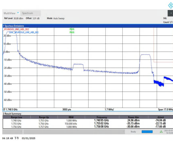
Band4_15MHz_QPSK_20325_1RB#0
