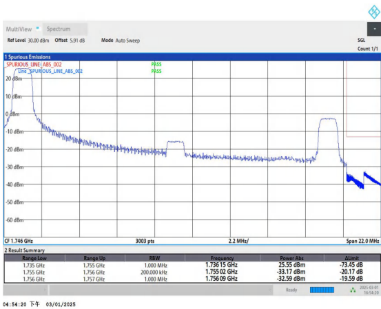
Band4_20MHz_QPSK_20300_1RB#0
