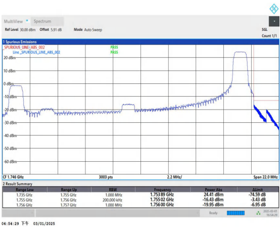
Band4_20MHz_QPSK_20300_1RB#99
