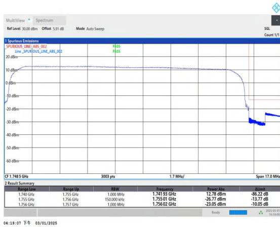
Band4_15MHz_QPSK_20325_75RB#0
