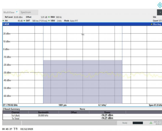
Band4_3MHz_QPSK_20385_1RB#14_Final1
