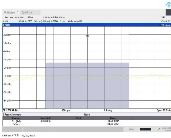
Band4_3MHz_QPSK_19965_1RB#0_Final1
