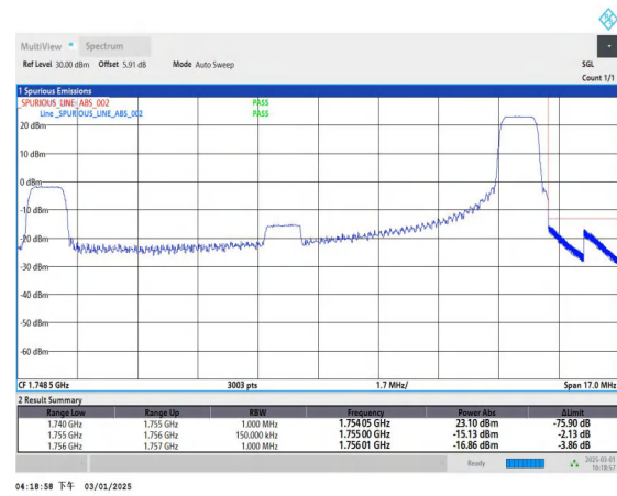
Band4_15MHz_QPSK_20325_1RB#74
