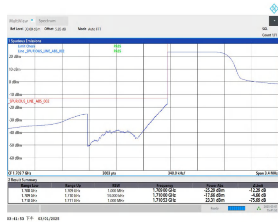
Band4_1.4MHz_QPSK_19957_1RB#0
