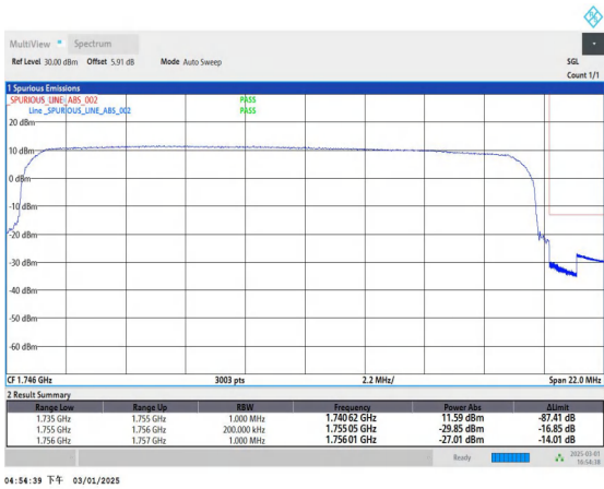
Band4_20MHz_QPSK_20300_100RB#0
