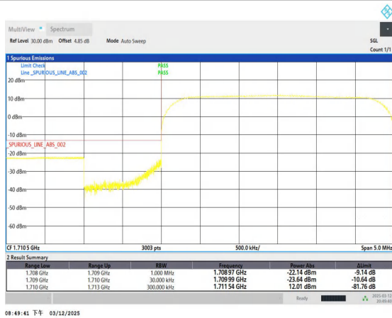
Band4_3MHz_QPSK_19965_15RB#0
