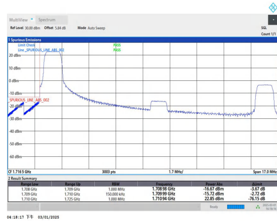
Band4_15MHz_QPSK_20025_1RB#0
