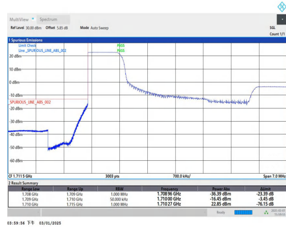
Band4_5MHz_QPSK_19975_1RB#0
