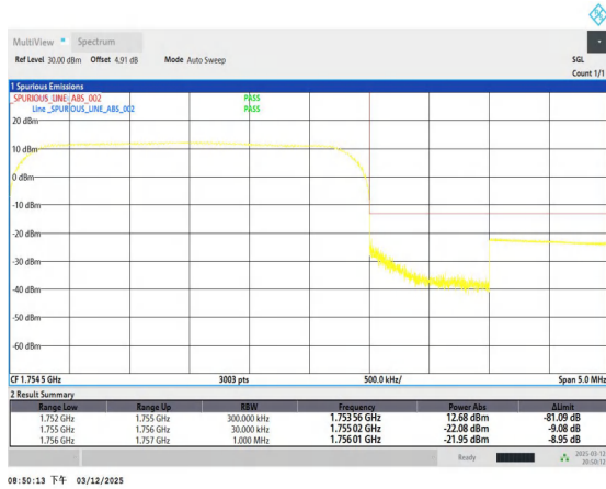
Band4_3MHz_QPSK_20385_15RB#0
