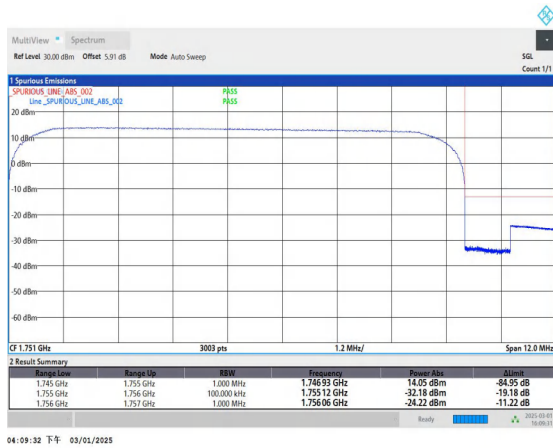
Band4_10MHz_QPSK_20350_50RB#0
