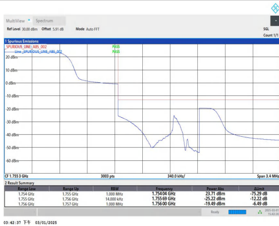
Band4_1.4MHz_QPSK_20393_1RB#0
