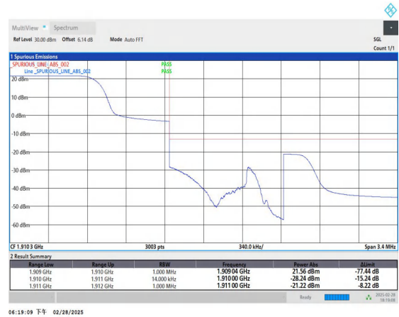
Band2_1.4MHz_QPSK_19193_1RB#0
