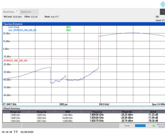
Band2_1.4MHz_QPSK_18607_6RB#0
