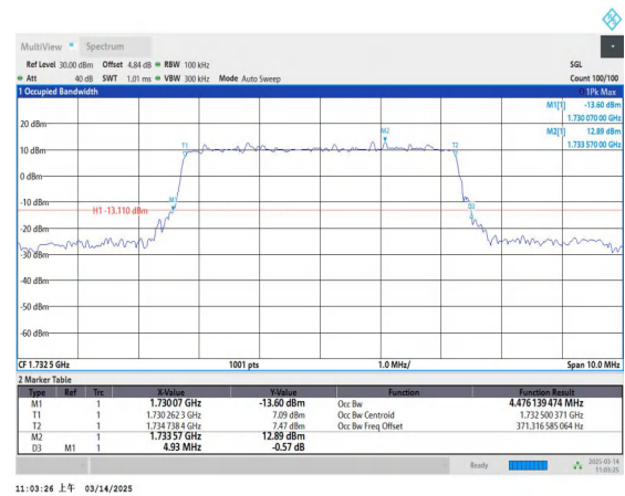
Band4-5MHz-16QAM-20175-25RB#0-PASS
