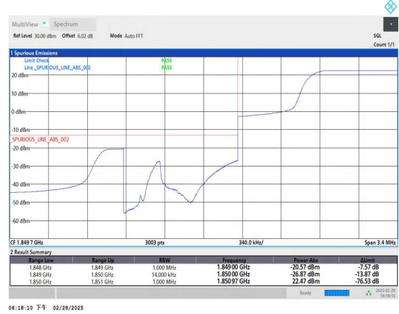
Band2_1.4MHz_QPSK_18607_1RB#5
