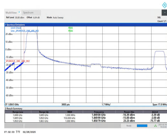
Band2_15MHz_QPSK_18675_1RB#0
