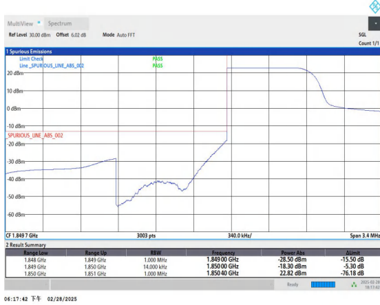
Band2_1.4MHz_QPSK_18607_1RB#0
