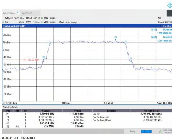
Band4-5MHz-16QAM-19975-25RB#0-PASS
