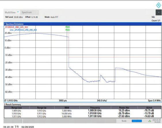
Band2_1.4MHz_QPSK_19193_6RB#0
