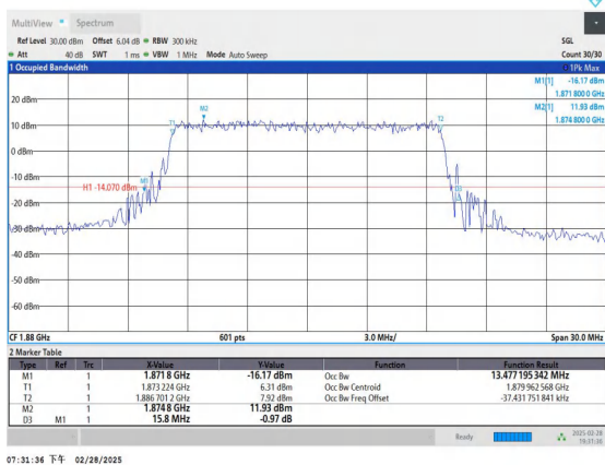
Band2-15MHz-QPSK-18675-75RB#0-PASS
