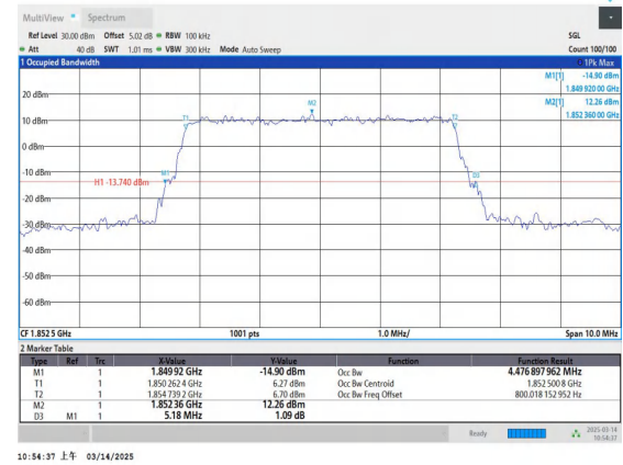
Band2-5MHz-16QAM-18625-25RB#0-PASS
