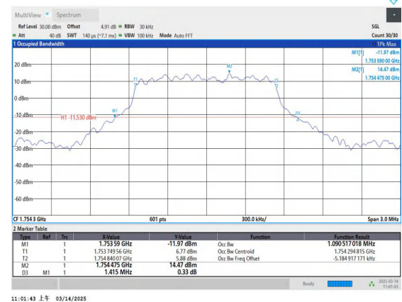
Band4-1.4MHz-QPSK-20393-6RB#0-PASS
