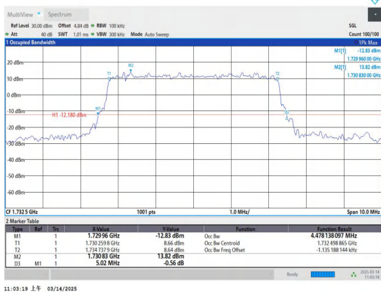
Band4-5MHz-QPSK-20175-25RB#0-PASS
