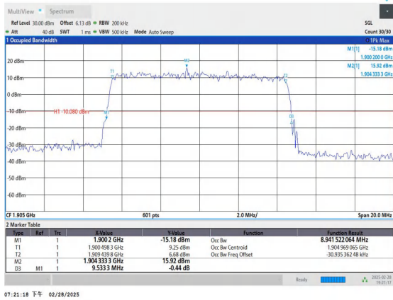
Band2-10MHz-QPSK-19150-50RB#0-PASS
