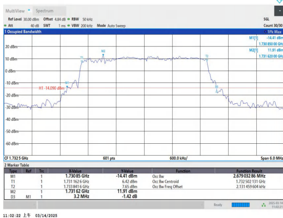
Band4-3MHz-QPSK-20175-15RB#0-PASS
