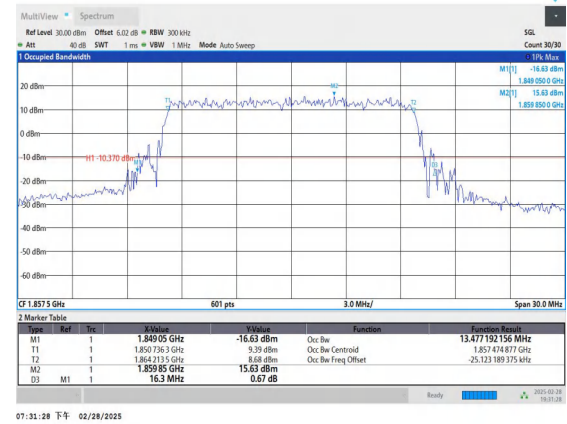
Band2-15MHz-QPSK-18675-75RB#0-PASS
