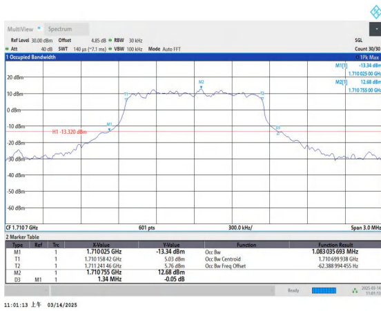
Band4-1.4MHz-16QAM-19957-6RB#0-PASS
