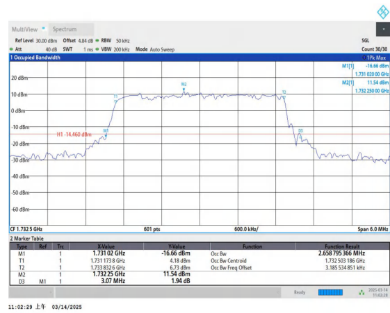
Band4-3MHz-16QAM-20175-15RB#0-PASS
