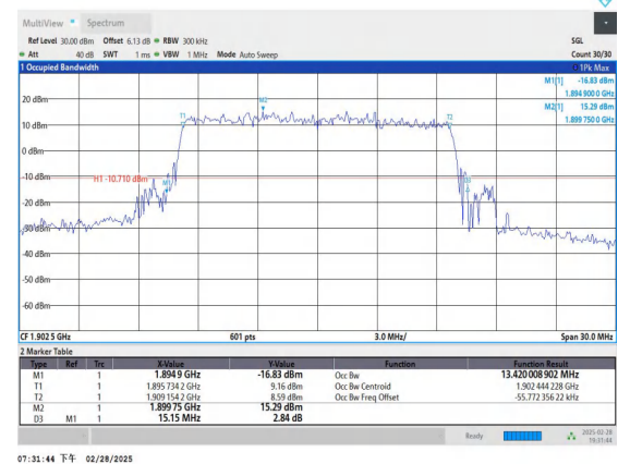
Band2-15MHz-QPSK-19125-75RB#0-PASS
