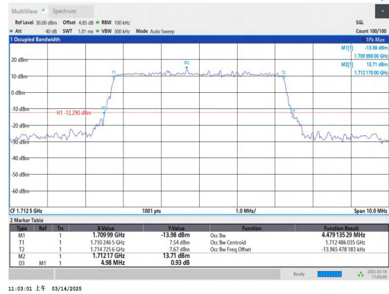
Band4-5MHz-QPSK-19975-25RB#0-PASS
