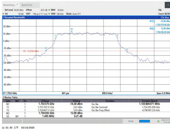
Band4-1.4MHz-16QAM-20393-6RB#0-PASS
