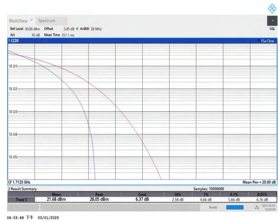
Band4-5MHz-QPSK-19975-25RB#0-PASS
