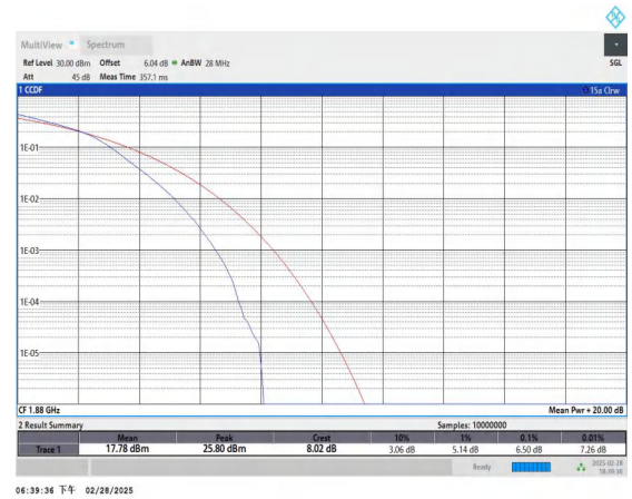
Band2-3MHz-16QAM-18900-15RB#0-PASS
