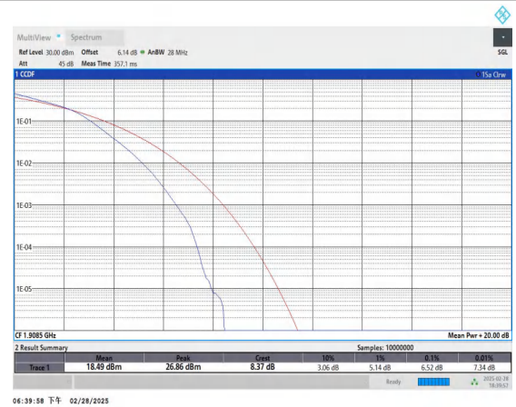
Band2-3MHz-16QAM-19185-15RB#0-PASS
