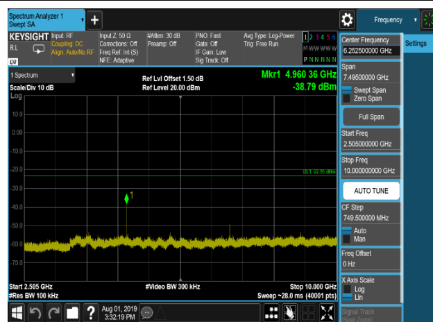
GFSK,2480MHz,DH5,Plot 3,2505MHz~10000 MHz
