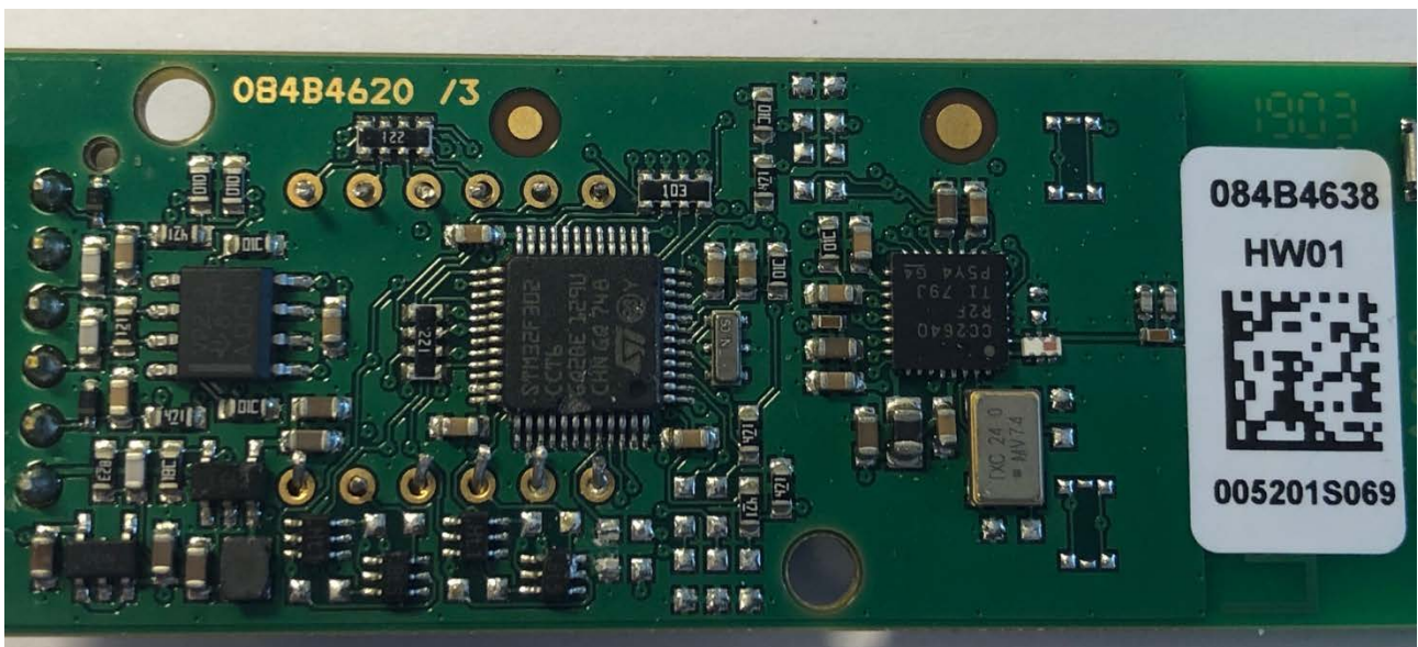
Picture of a PCBA without display.
