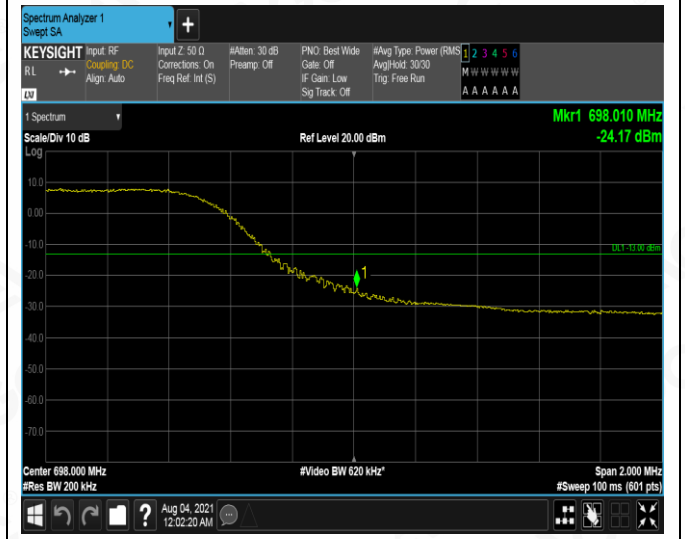
HCH_16QAM_50RB#0
