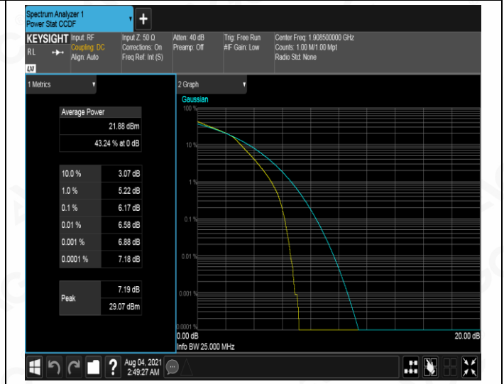
HCH_16QAM_15RB#0
