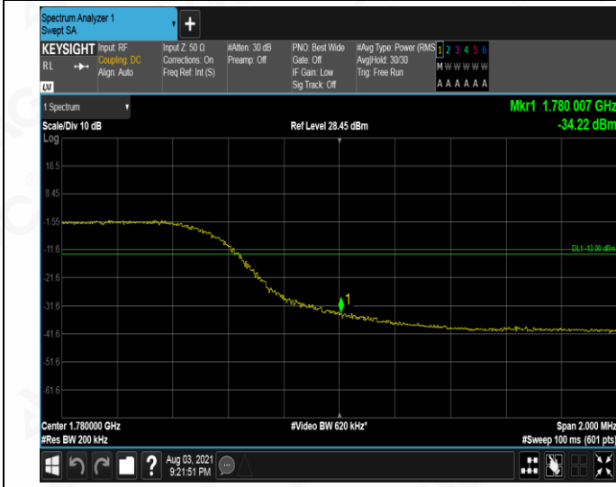
HCH_QPSK_50RB#0
