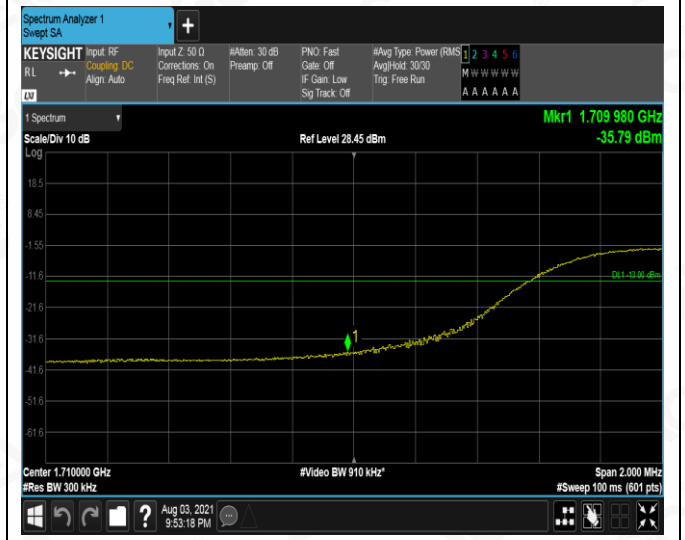
LCH_16QAM_75RB#0
