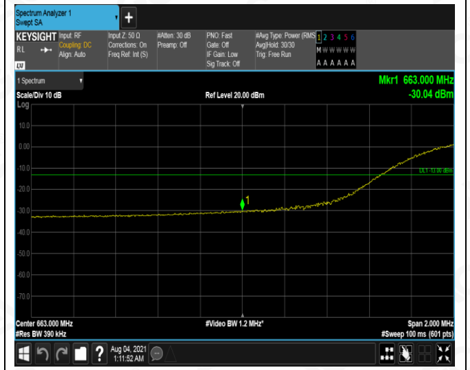
LCH_16QAM_100RB#0
