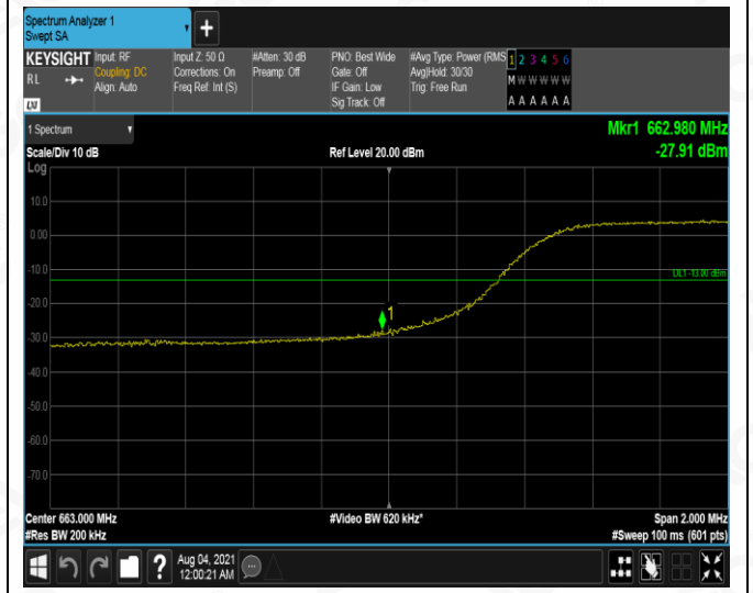
LCH_16QAM_50RB#0
