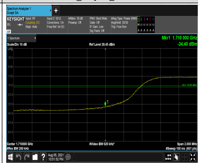
LCH_16QAM_50RB#0
