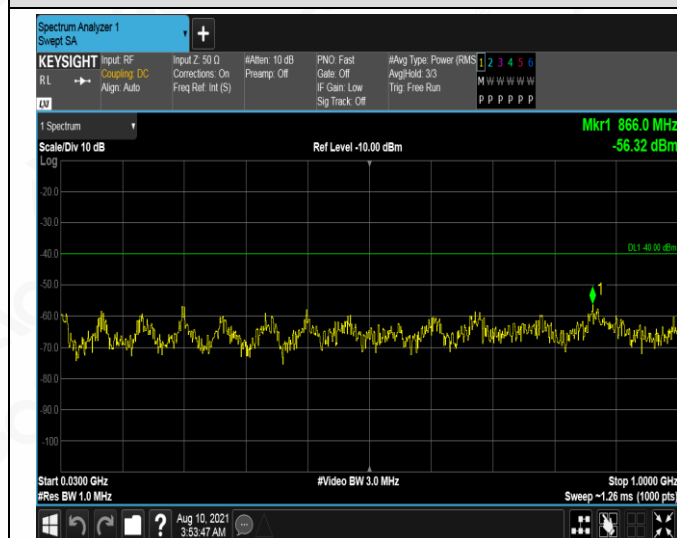
5MHz_HCH_QPSK_1RB#0_2288~2292MHz
