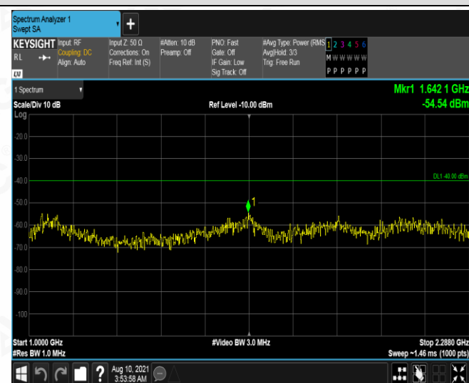
5MHz_HCH_QPSK_1RB#0_2292~2296MHz
