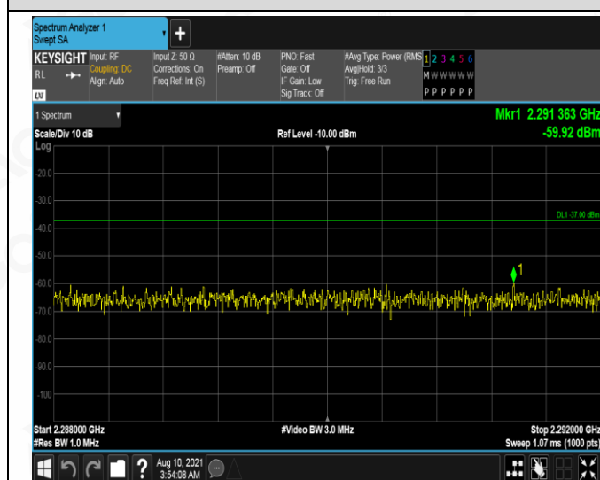
5MHz_HCH_QPSK_1RB#0_2288~2292MHz
