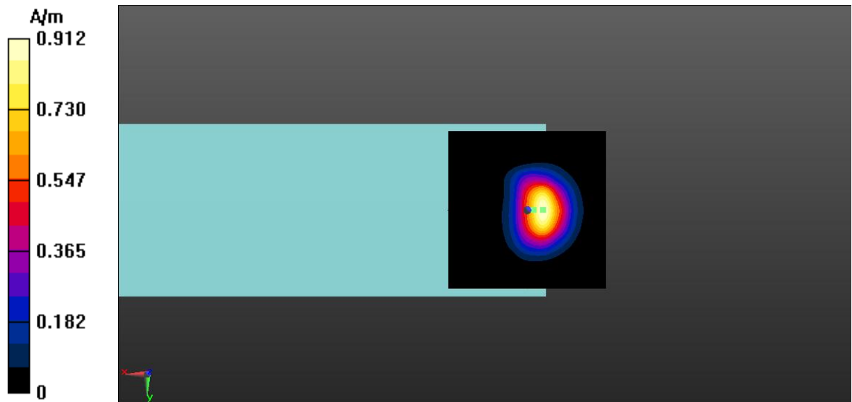
Fig A.7 T-Coil LTE-Band 4-Z
