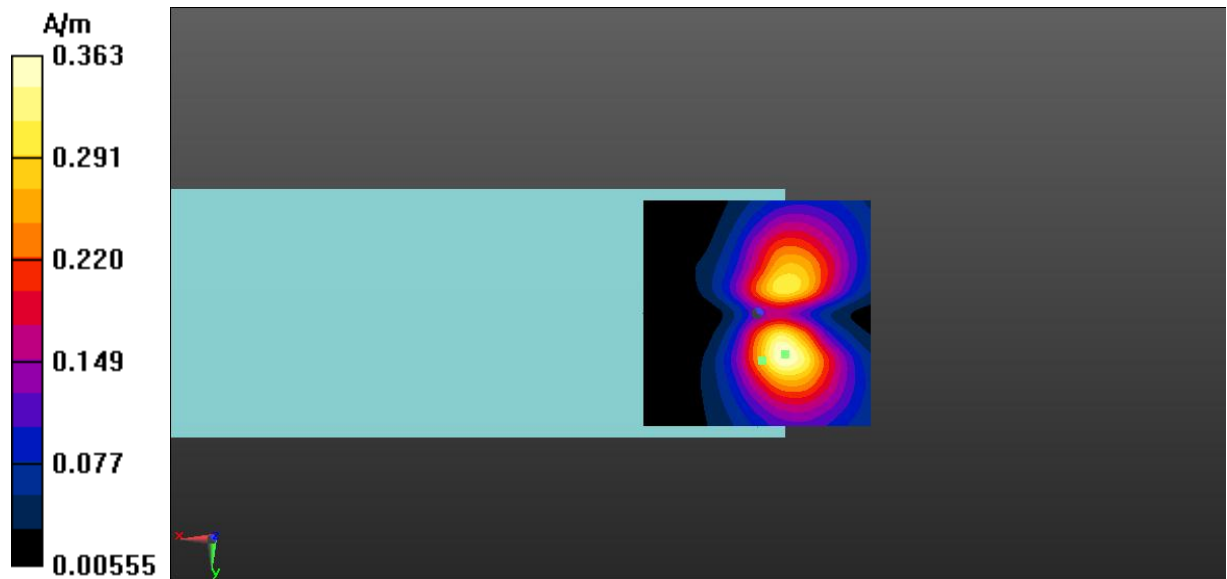
Fig A.8 T-Coil LTE-Band 5-Y
