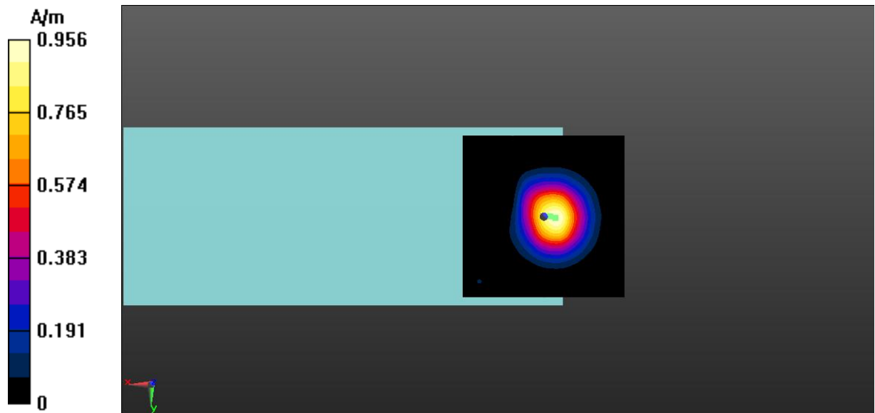
Fig A.17 T-Coil LTE-Band 38-Z
