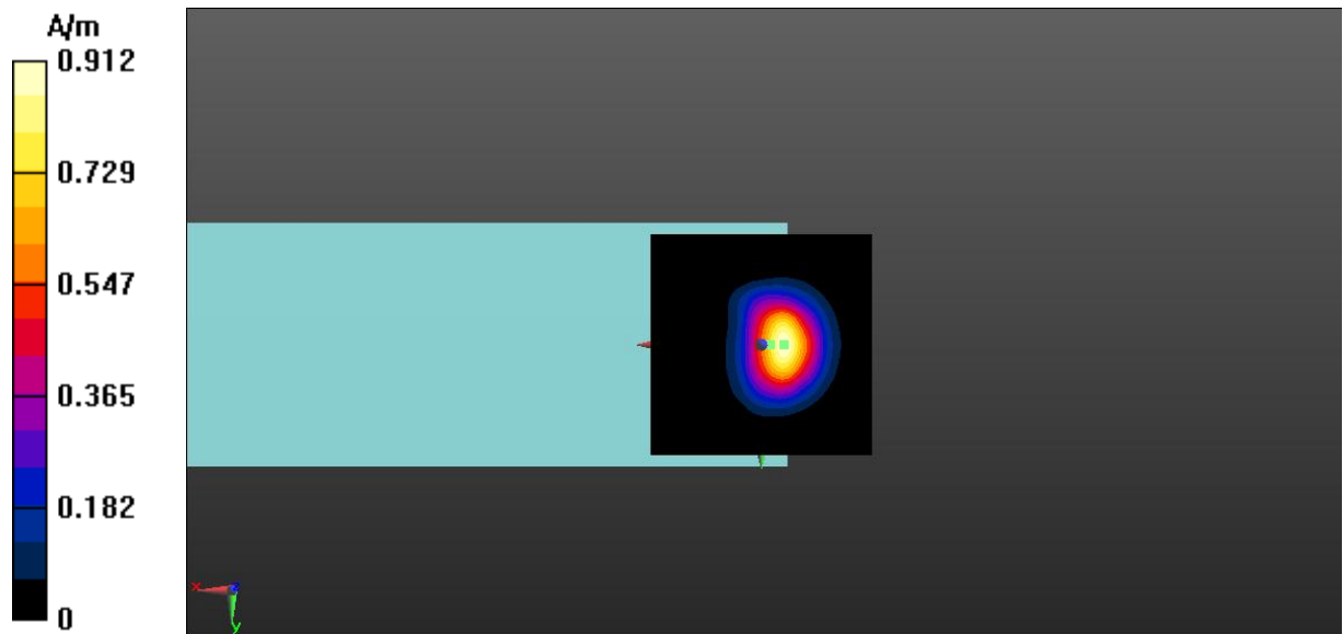
Fig A.9 T-Coil LTE-Band 7-Z
