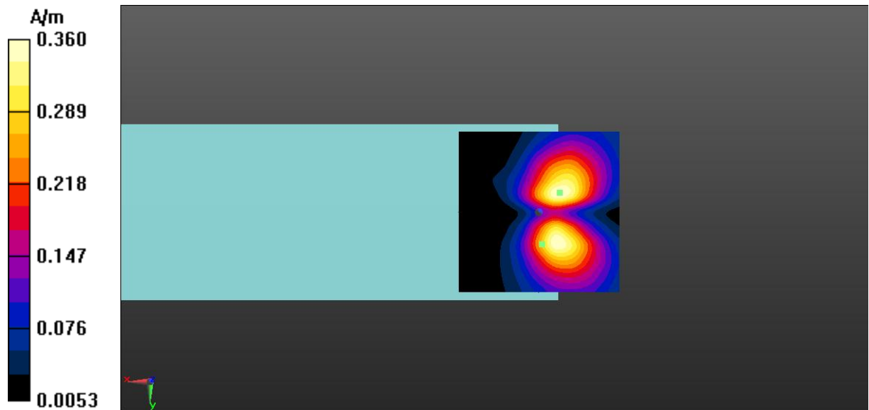
Fig A.11 T-Coil LTE-Band 13-Y
