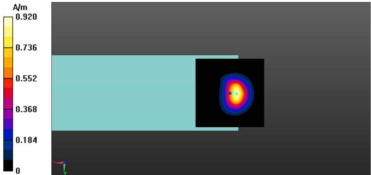
Fig A.11 T-Coil LTE-Band 13-Z
