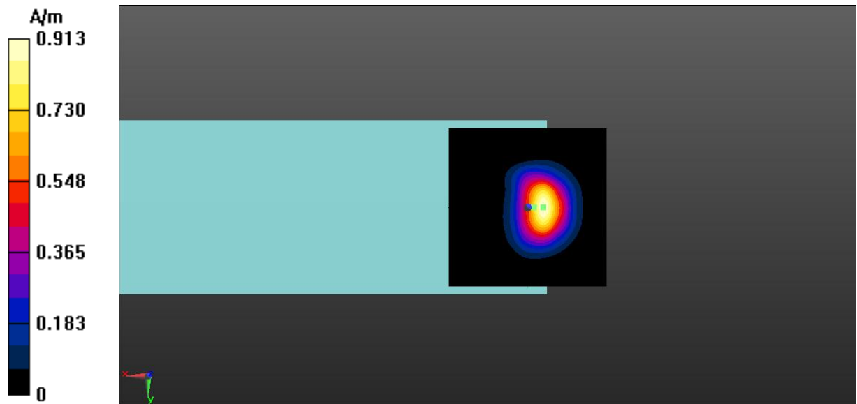
Fig A.13 T-Coil LTE-Band 25-Z
