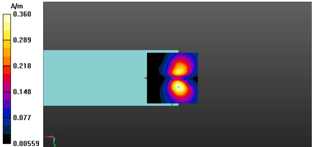
Fig A.10 T-Coil LTE-Band 12-Y
