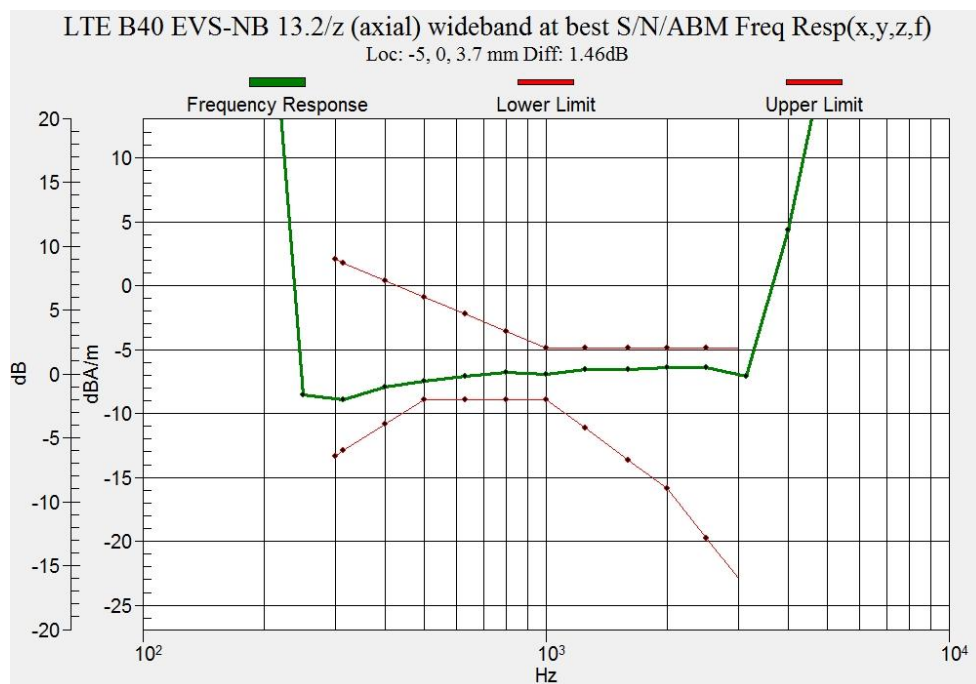
Figure B.18 Frequency Response of LTE Band 40
