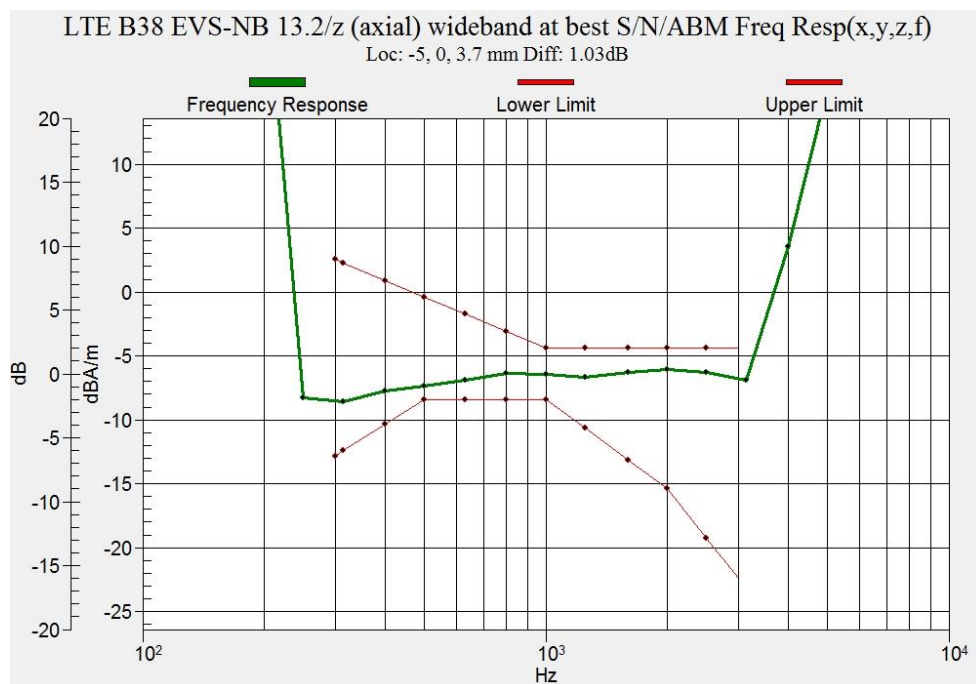
Figure B.17 Frequency Response of LTE Band 38
