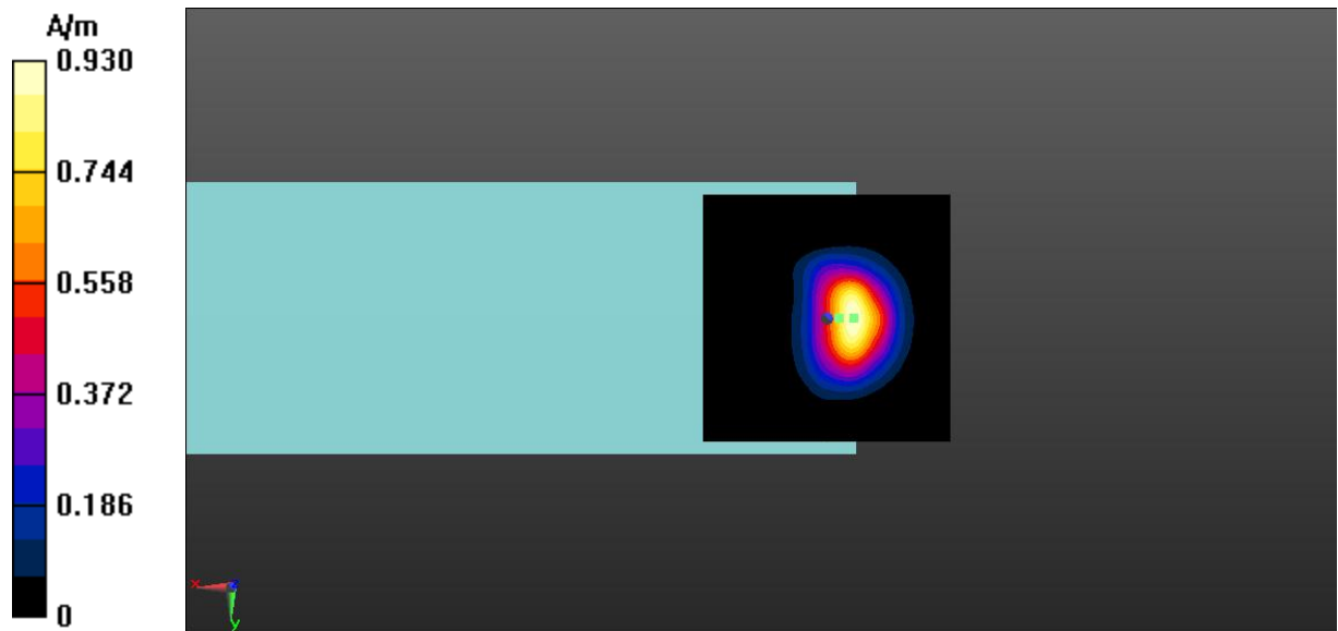
Fig A.14 T-Coil LTE-Band 26-Z
