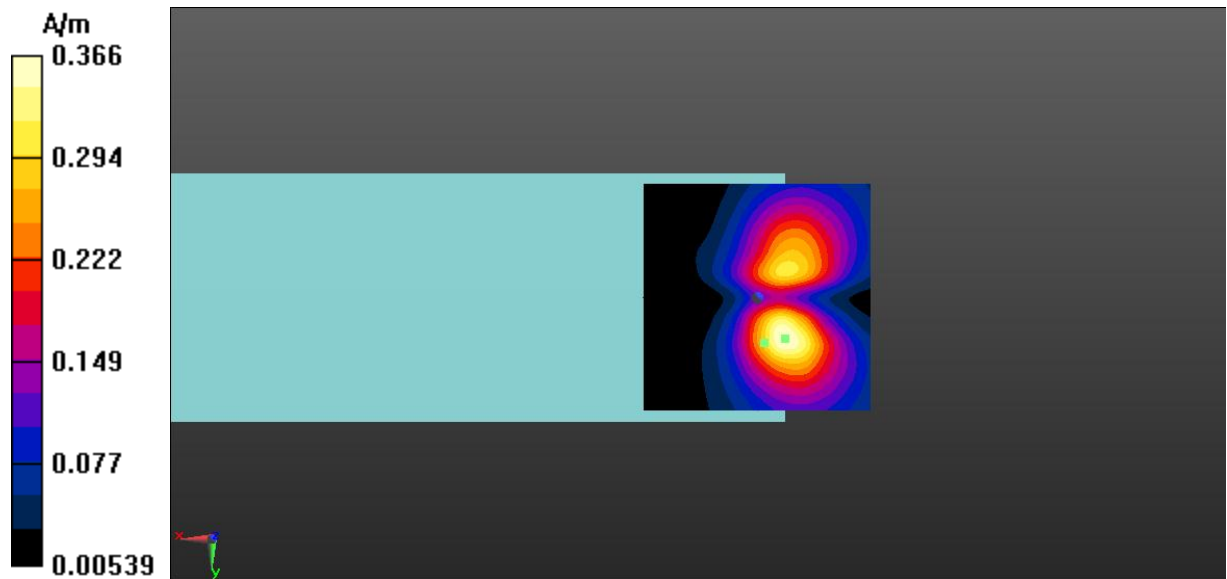
Fig A.16 T-Coil LTE-Band 71-Y
