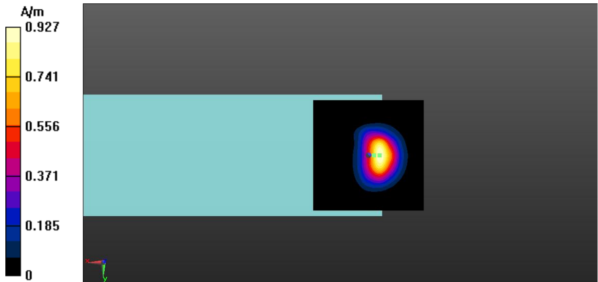
Fig A.16 T-Coil LTE-Band 71-Z
