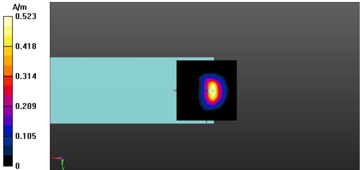
Fig A.3 T-Coil WCDMA Band 2-Z
