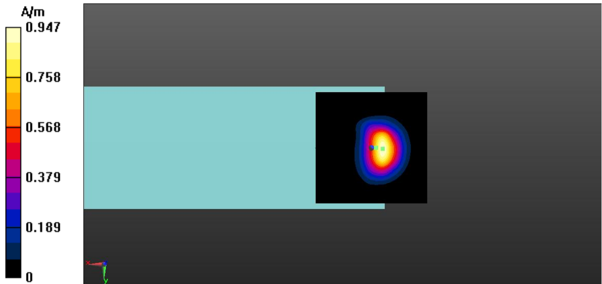
Fig A.8 T-Coil LTE-Band 5-Z
