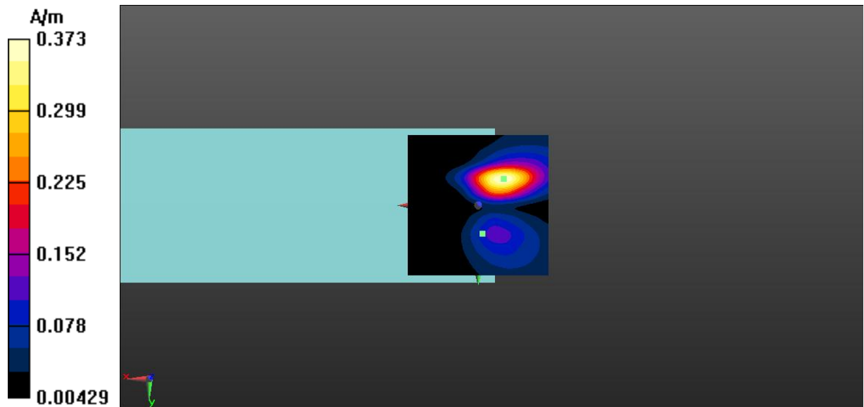
Fig A.18 T-Coil LTE-Band 40-Y
