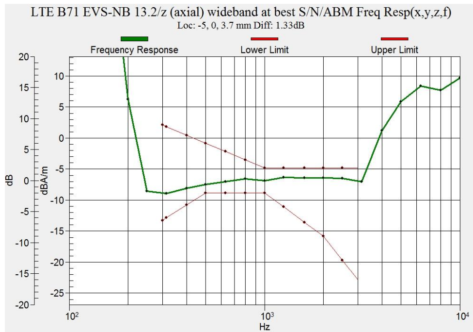
Figure B.16 Frequency Response of LTE Band 71
