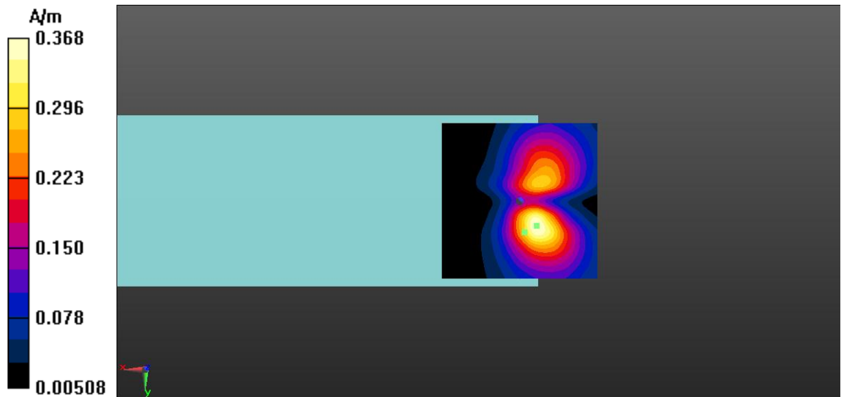
Fig A.12 T-Coil LTE-Band 17-Y
