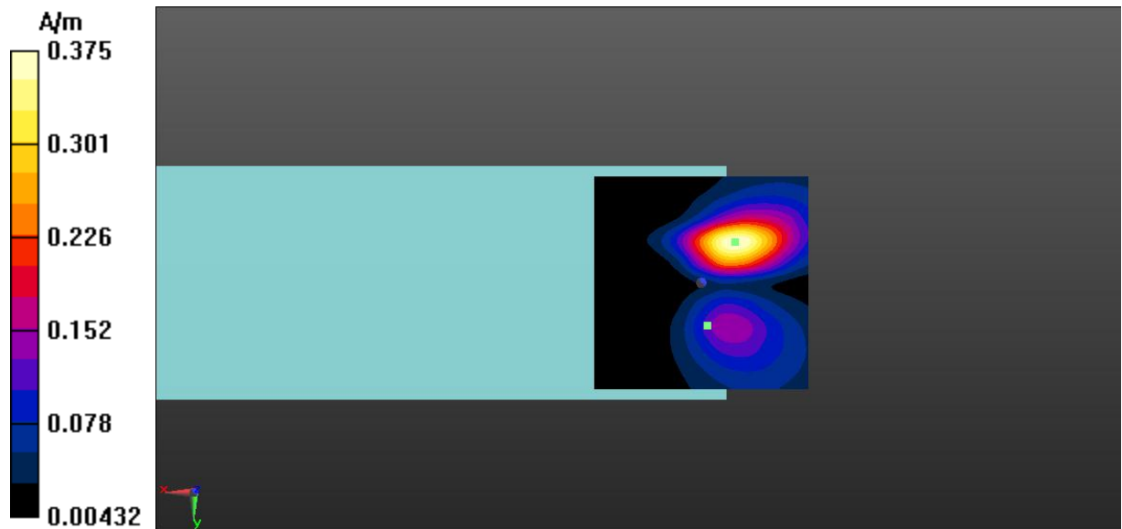
Fig A.17 T-Coil LTE-Band 38-Y
