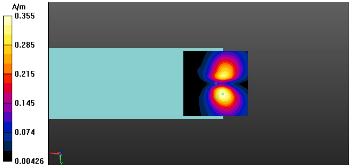
Fig A.13 T-Coil LTE-Band 25-Y
