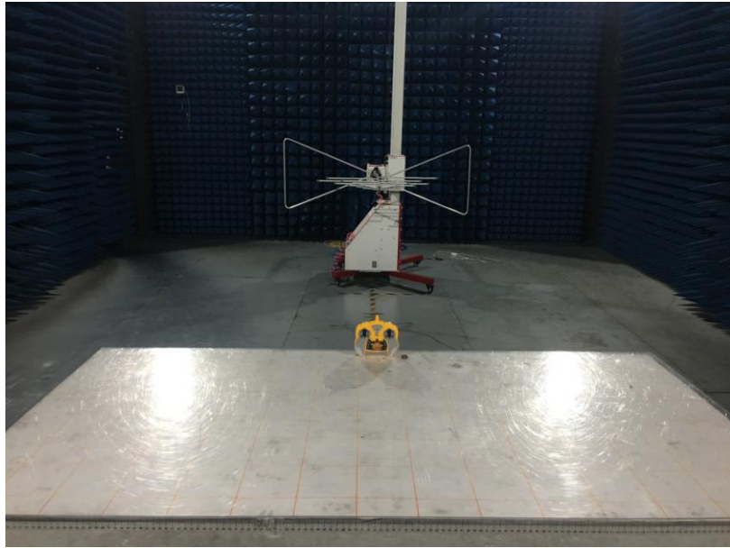
Radiated Emission for part 15C
