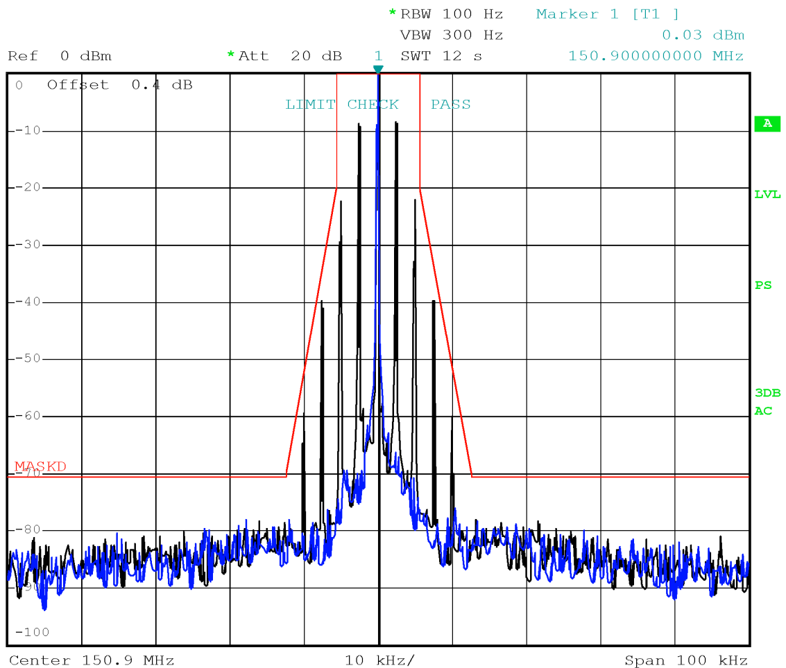
Channel LOW – FM modulation with 12.5 kHz channel bandwidth
