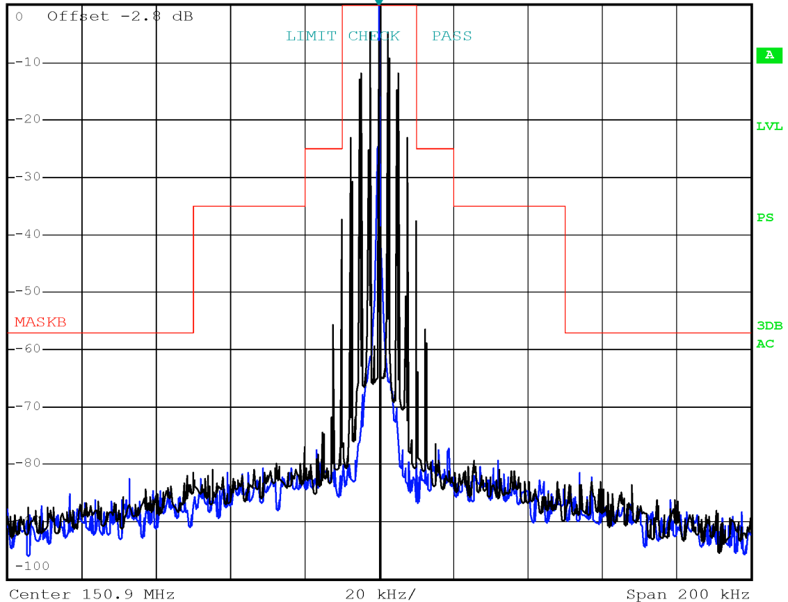
Channel LOW – FM modulation with 25 kHz channel bandwidth
