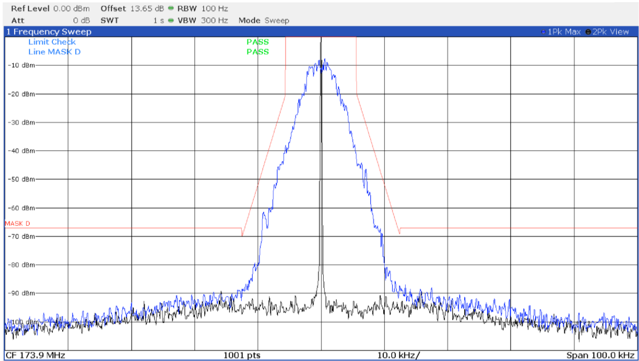
Emission mask D with modulation DMR 4FSK at 173.9 MHz
