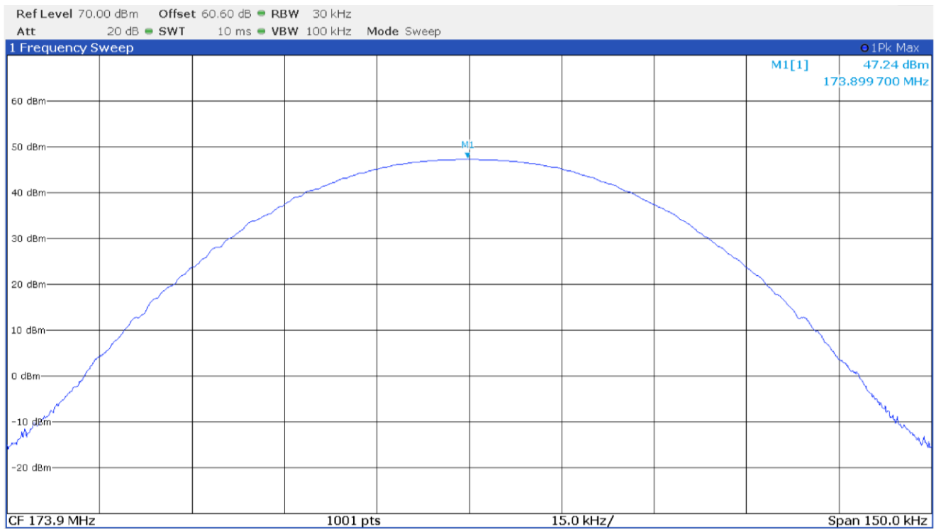
Output power with modulation P25 C4FM at 173.9 MHz
