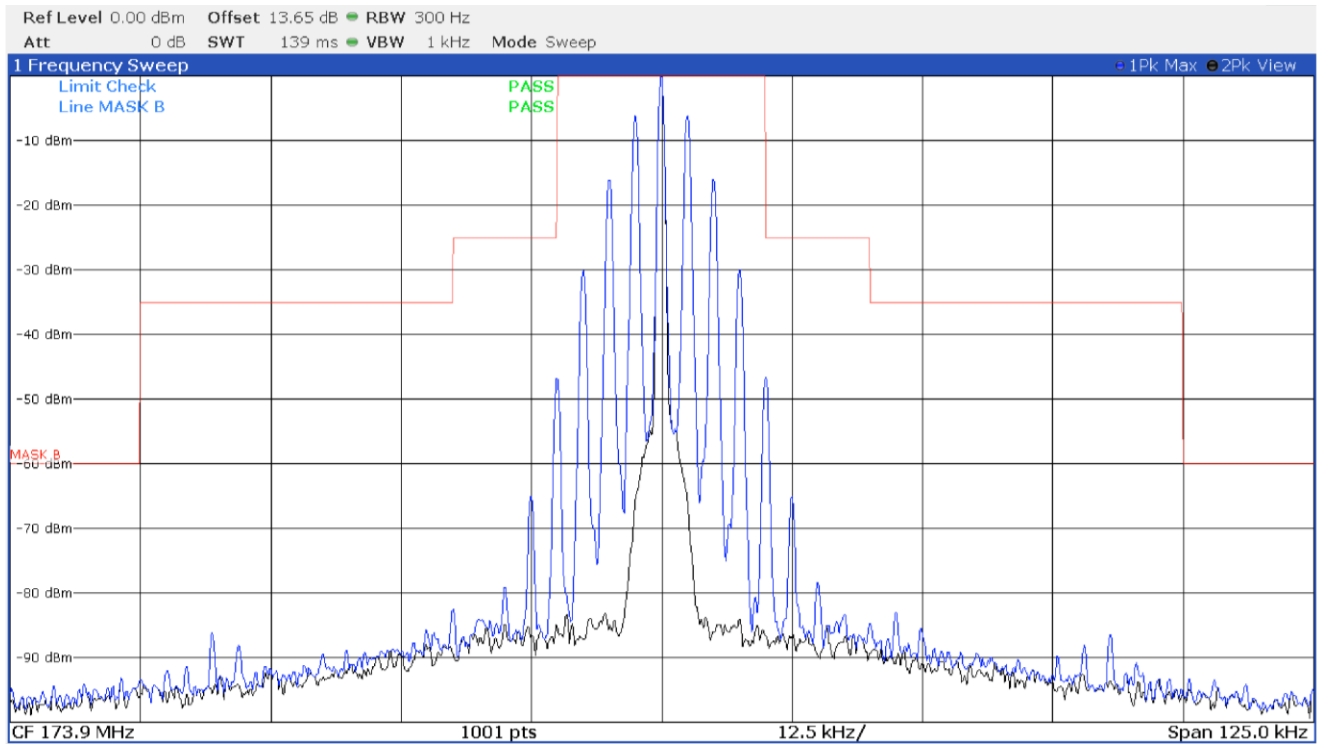
Emission mask B with modulation FM 25.0 kHz at 173.9 MHz
