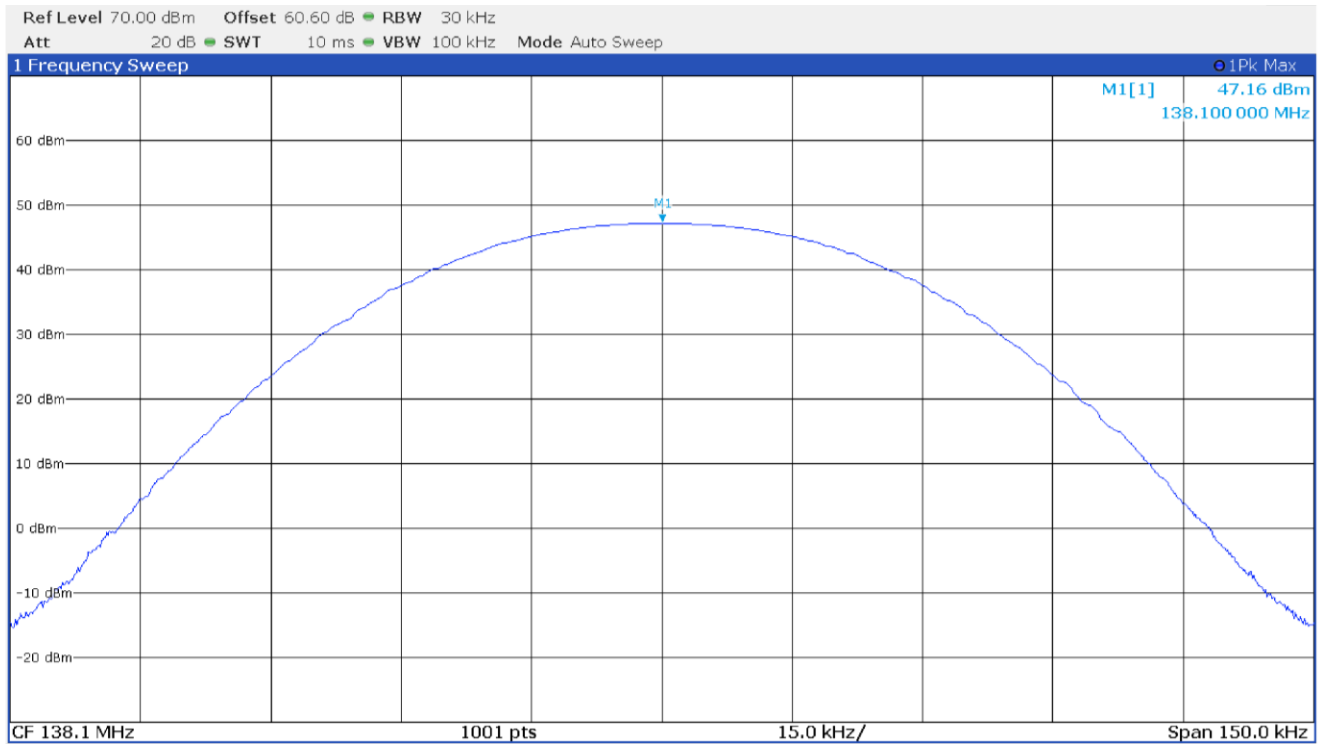
Output power with modulation P25 C4FM at 138.1 MHz
