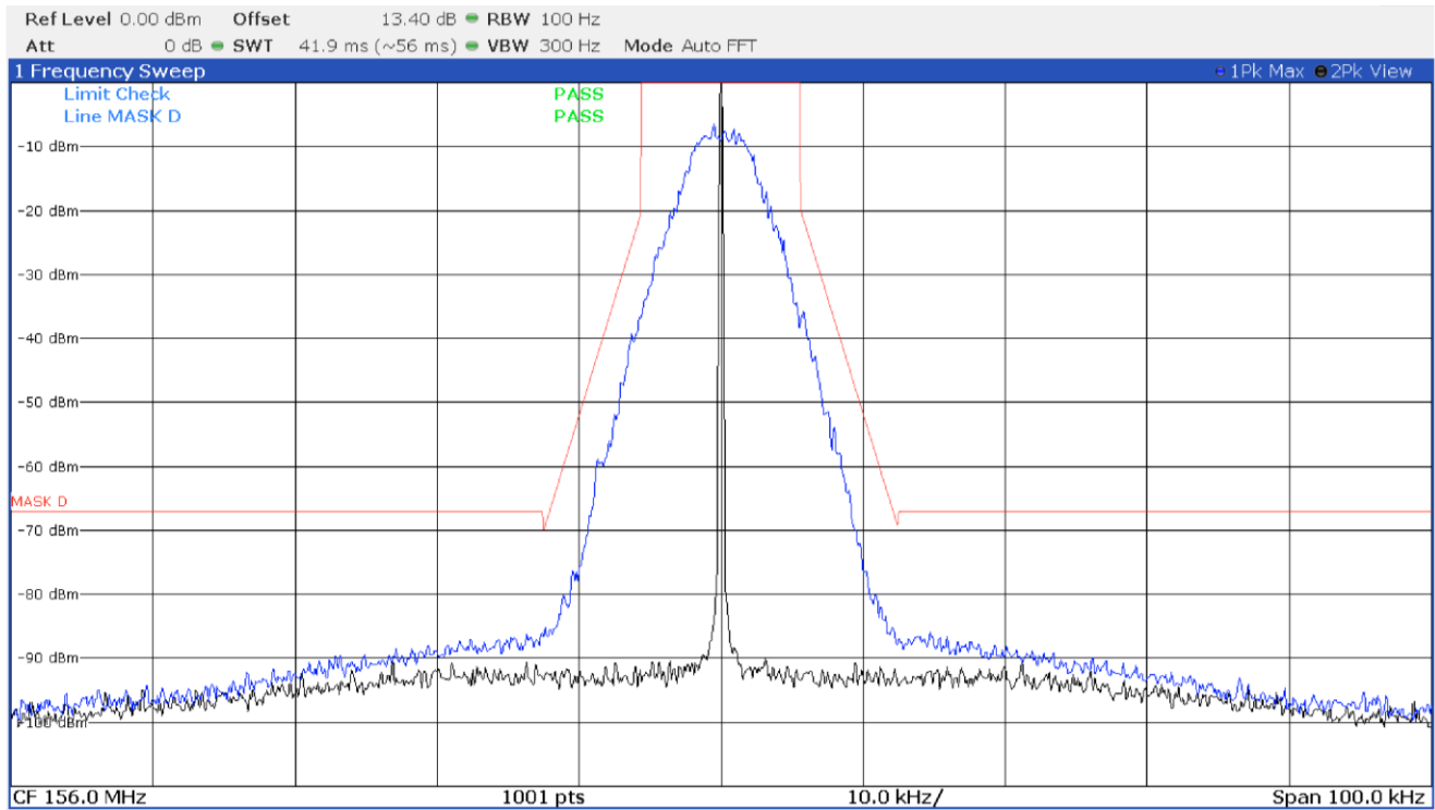
Emission mask D with modulation DMR 4FSK at 156.0 MHz
