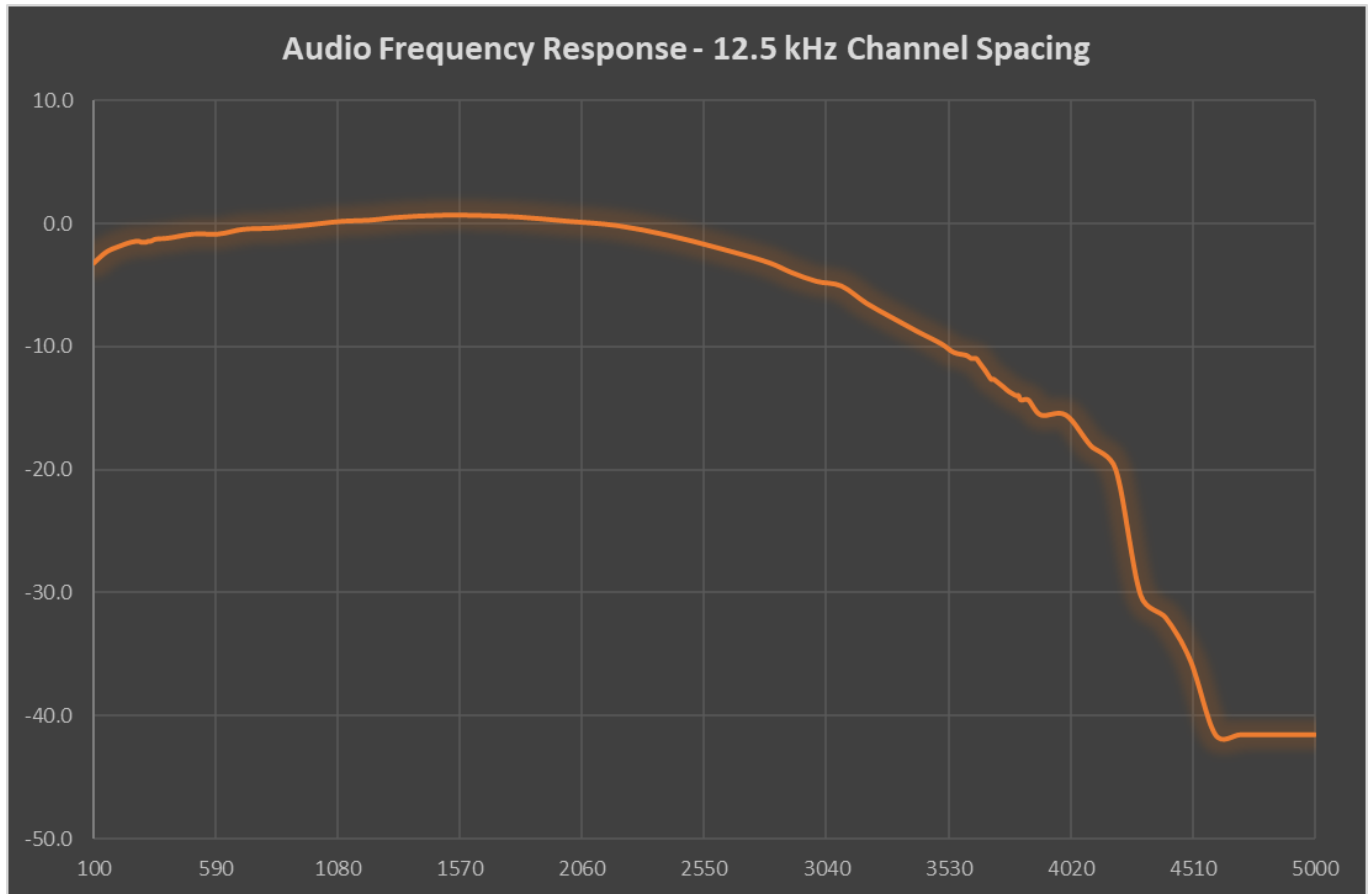
Audio frequency response
