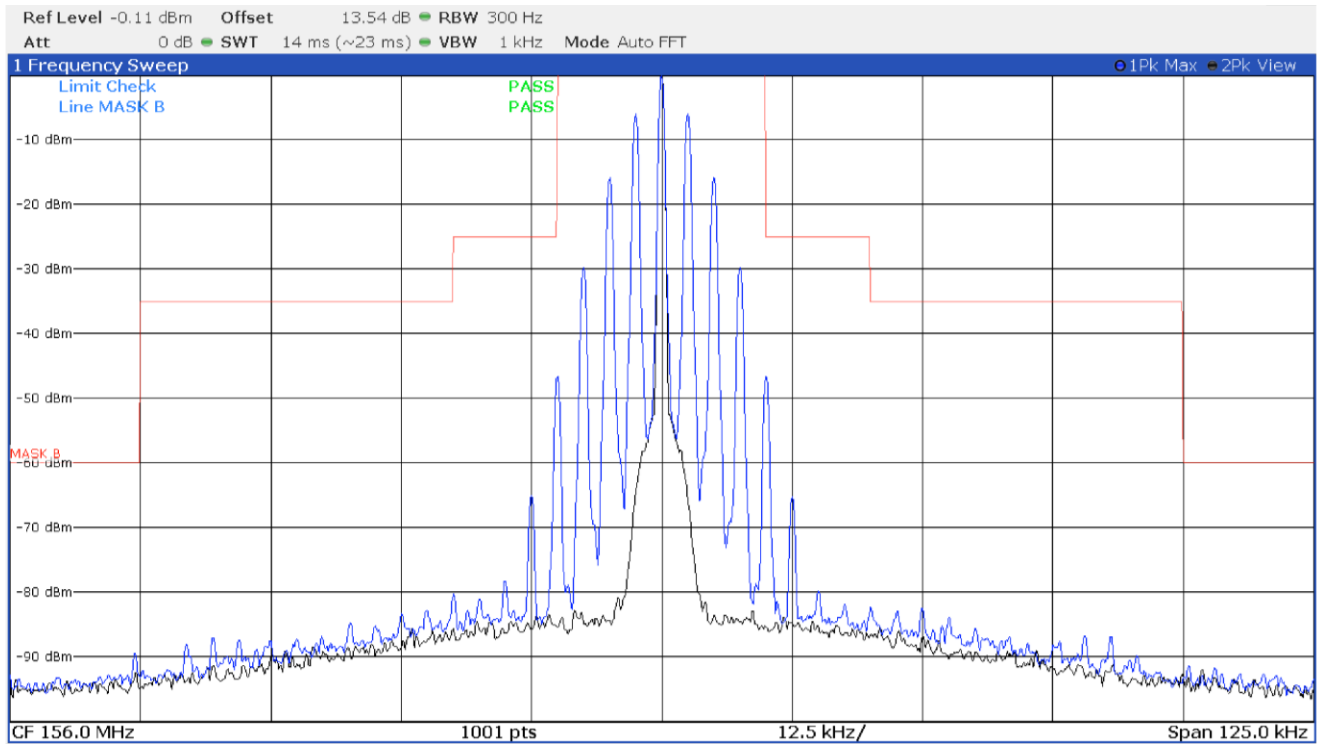
Emission mask B with modulation FM 25.0 kHz at 156.0 MHz
