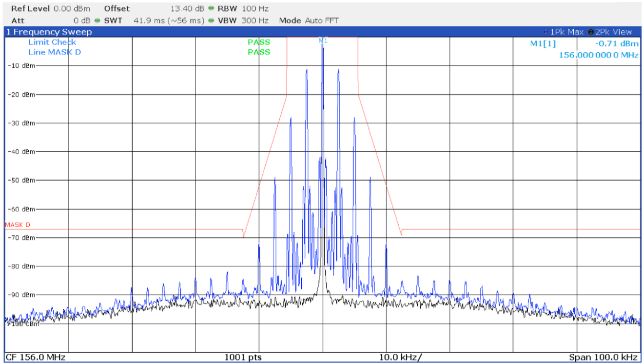
Emission mask D with modulation FM 12.5 kHz at 156.0 MHz
