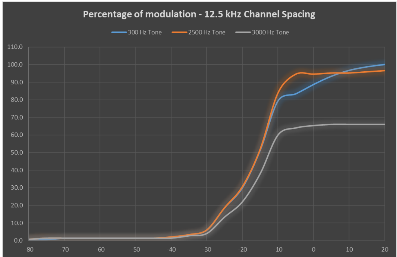
Modulation Limiting
