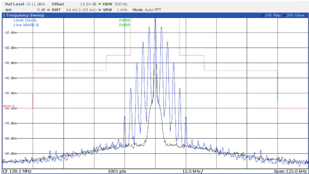
Emission mask B with modulation FM 25.0 kHz at 138.1 MHz
