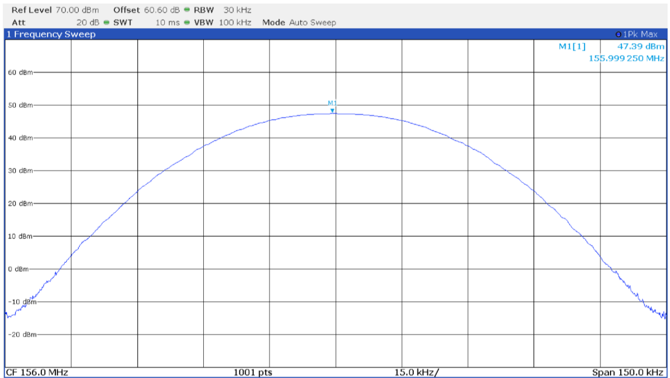
Output power with modulation DMR 4FSK at 156.0 MHz
