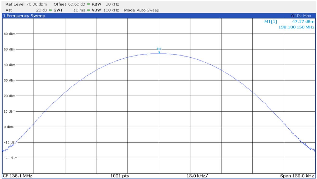
Output power with modulation CST 4FSK at 138.1 MHz
