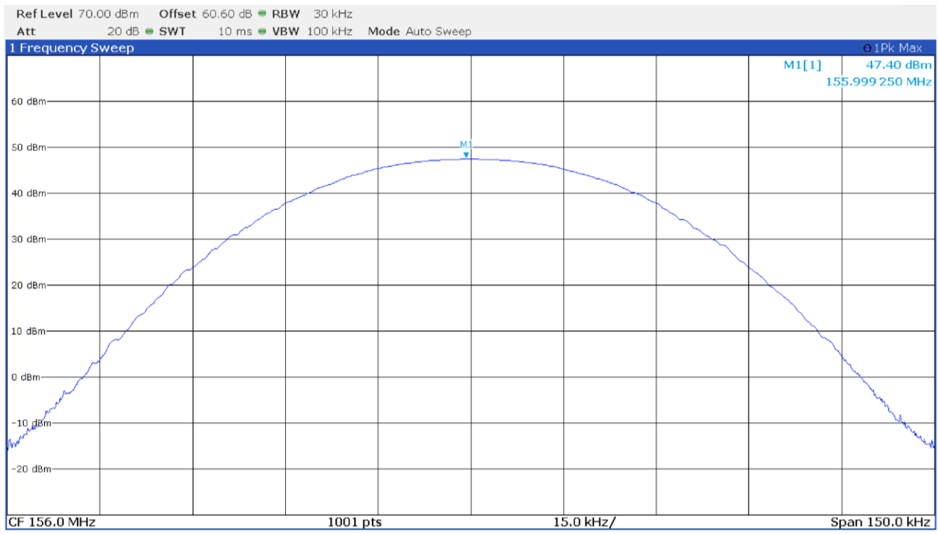
Output power with modulation P25 C4FM at 156.0 MHz
