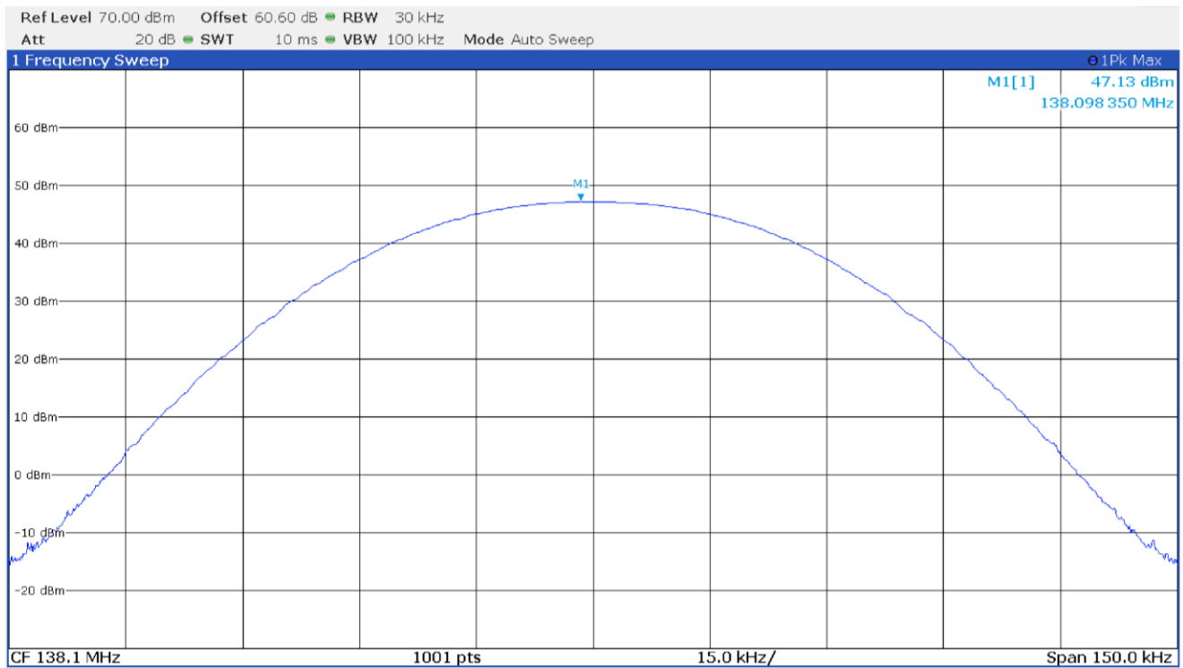
Output power with modulation DMR 4FSK at 138.1 MHz
