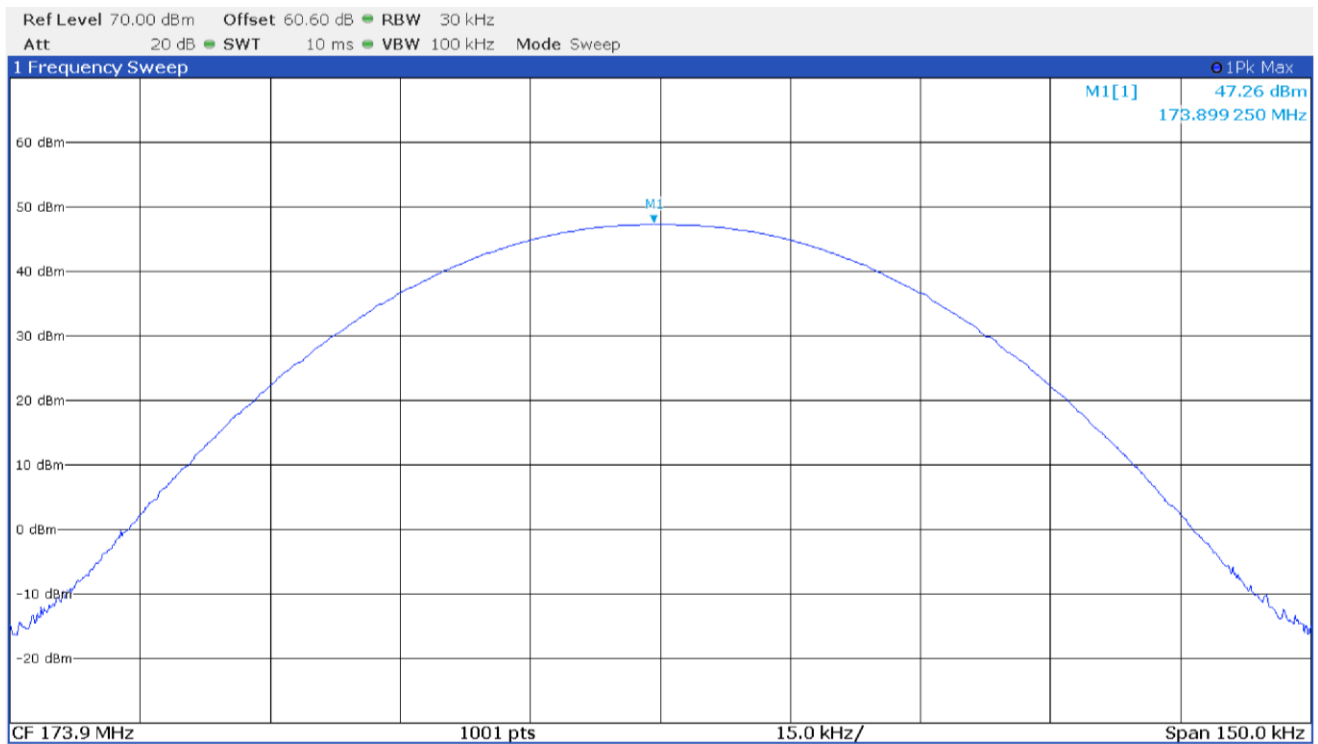
Output power with modulation CST 4FSK at 173.9 MHz
