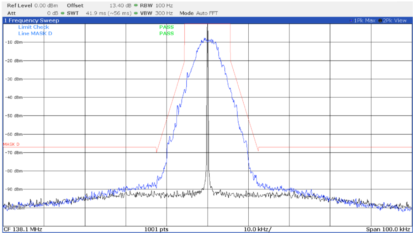
Emission mask D with modulation DMR 4FSK at 138.1 MHz
