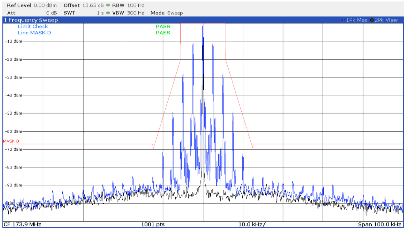
Emission mask D with modulation FM 12.5 kHz at 173.9 MHz
