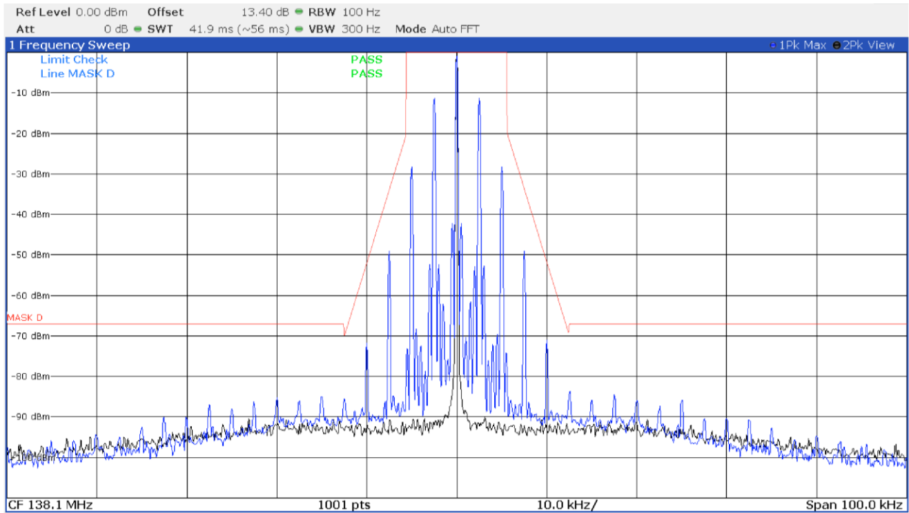
Emission mask D with modulation FM 12.5 kHz at 138.1 MHz
