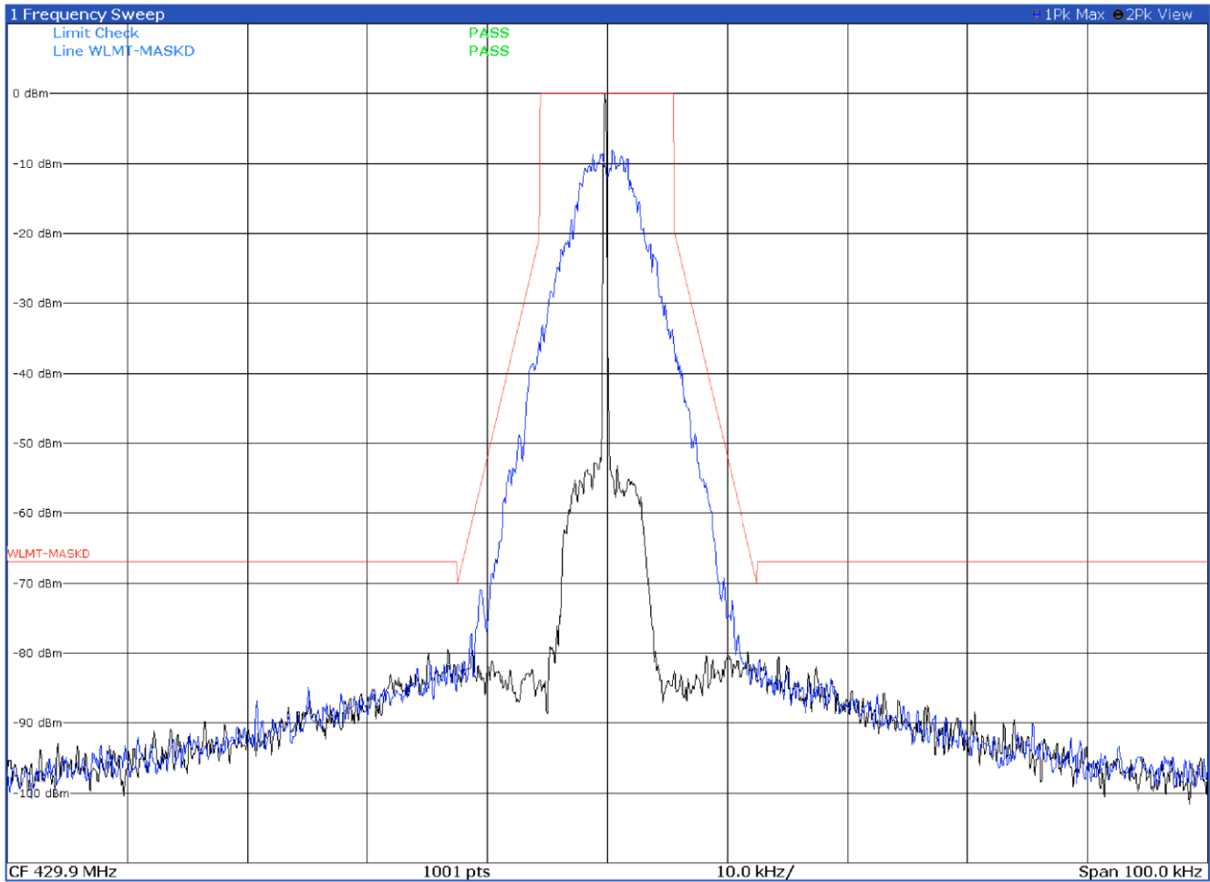
Emission mask D with modulation P25 C4FM at 429.9 MHz
