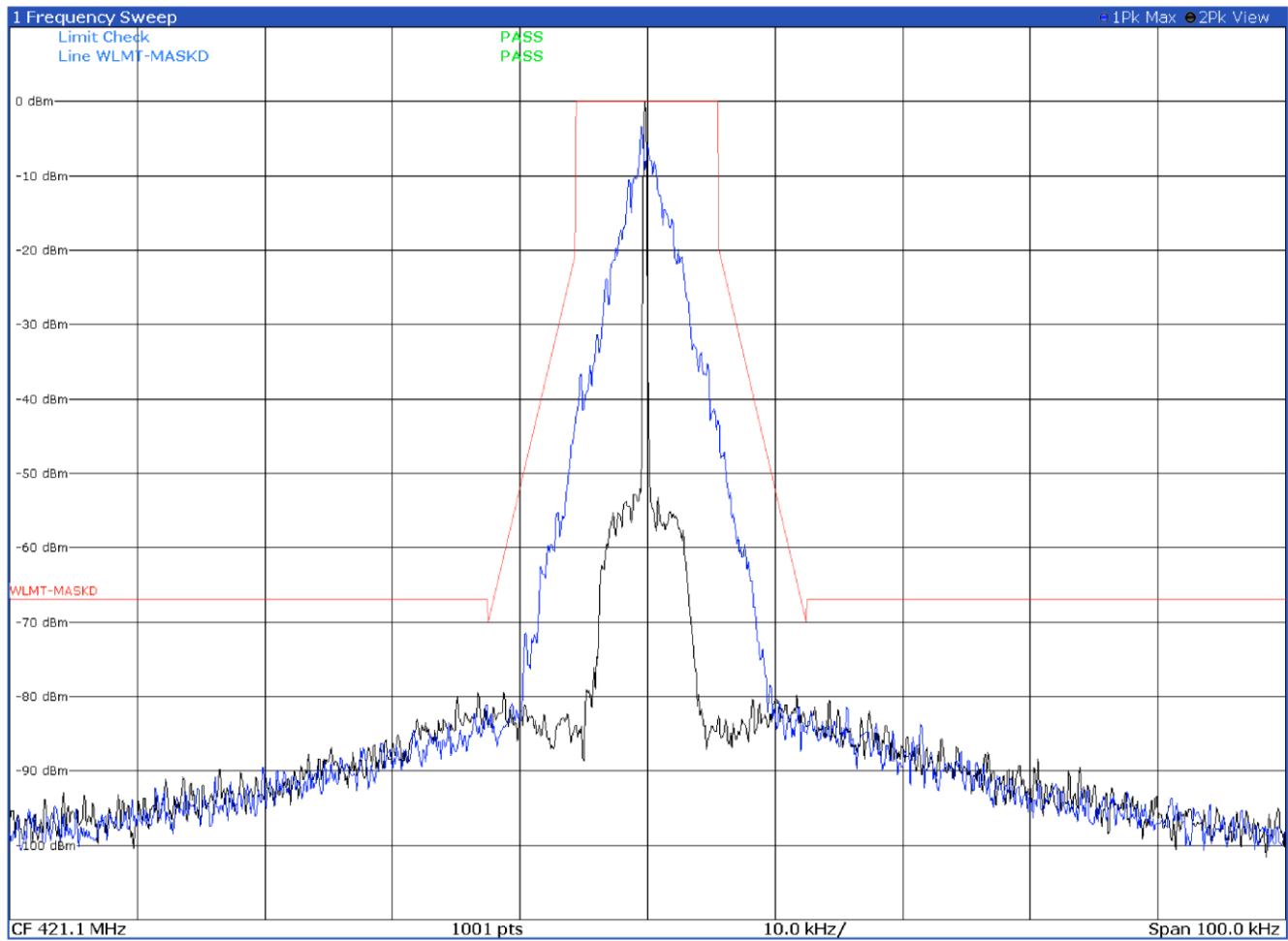
Emission mask D with modulation CST 4FSK at 421.1 MHz
