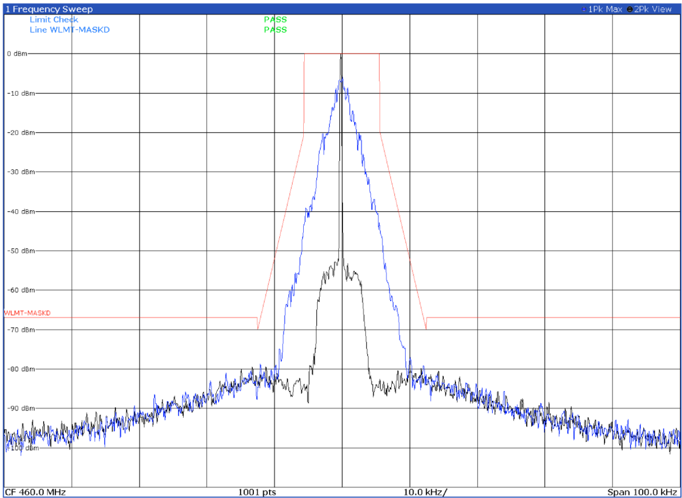
Emission mask D with modulation CST 4FSK at 460.0 MHz
