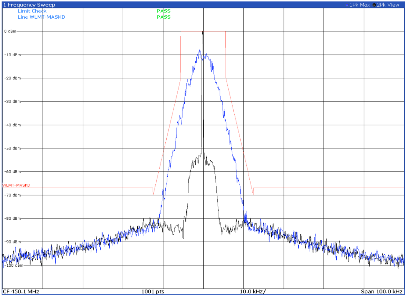
Emission mask D with modulation P25 C4FM at 450.1 MHz
