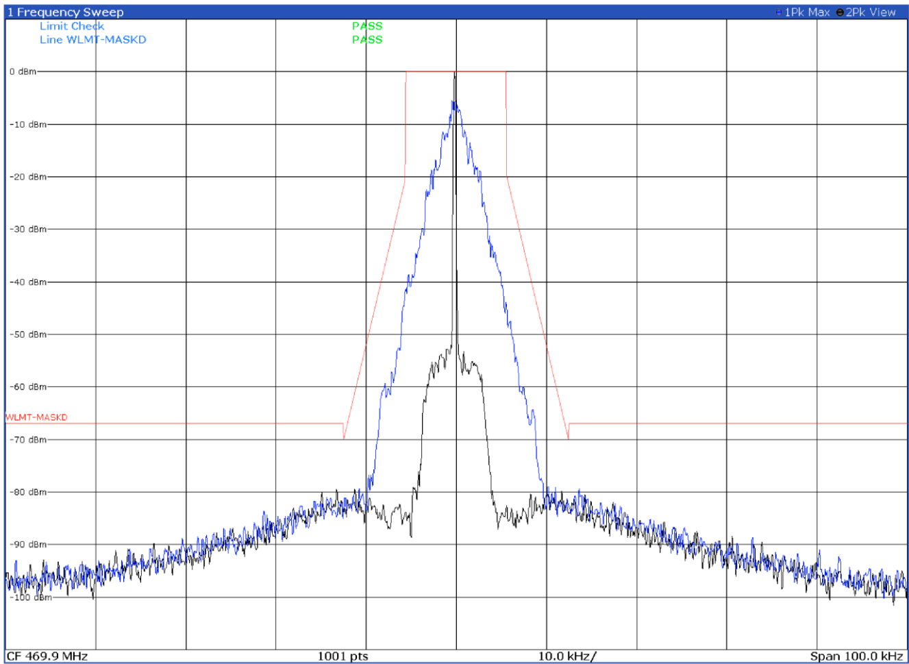
Emission mask D with modulation CST 4FSK at 469.9 MHz
