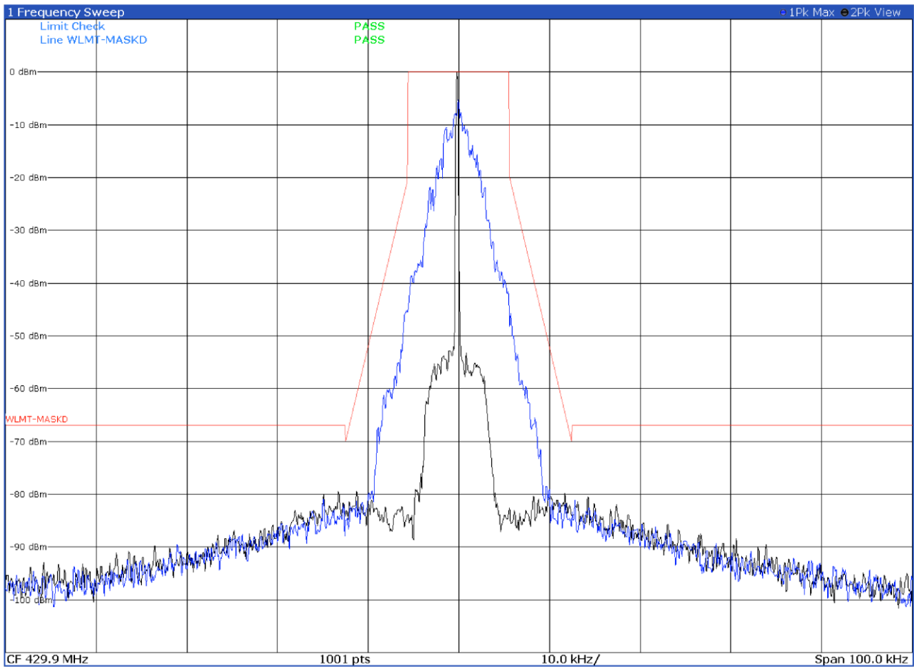
Emission mask D with modulation CST 4FSK at 429.9 MHz
