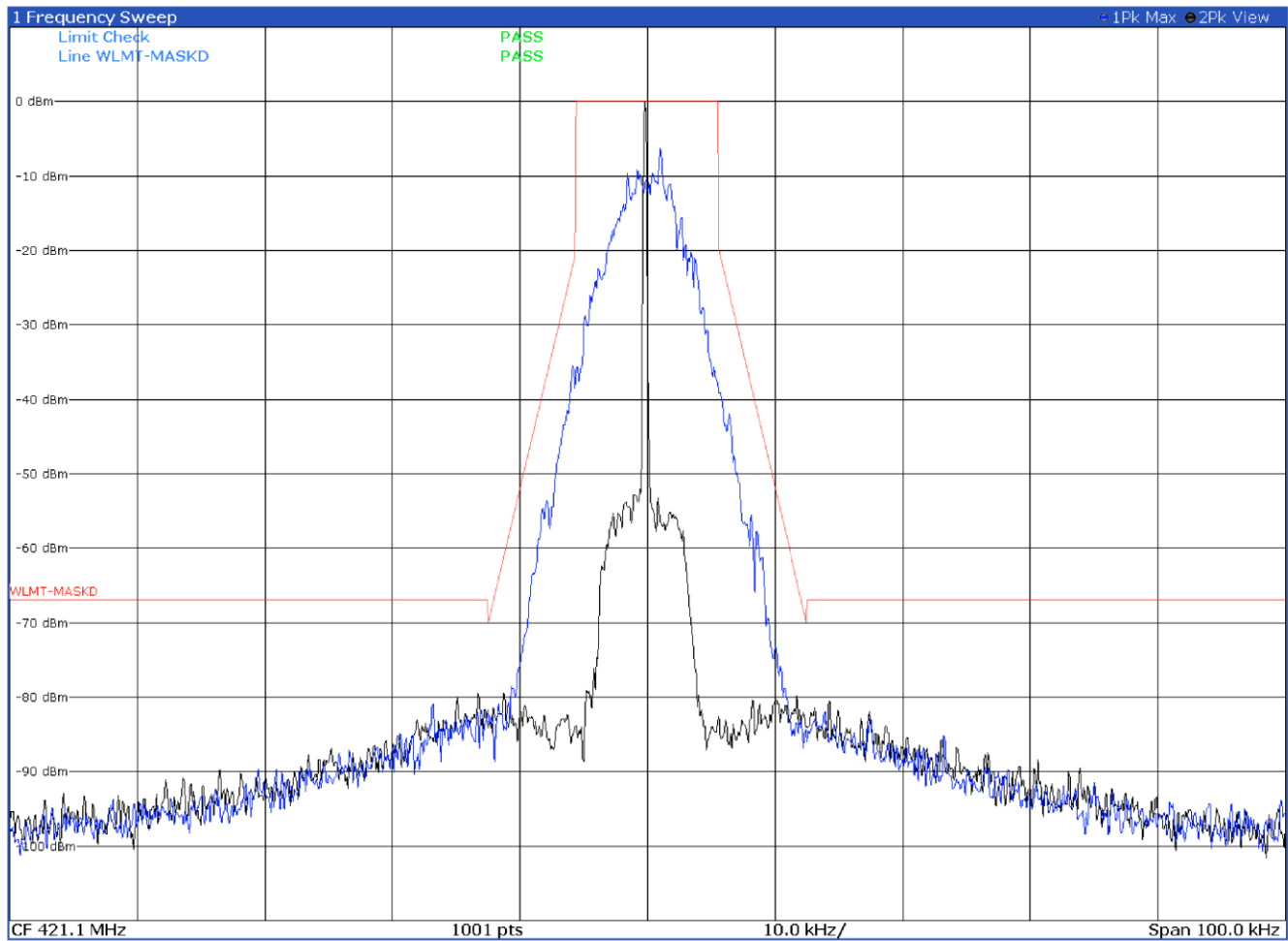
Emission mask D with modulation P25 C4FM at 421.1 MHz
