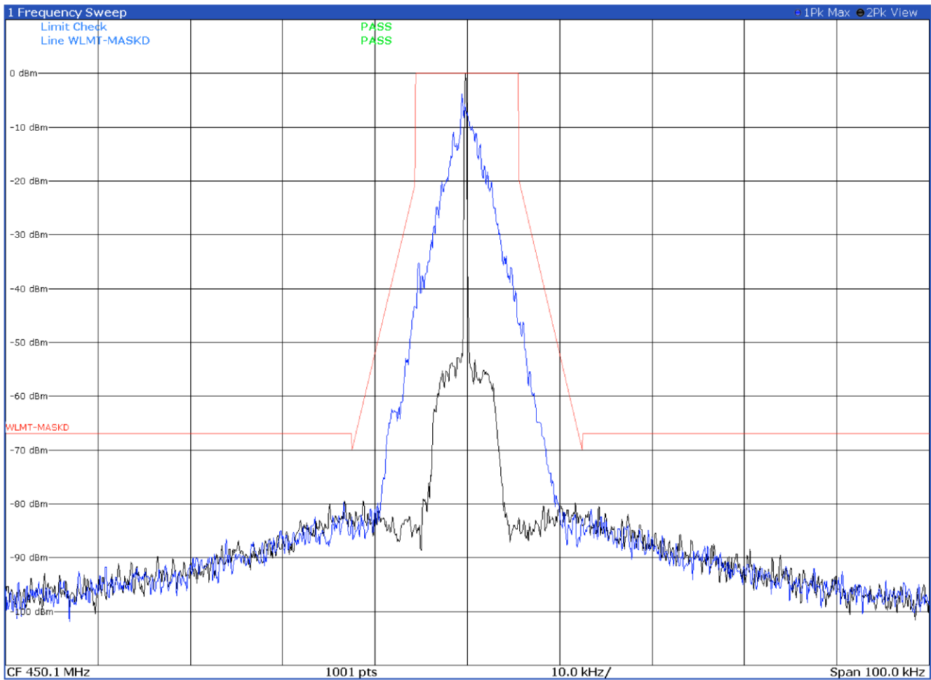
Emission mask D with modulation CST 4FSK at 450.1 MHz
