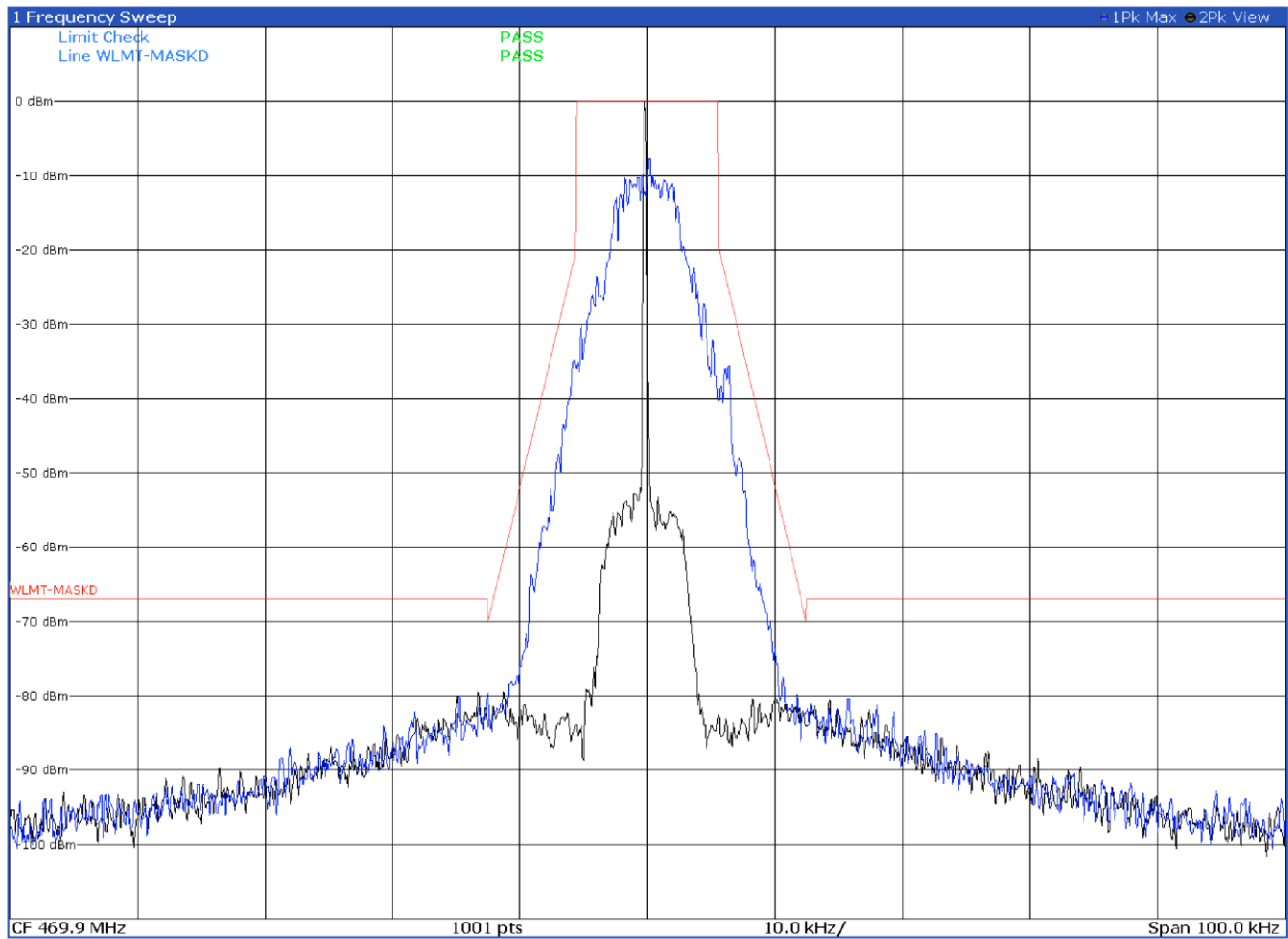
Emission mask D with modulation P25 C4FM at 469.9 MHz
