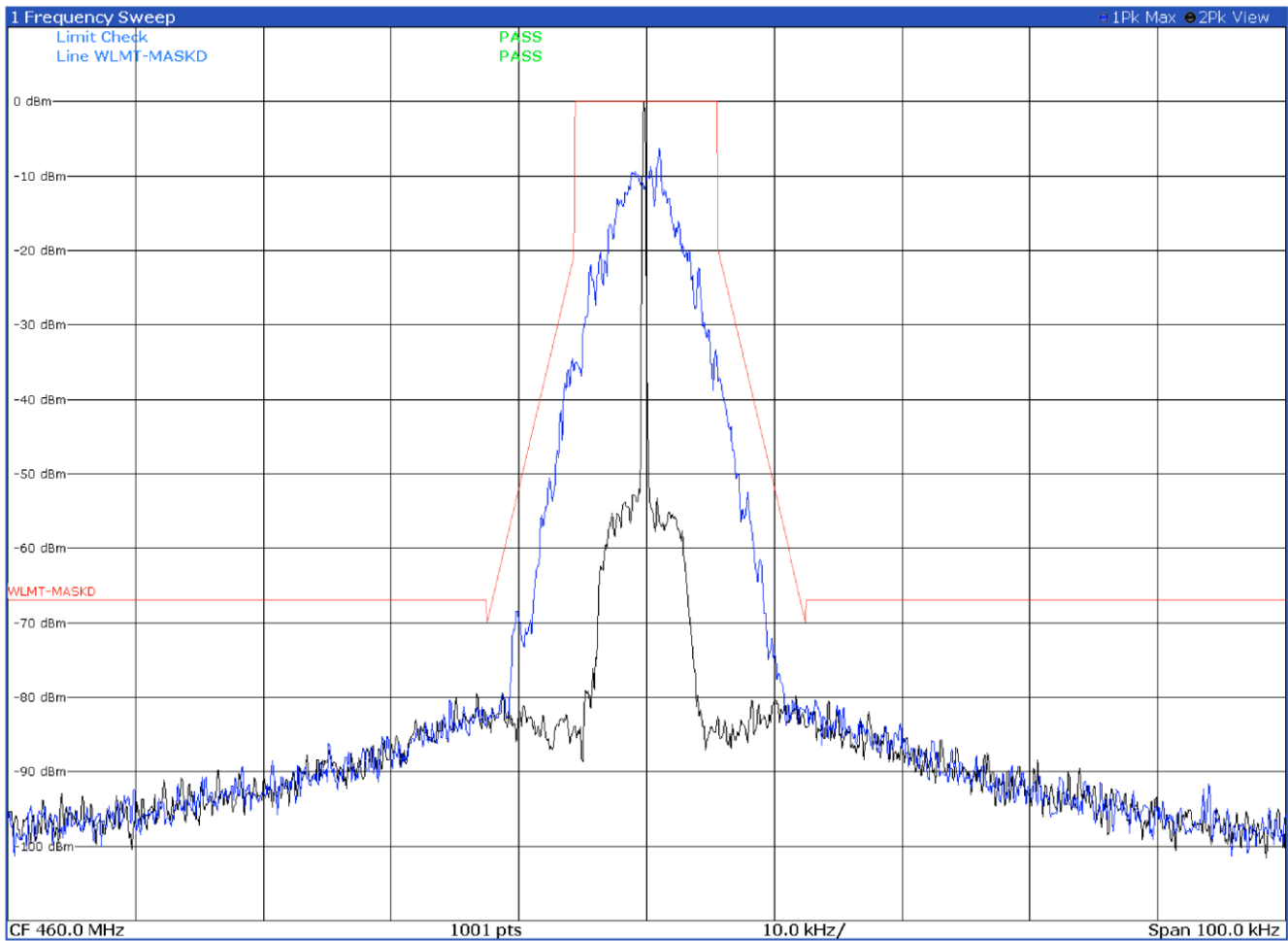
Emission mask D with modulation P25 C4FM at 460.0 MHz
