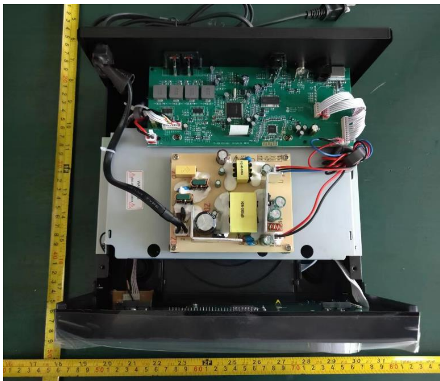
Internal photos M/N: XL-B530(BR)
