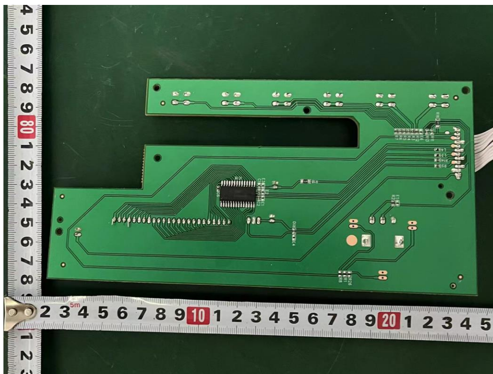
Internal photos M/N: XL-B530(BK)
