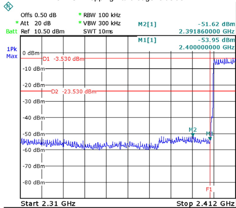
8DPSK Hopping Band edge-left side
