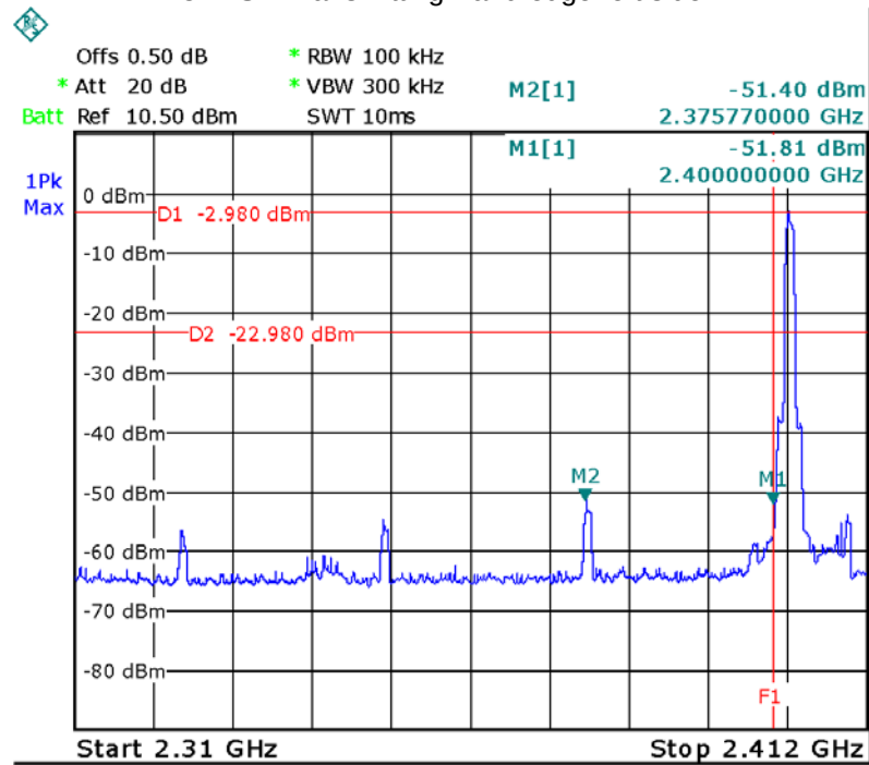
8DPSK Transmitting Band edge-left side
