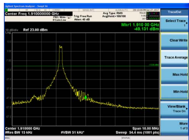
LTE Band 2 3MHz QPSK 100%RB CH-High
