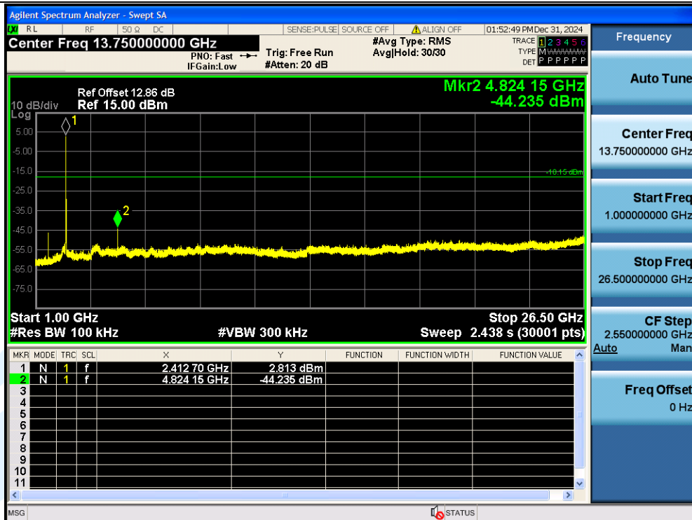
11B-Ant1-2412-1000~26500-PASS
