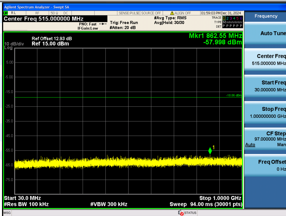
11B-Ant1-2462-30~1000-PASS
