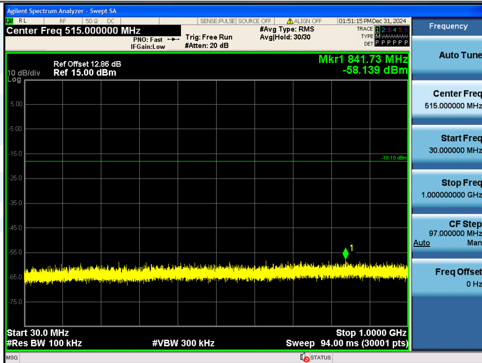
11B-Ant1-2412-30~1000-PASS
