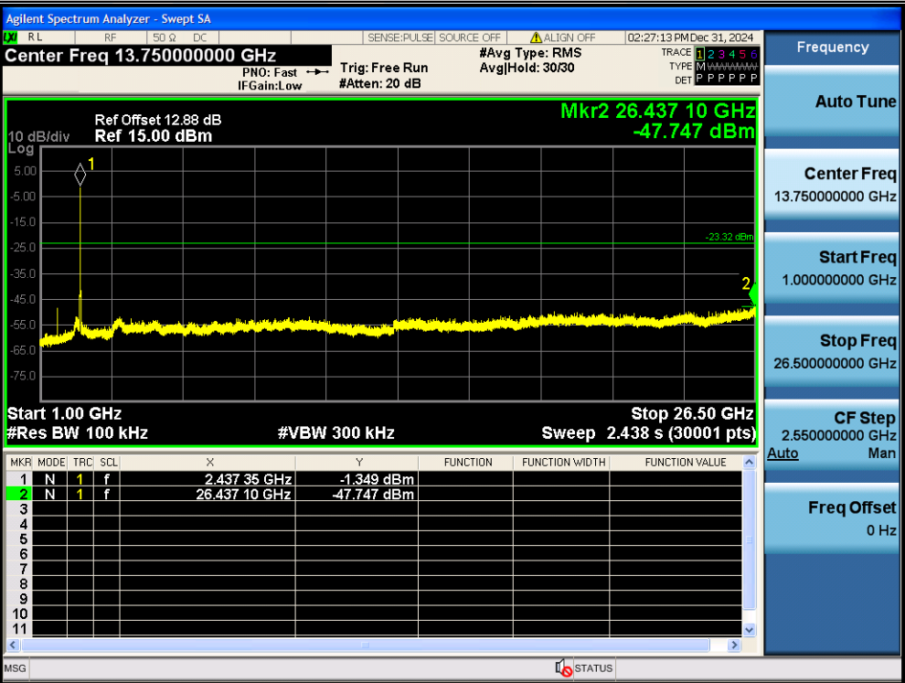
11N20SISO-Ant1-2437-1000~26500-PASS
