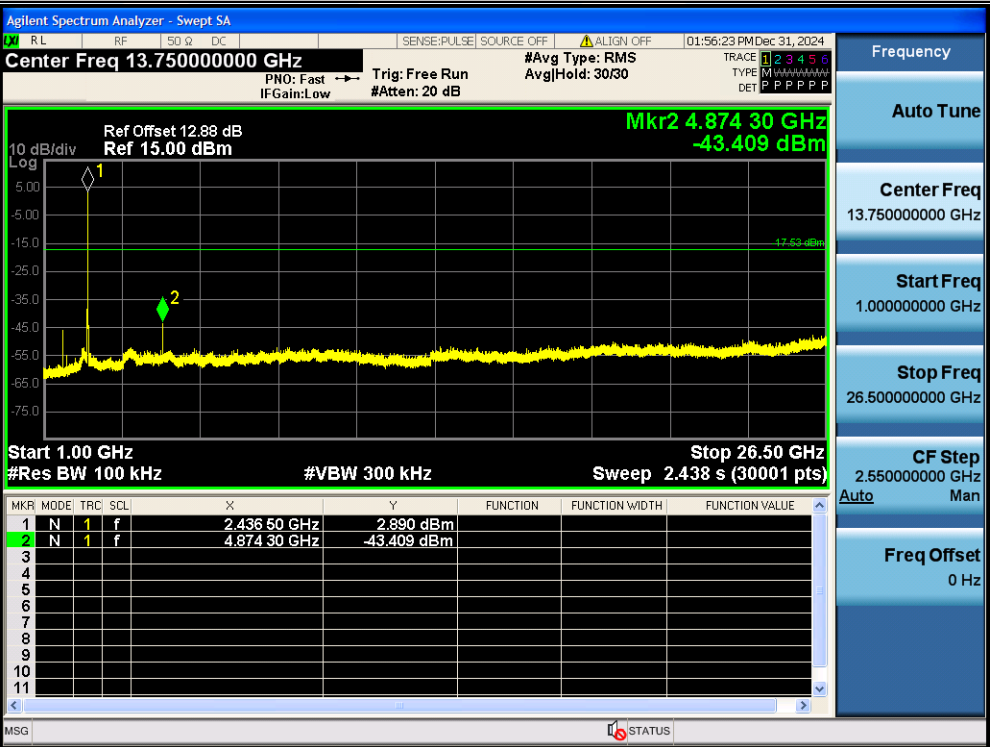
11B-Ant1-2437-1000~26500-PASS
