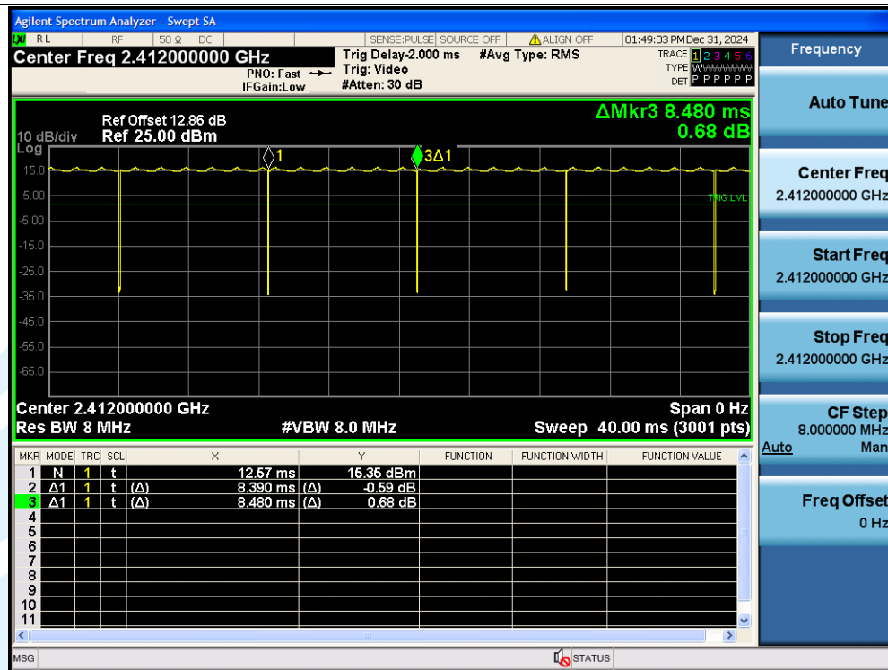
NTNV-11B-Ant1-2412
