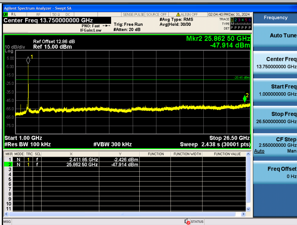
11G-Ant1-2412-1000~26500-PASS
