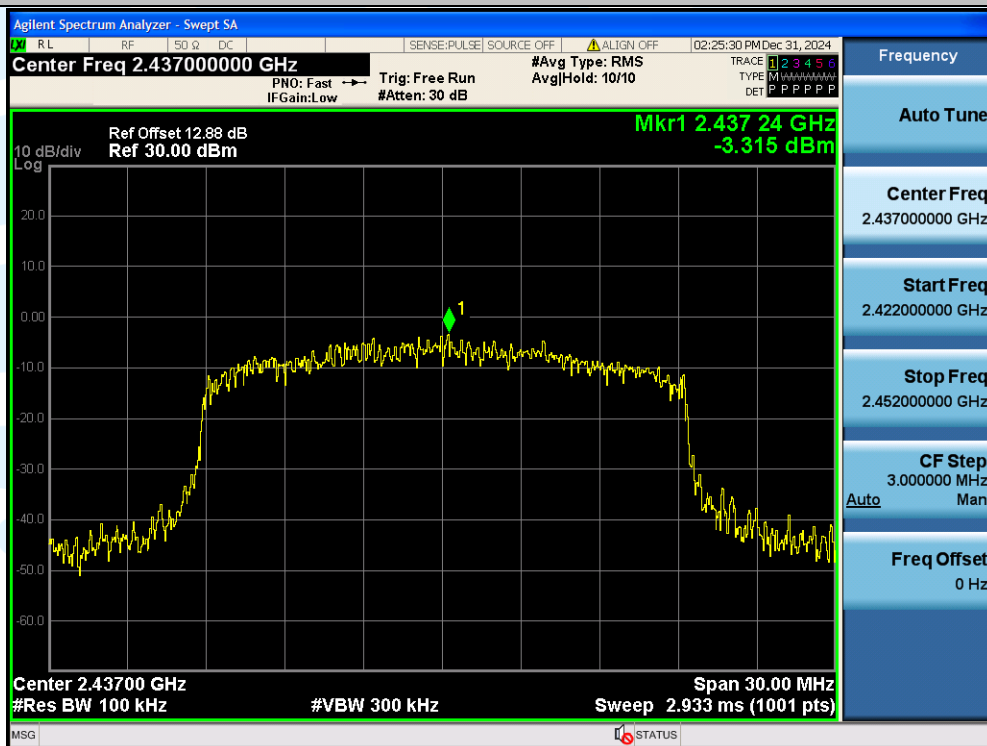
11N20SISO-Ant1-2437-0~Reference-PASS
