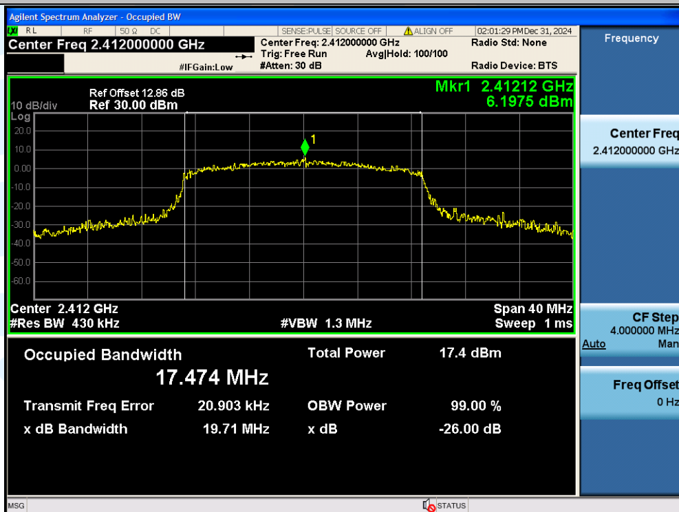
11G-Ant1-2412
