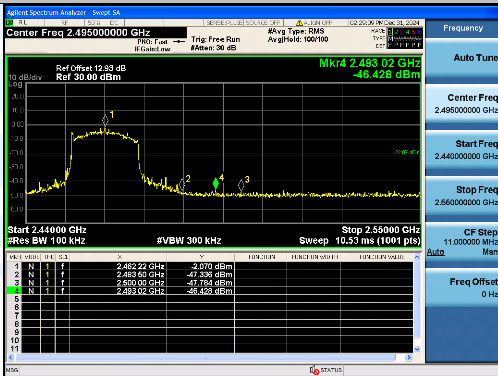
11N20SISO-Ant1-2462-PASS
