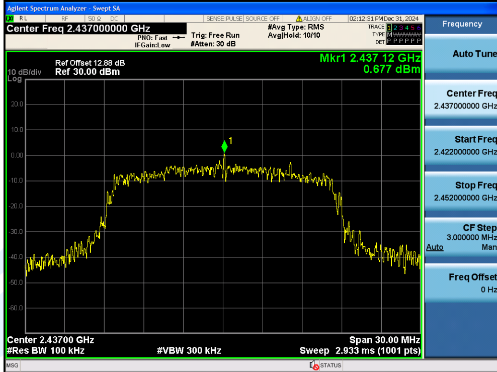
11G-Ant1-2437-0~Reference-PASS
