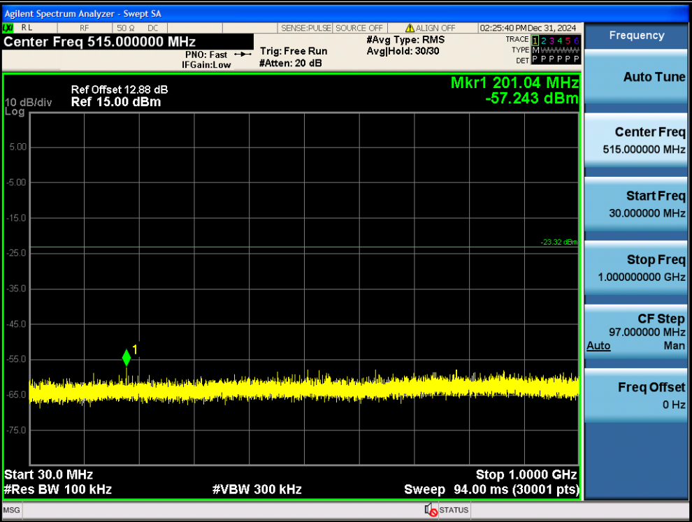
11N20SISO-Ant1-2437-30~1000-PASS
