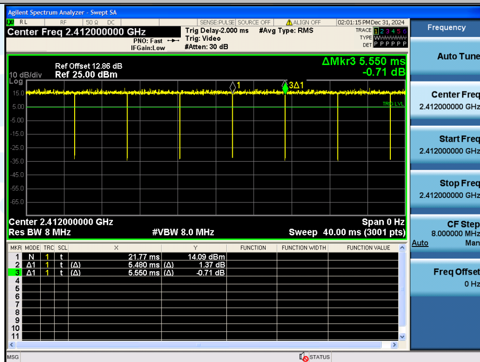
NTNV-11G-Ant1-2412
