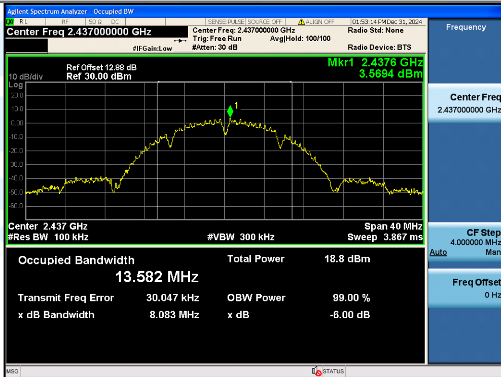
11B-Ant1-2437-PASS
