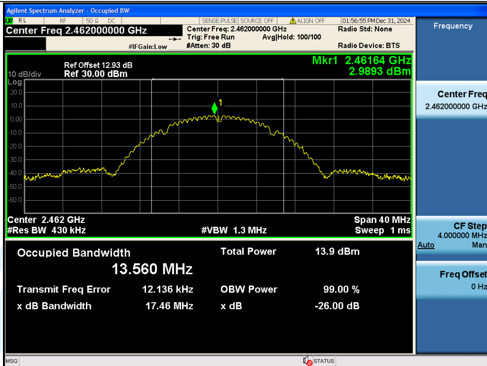
11B-Ant1-2462
