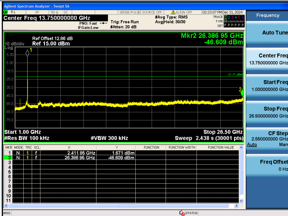
11N20SISO-Ant1-2412-1000~26500-PASS
