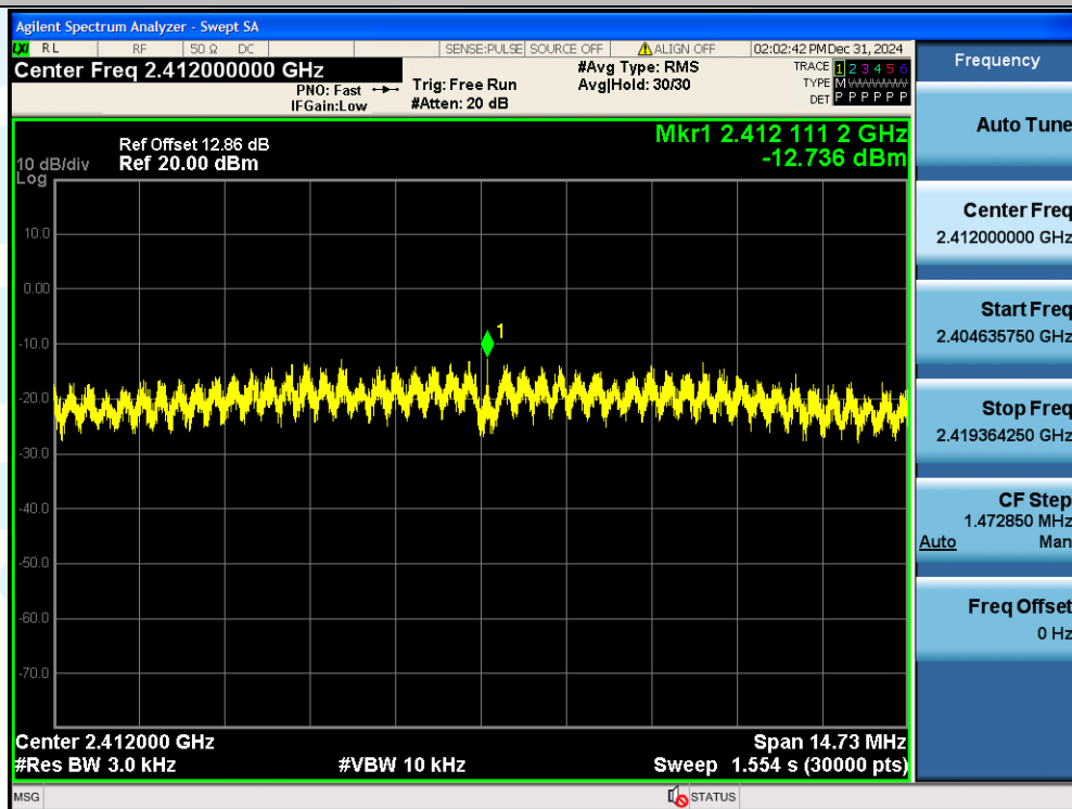
11G-Ant1-2412-PASS
