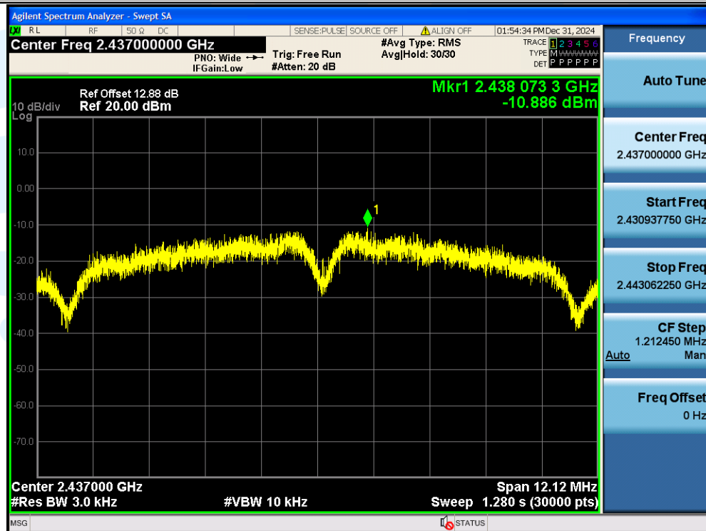
11B-Ant1-2437-PASS
