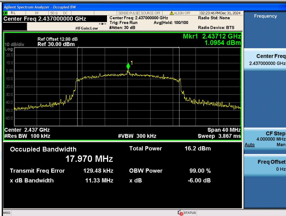
11N20SISO-Ant1-2437-PASS
