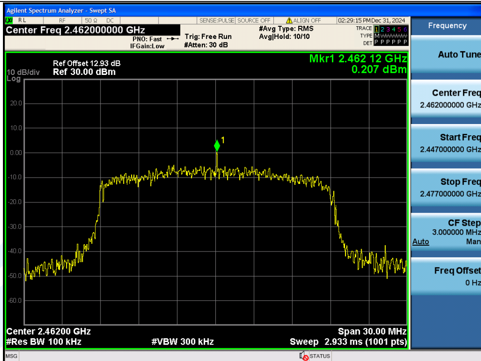
11N20SISO-Ant1-2462-0~Reference-PASS
