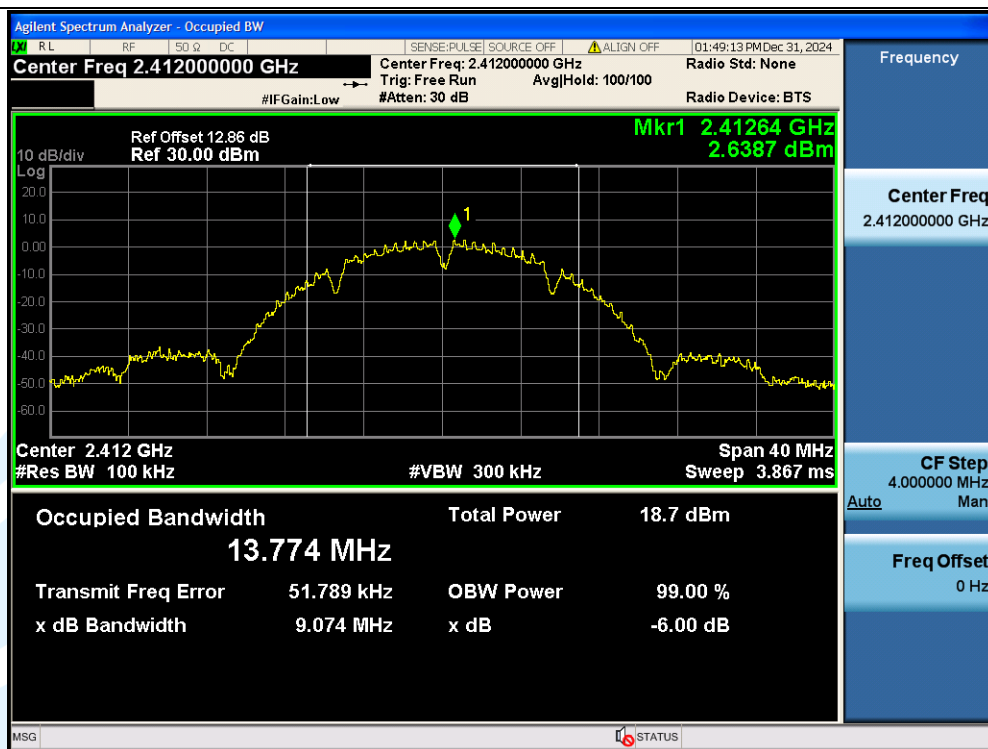
11B-Ant1-2412-PASS
