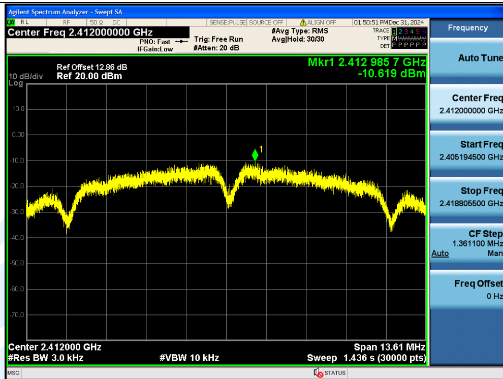
11B-Ant1-2412-PASS
