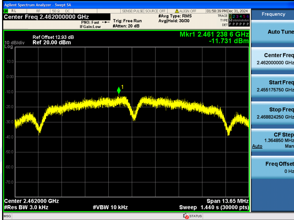
11B-Ant1-2462-PASS
