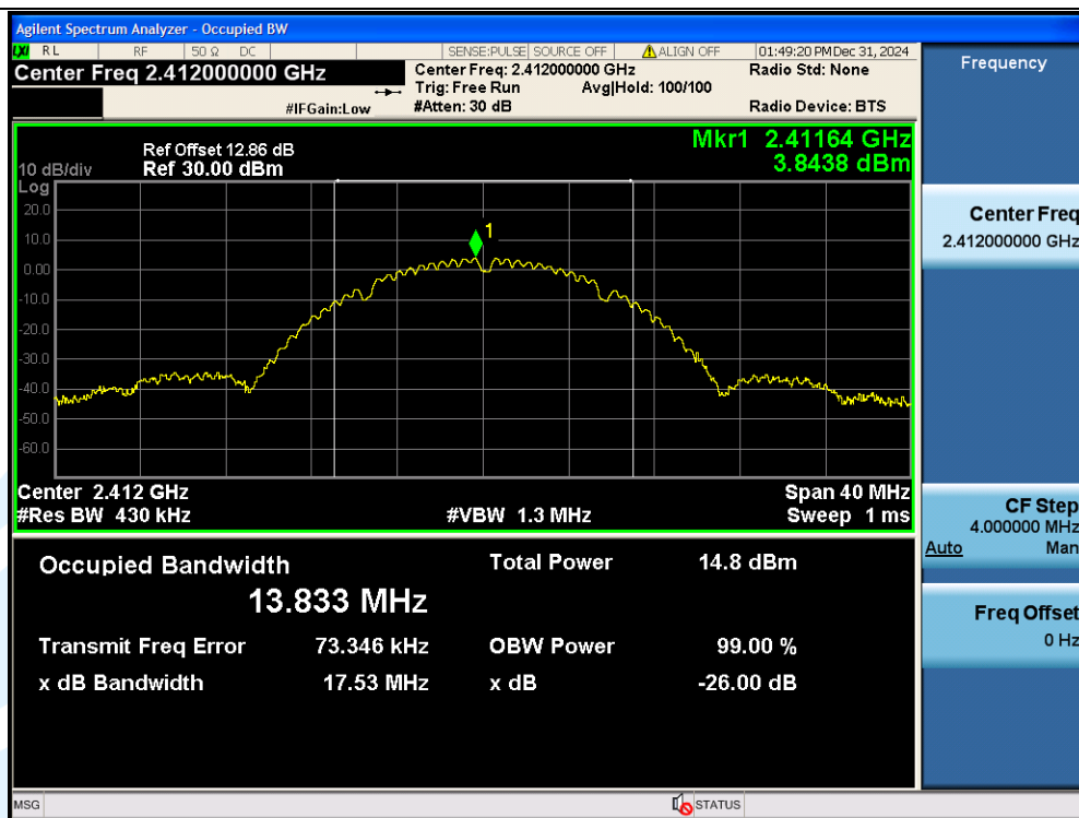
11B-Ant1-2412
