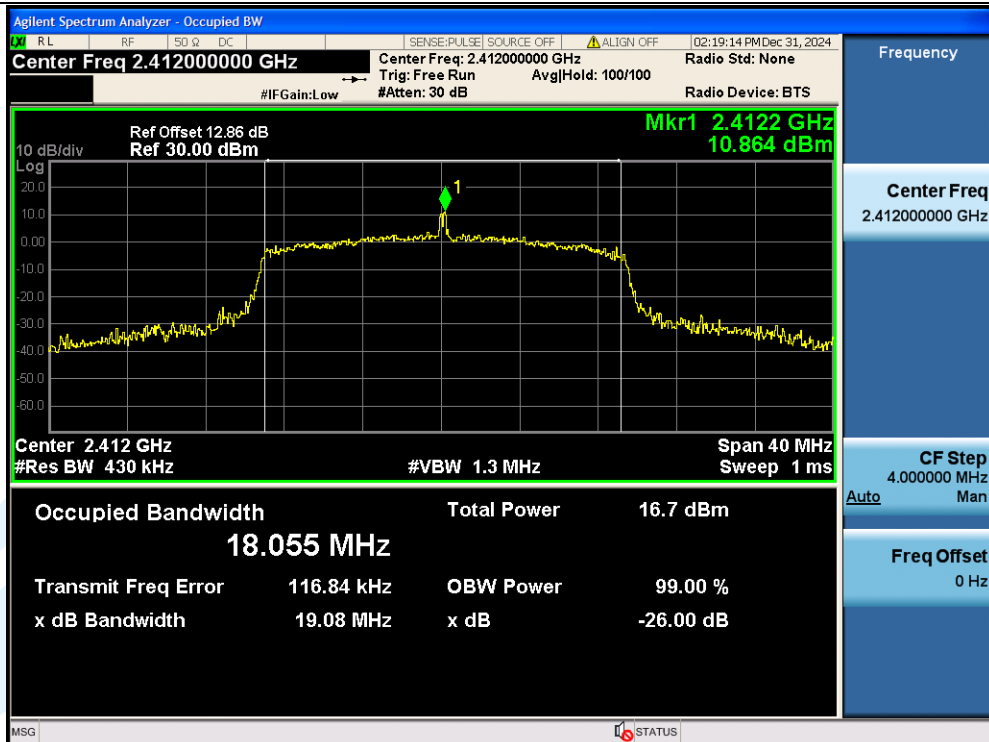
11N20SISO-Ant1-2412
