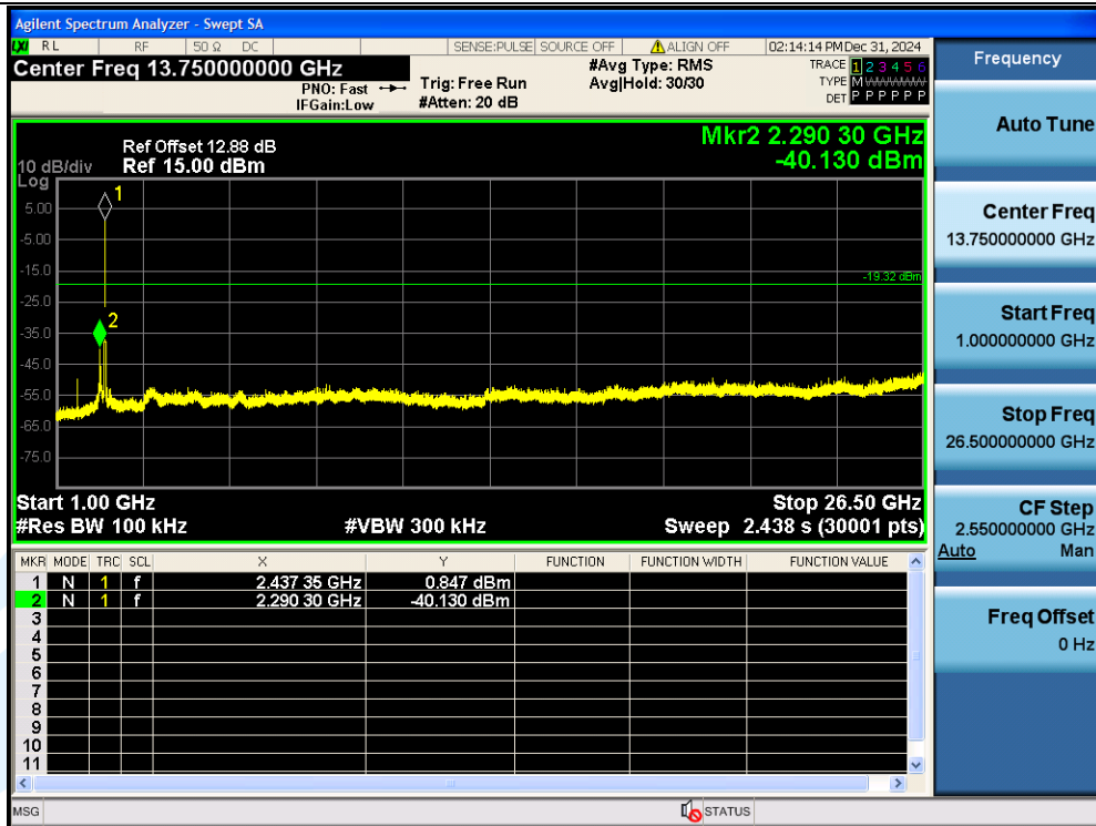
11G-Ant1-2437-1000~26500-PASS
