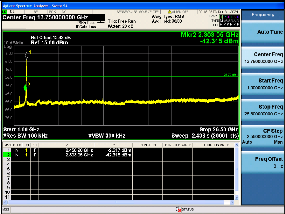
11G-Ant1-2462-1000~26500-PASS
