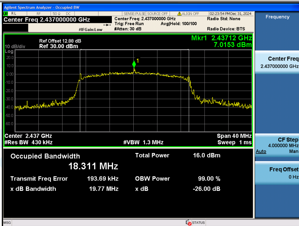
11N20SISO-Ant1-2437
